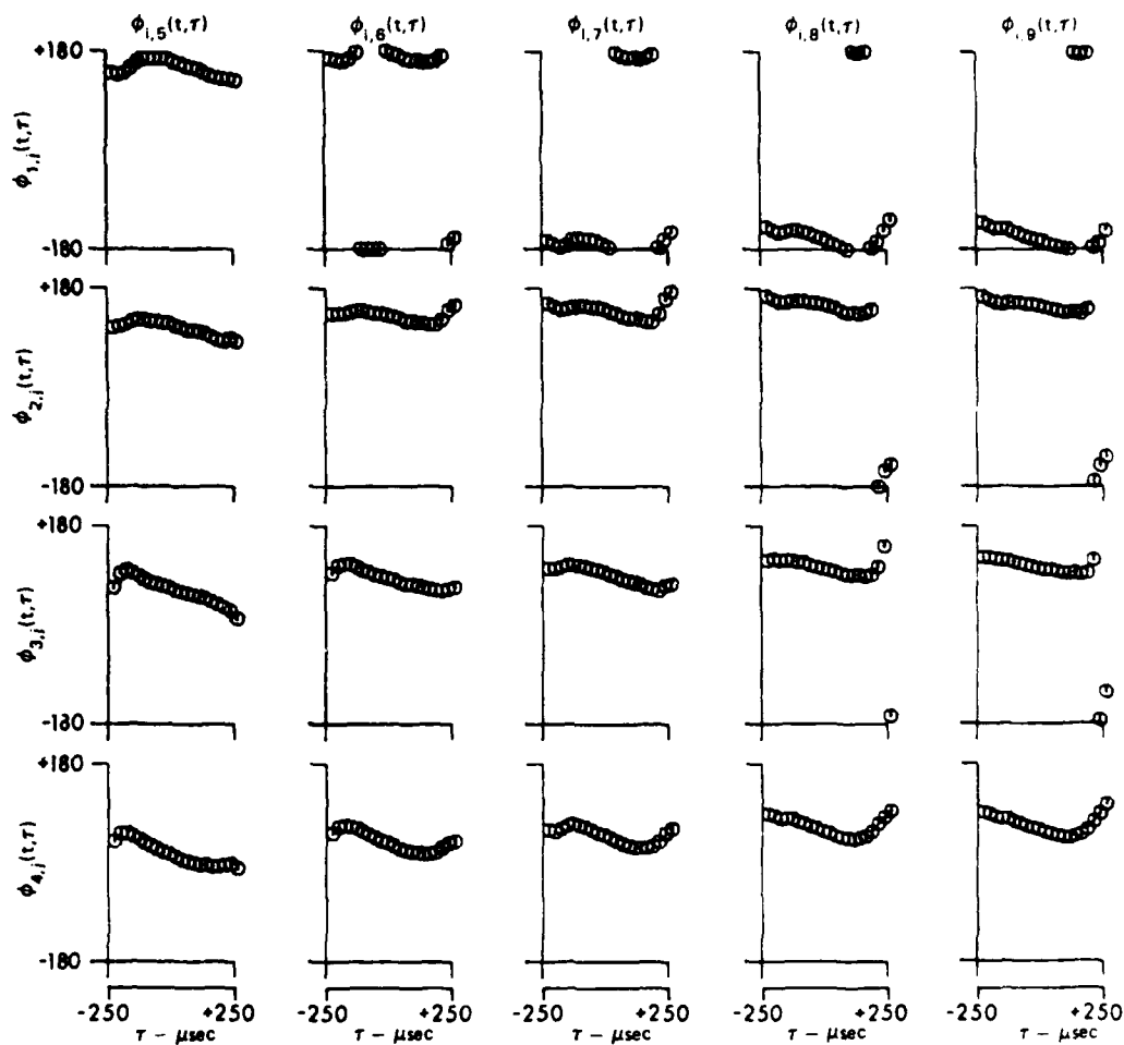
FIGURE V-54 PHASES OF THE SAMPLE ESTIMATE OF THE NORMALIZED COVARIANCE OF THE VERTICAL ARRAY AS A FUNCTION OF \tau FOR t = 75.25 msec
