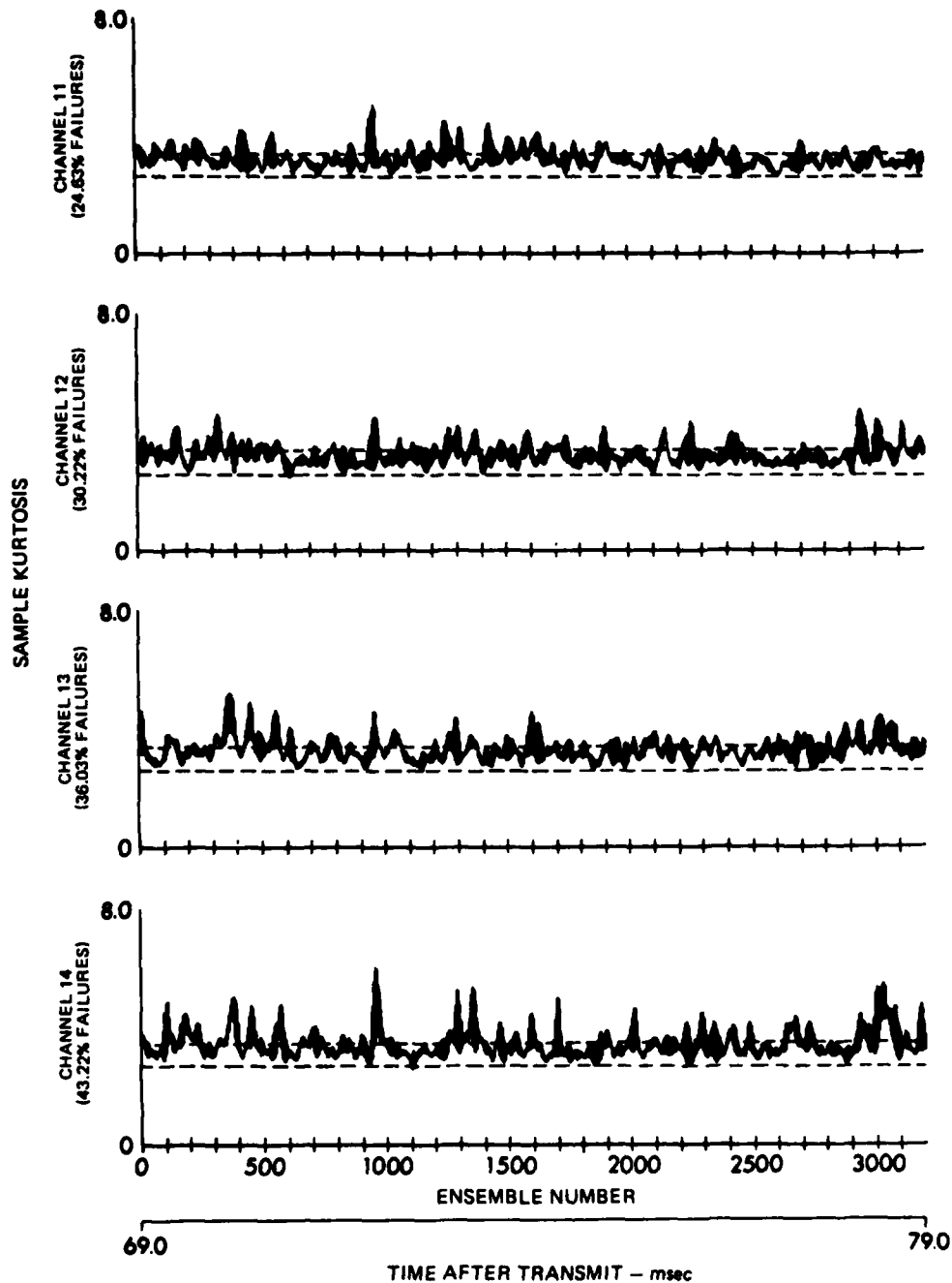
FIGURE IV-23 PEARSON'S TEST OF KURTOSIS FOR NORMALITY, CHANNELS 11-14
