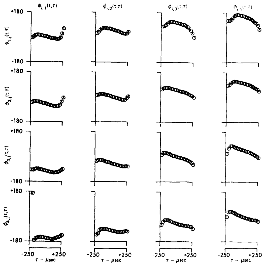
FIGURE V-53 PHASES OF THE SAMPLE ESTIMATE OF THE NORMALIZED COVARIANCE OF THE VERTICAL ARRAY AS A FUNCTION OF \tau FOR t = 75.25 msec
