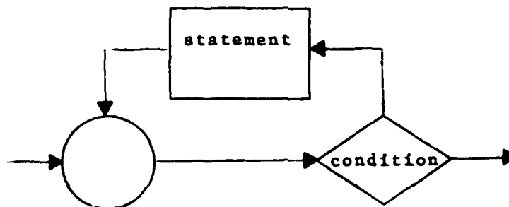
DOWHILE
