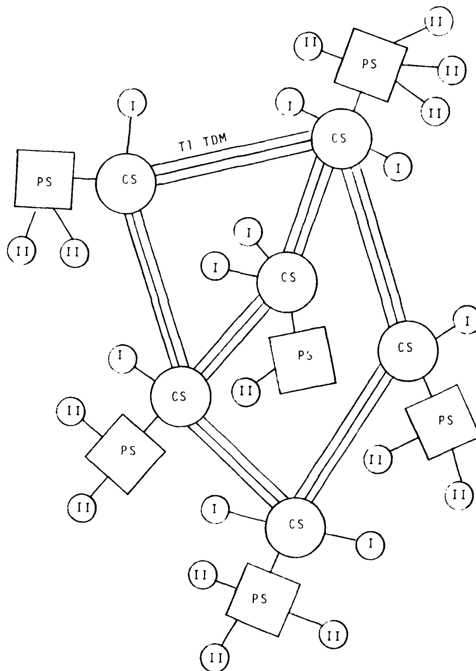
Fig. 5. Network configuration
