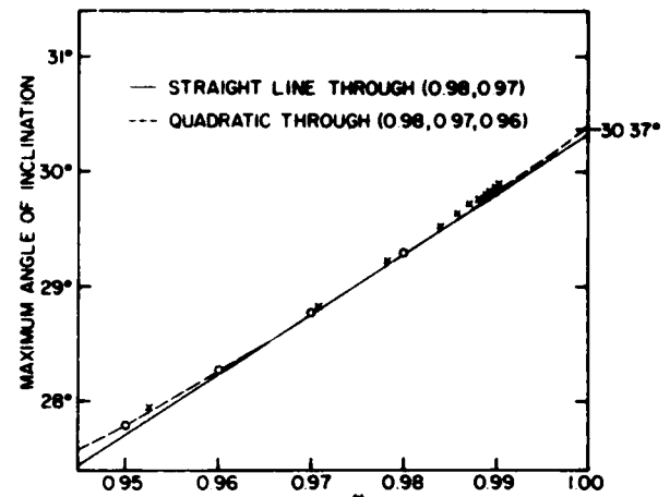
Fig. 5 — The maximum surface angle of inclination for very high solitary waves. The open circles and error bar are from these calculations. The x's are from Sasaki and Murakami (1973). The value of 30.37^\circ is derived by Longuet-Higgins and Fox (1977). The solid curve is a straight line matching the open circles at \omega = 0.98 and \omega = 0.97 . The dashed curve is a quadratic fit to the open circles at \omega = 0.98, 0.97 , and 0.96 .
