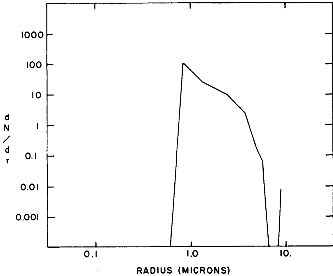
Fig. 21 — A plot of the difference between the dN/dr data obtained with the PMS aerosol size spectrometer during the fog event of 28 July 1980 and the ambient values taken shortly after the event. The instrument was located on the NRL micrometeorological tower on SNI for these measurements.
