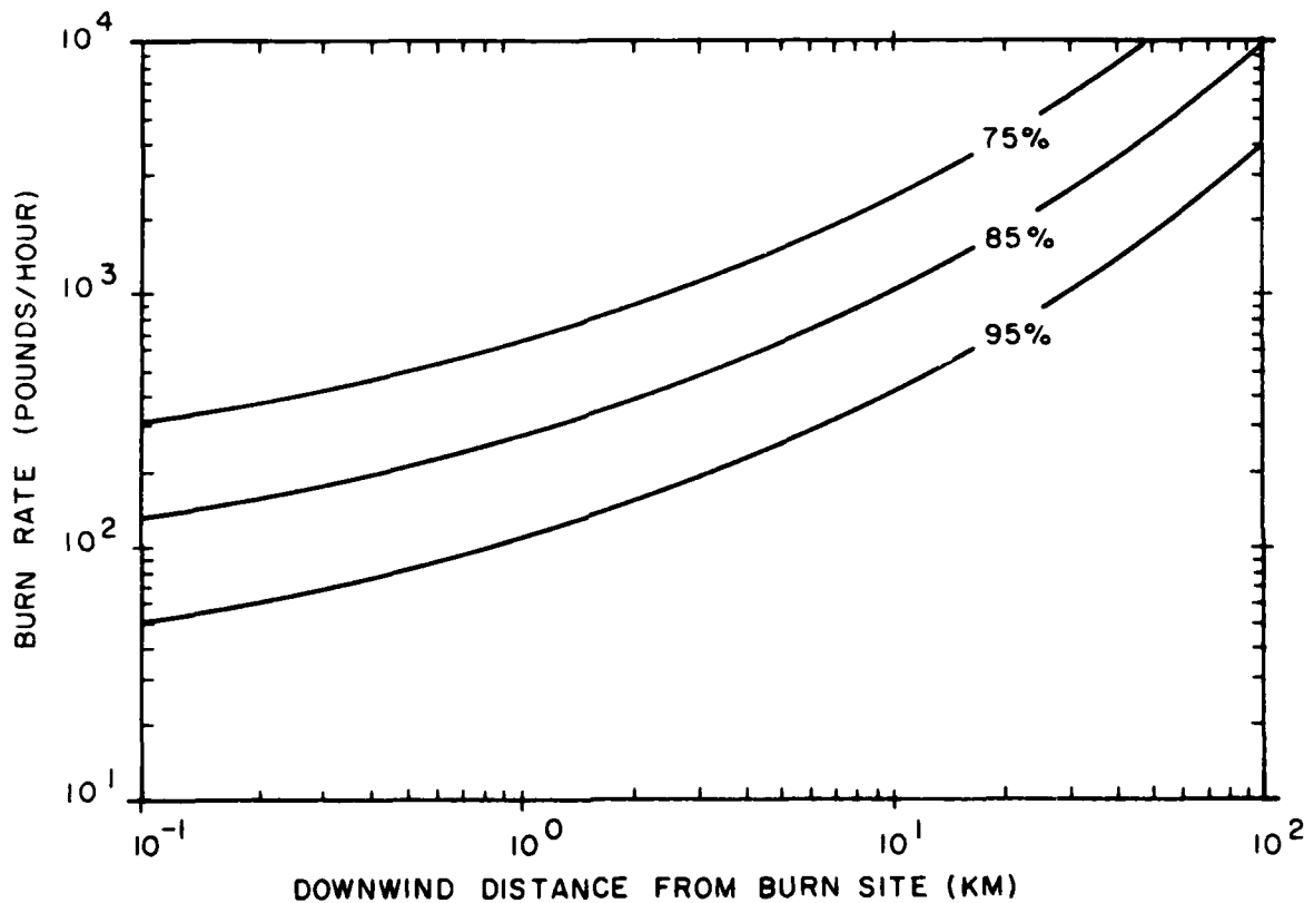
Fig. 7 - The effect of variations in the ambient relative humidity and its effect in the growth of the "Salty Dog" aerosol and the required burning rate necessary to achieve a reduction in the visibility from 32 km to 12.8 km in the crosswind transmissometer path plotted as a function of distance from the source to the sensor. The calculation assumes a wind speed of 7 m/s, a 500 meter inversion base height, neutral stability, an effective emission height of 10 m and a sampling height of 15.2 m.
