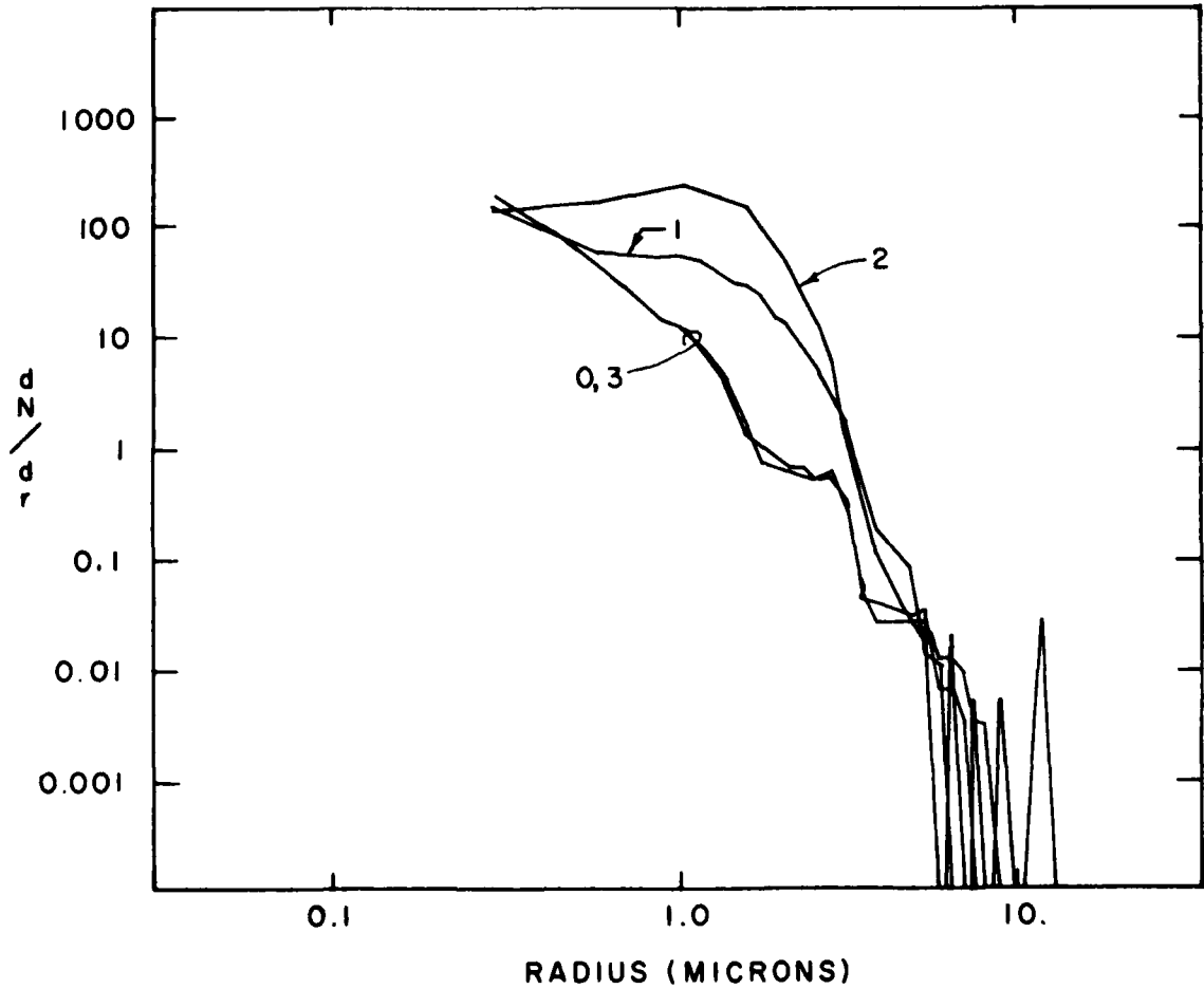
Fig. 23 - Plot of the aircraft measured dN/dr size distribution before, during and after the artificial fog event of 30 July 1980
