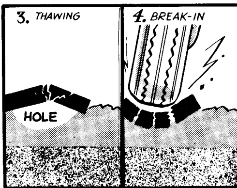
Factors leading to pothole failure by fatigue
