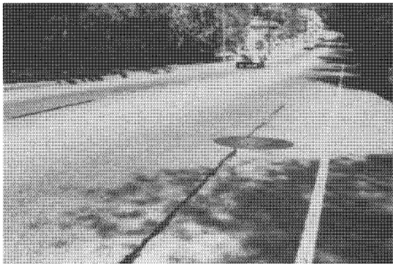
Sealing cracks and repairing pavement at manholes prevents potholes
