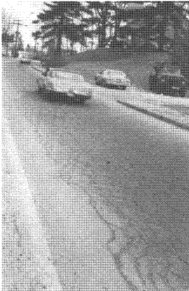
Thick pavements may crack but are difficult to pothole because of their mass
