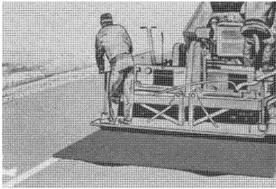
Rutted roadways should be leveled and compacted before overlaying to prevent delamination
