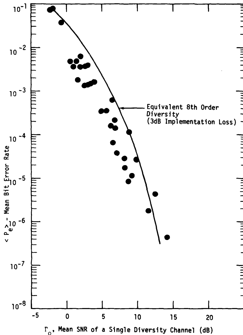
Figure 23. MDTs Over-the-Air Performance Youngstown - Verona (168 Miles) C - Band, Quad Diversity 6dBNF, AN/TRC-132A 12.6 Mb/s
