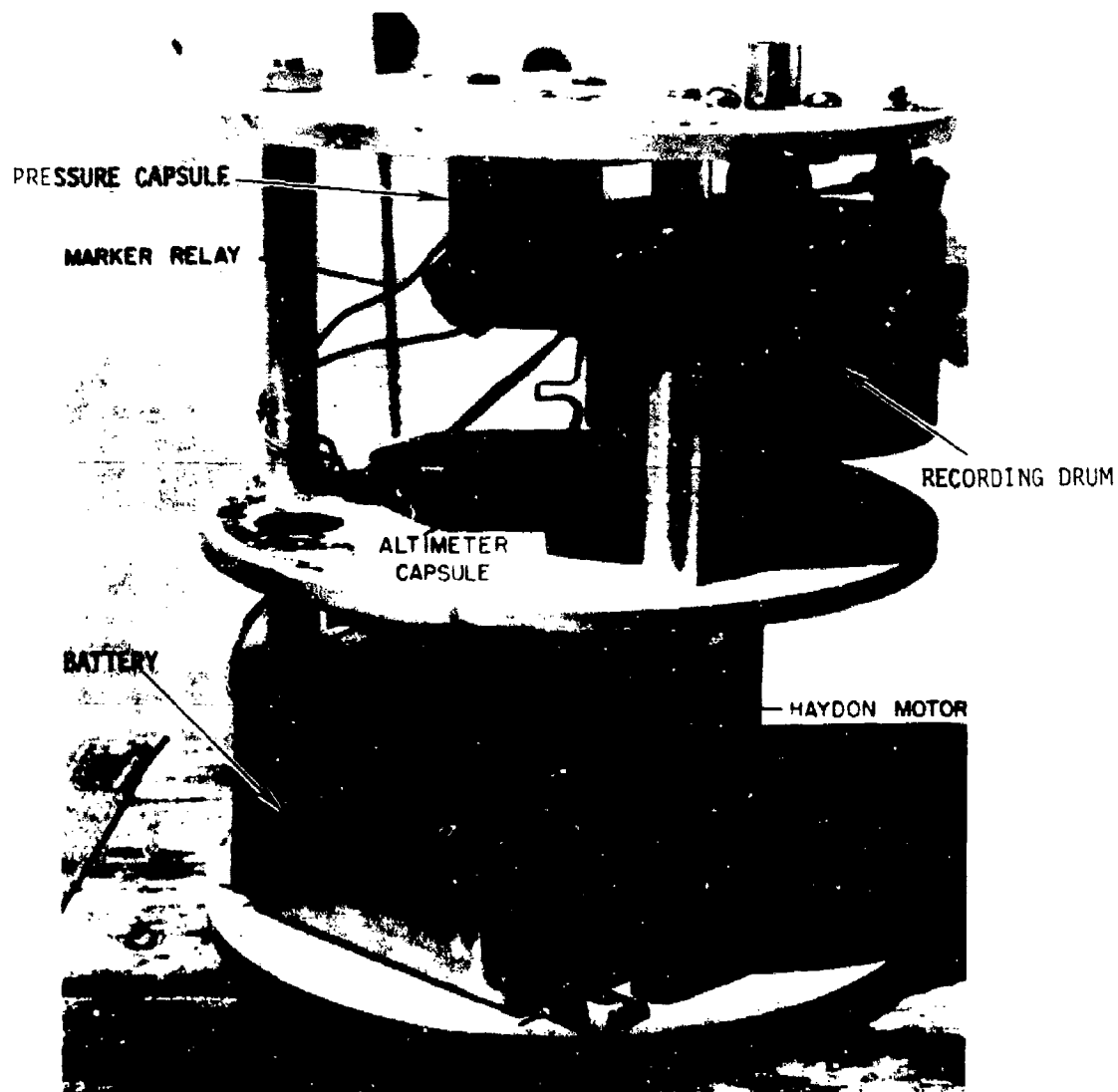
Figure 5-4. PRESSURE AND TIMING SYSTEM.
