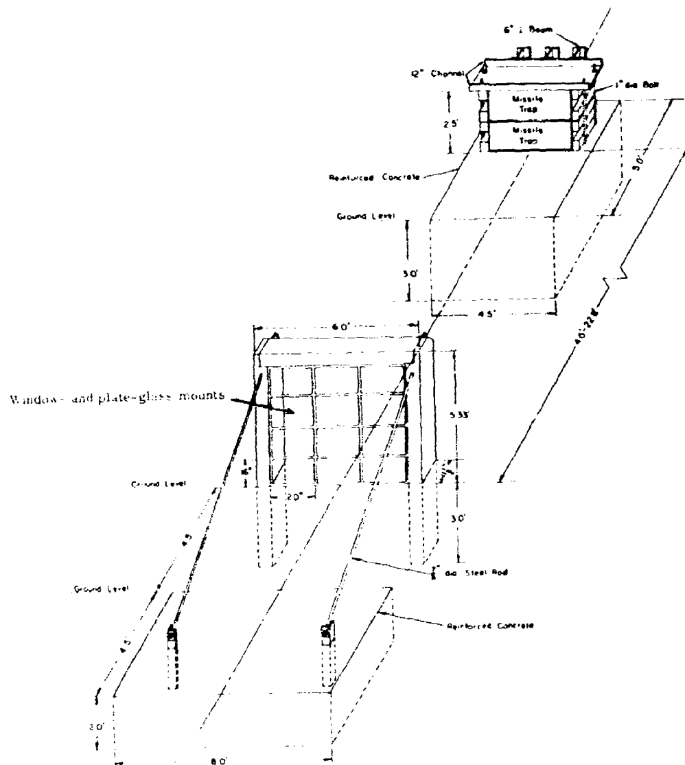
Figure 5-18. MISSILE-COLLECTING TRAP SYSTEM.
