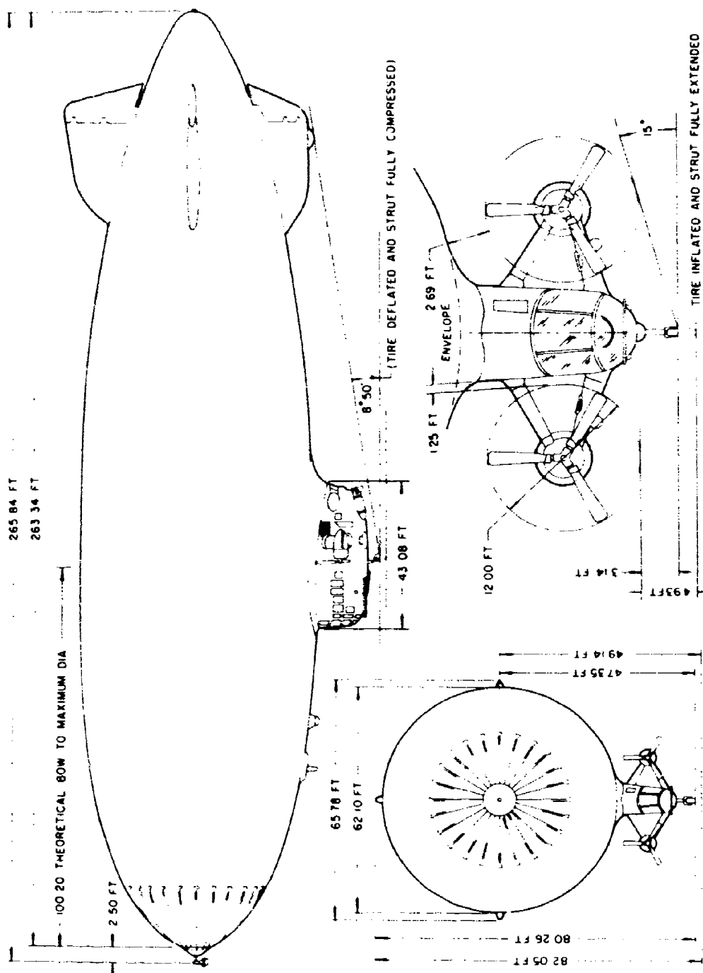
Figure 5-19. PRINCIPAL DIMENSIONS OF MODEL ZSG-3 AIRSHIP.
