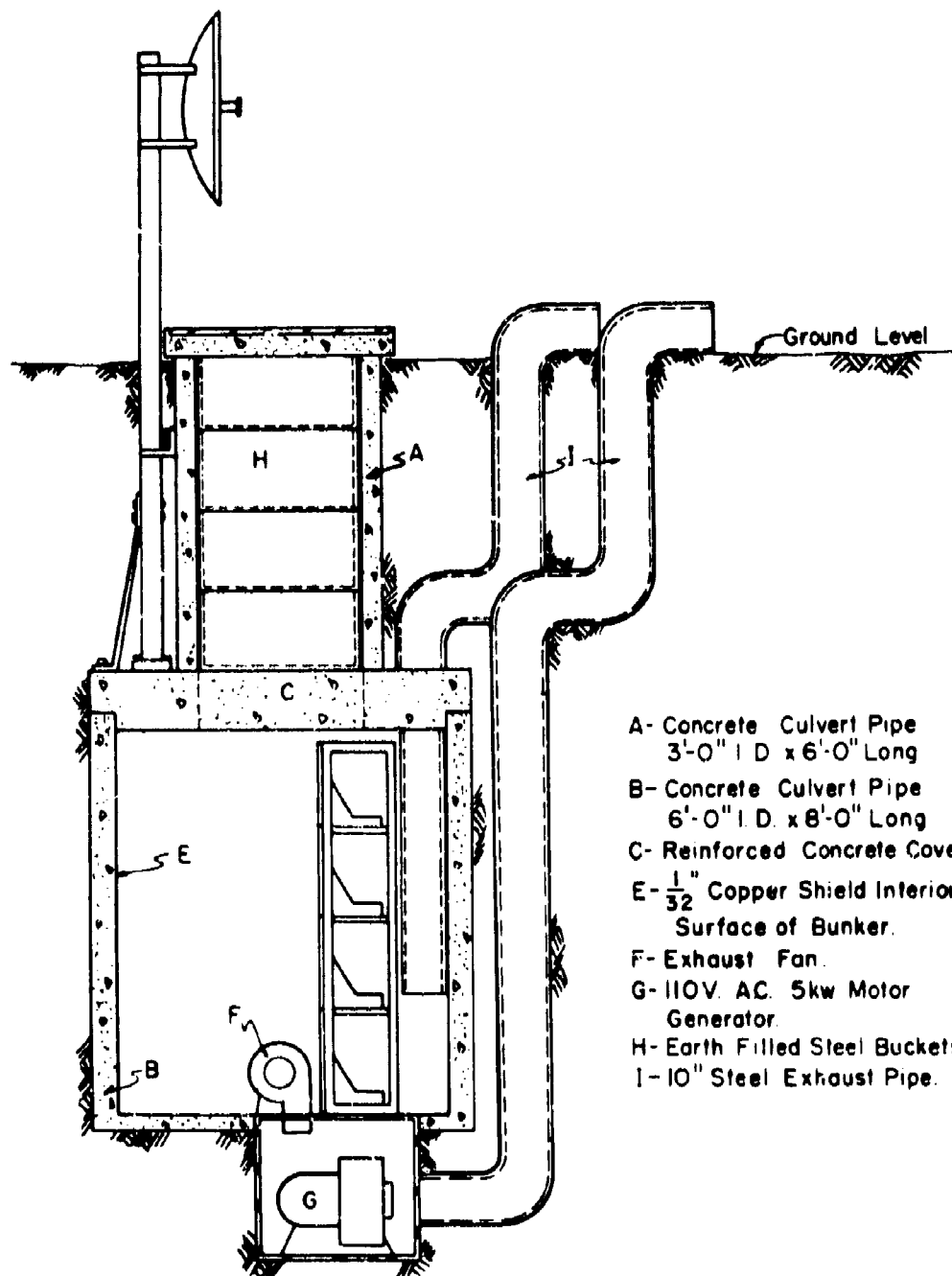
Figure 5-13. TYPICAL BUNKER INSTALLATION.
