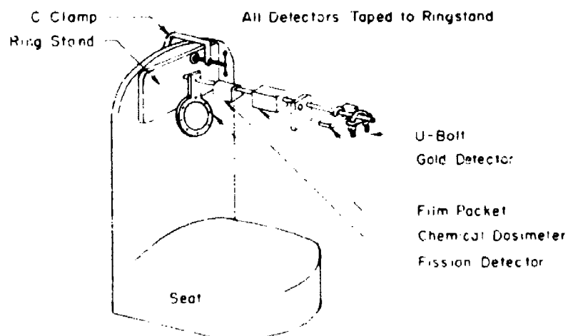
Figure 5-10. MOUNTING OF DETECTORS IN M-48 TANK.
