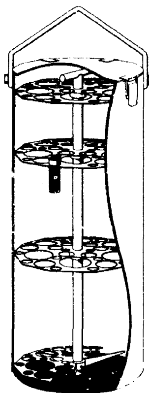
Figure 5-11. CROSS-SECTIONAL DIAGRAM OF ALUMINUM SAMPLE CONTAINER.
