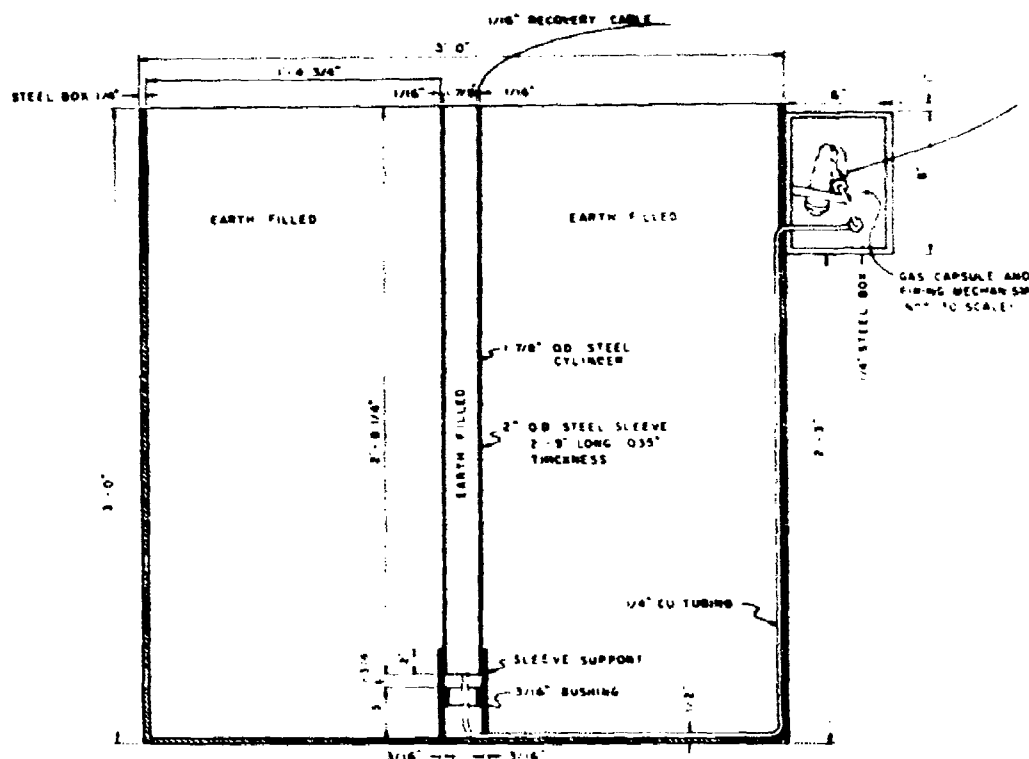
Figure 5-7. CROSS-SECTIONAL DIAGRAM OF AN EXPOSED SOIL SAMPLE.
