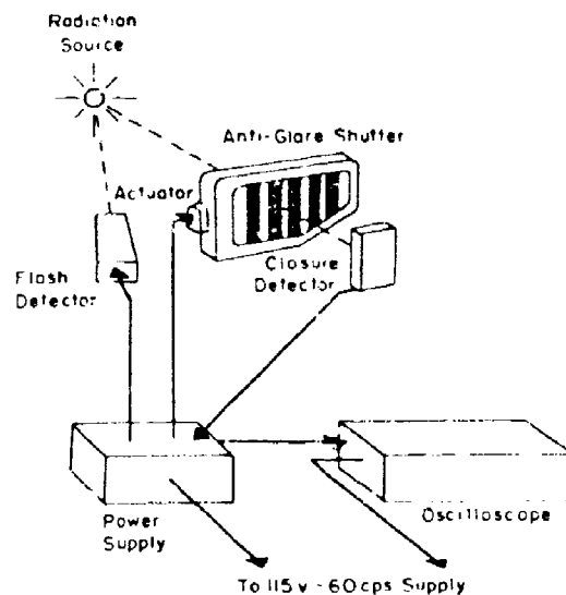
Figure 5-17. ANTI-GLARE SHUTTER SYSTEM.
