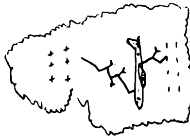
INTRA CLOUD RETURN STROKE
