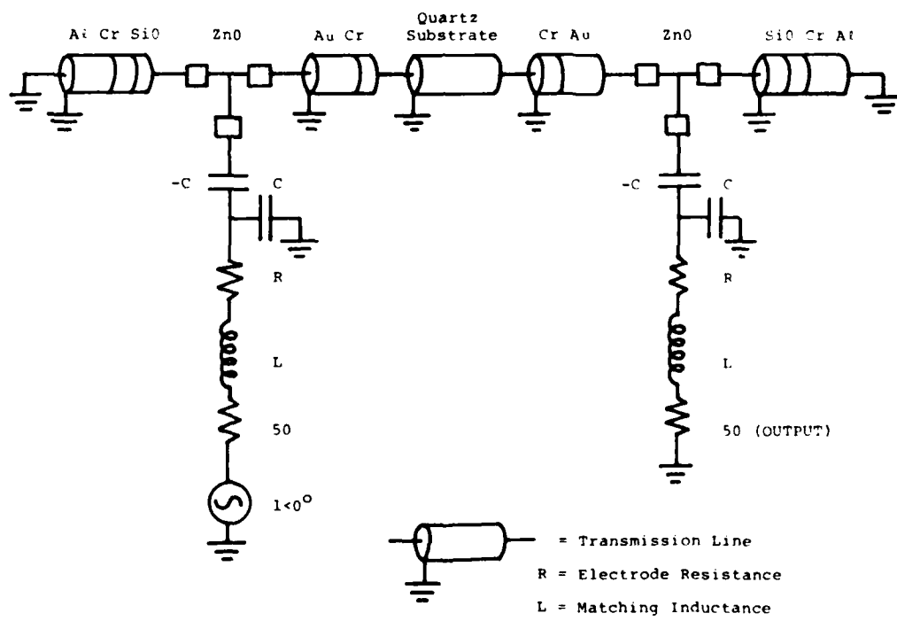
Figure 2. Transmission-line model
