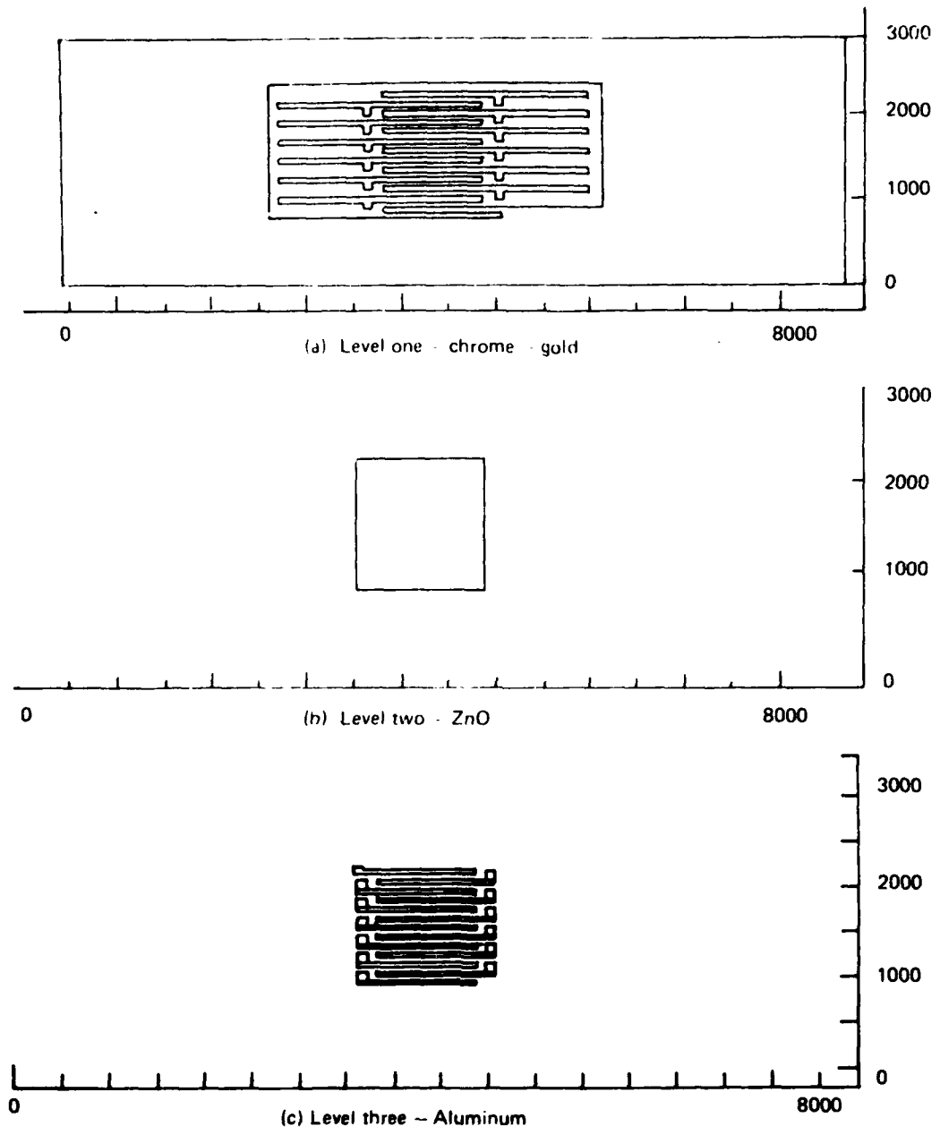
Figure 5. Initial mosaic transducer design (1 grid unit = 0.5 \mu\text{m} ).
