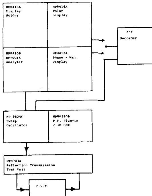
Figure 43. Block diagram of swept test setup.
