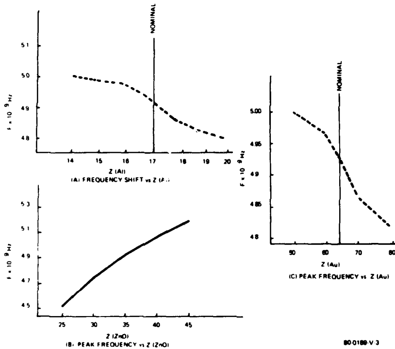
Figure 3. Variation in center frequency versus acoustical impedance ( Z ) of transducer constituent films.
