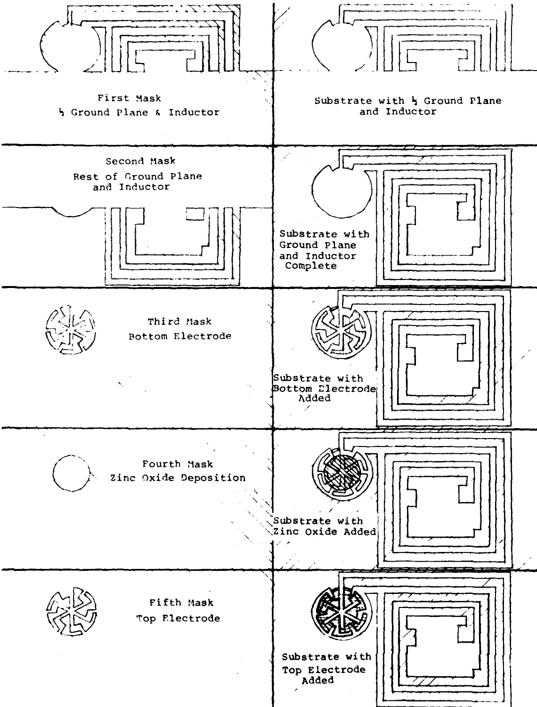
Figure 26. Exploded view of metal mask series.
