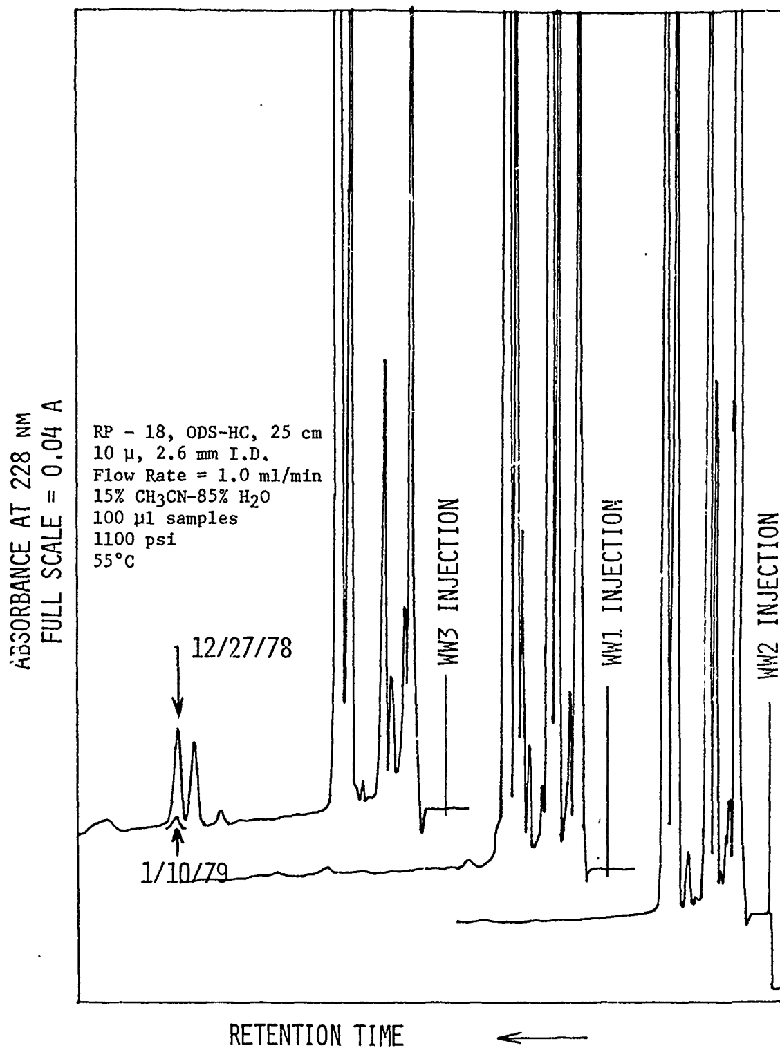
Figure 7. Liquid chromatograms of HSAAP wastewaters
