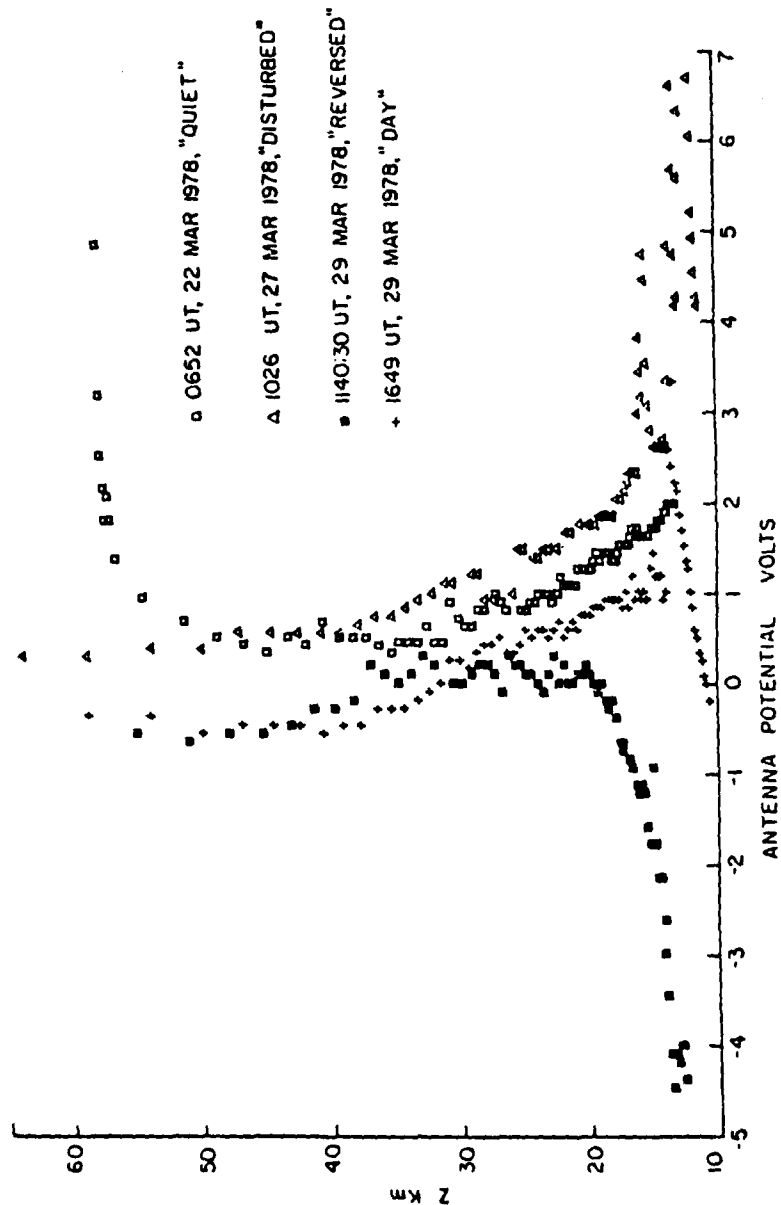
Figure 3: ~ DOWNWARD ELECTRIC FIELD (VOLTS/METER) DURING "AUFOROZONE II"
