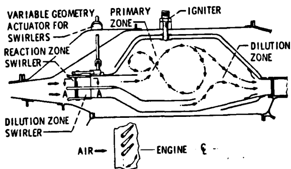
VIEW A-A (VARIABLE SWIRLER)
