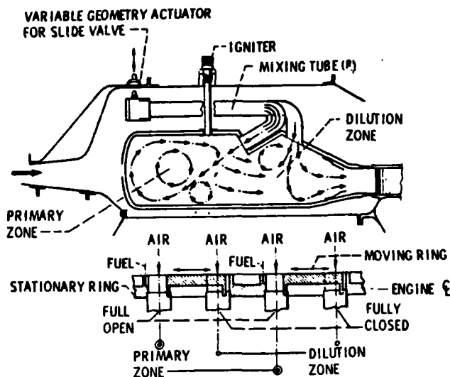
DEVELOPMENT OF VARIABLE SLIDE VALVE (a) JET-INDUCED-CIRCULATION (JIC) CONCEPT.
