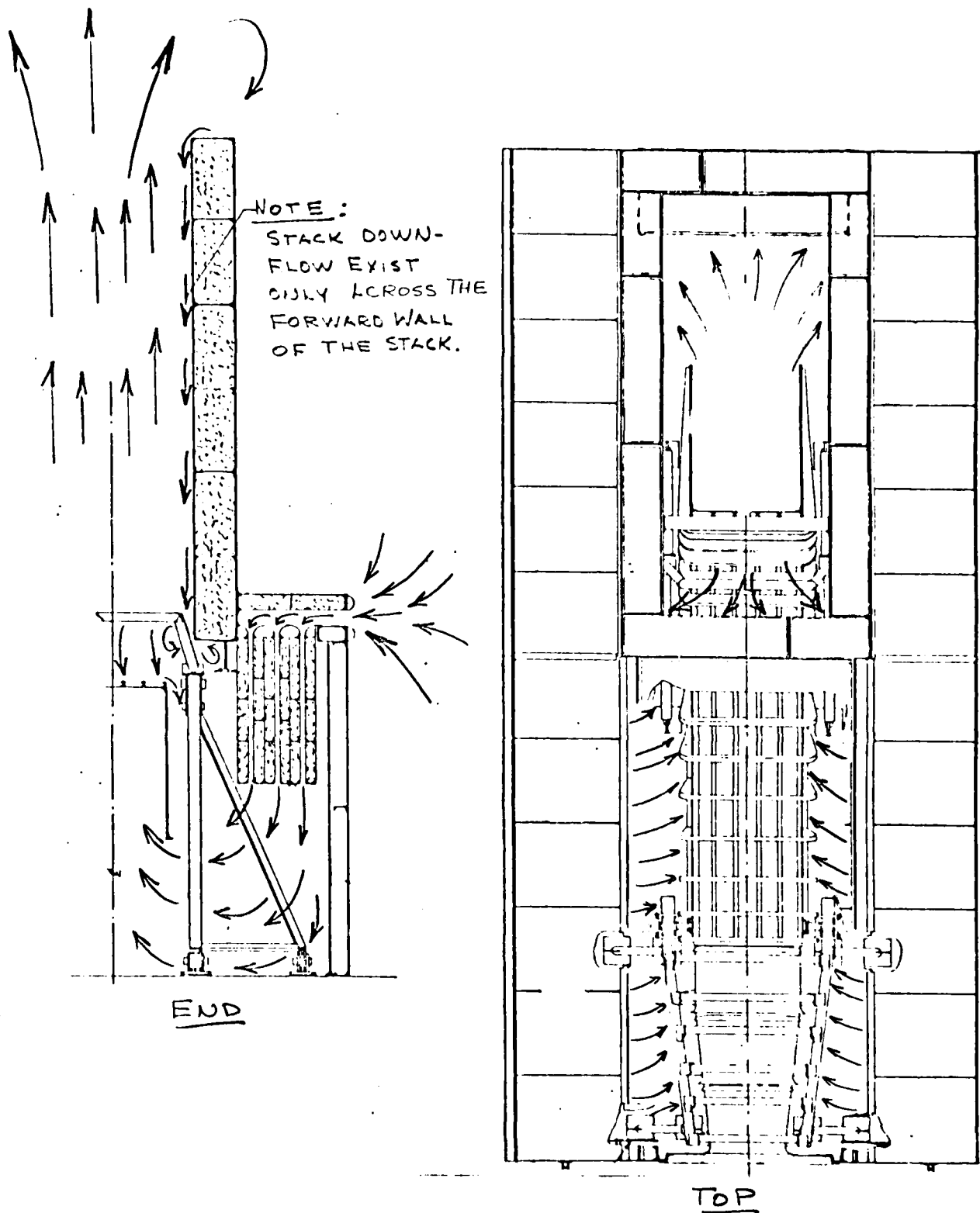
FIGURE 4, FLOW FIELD END & TOP VIEWS
