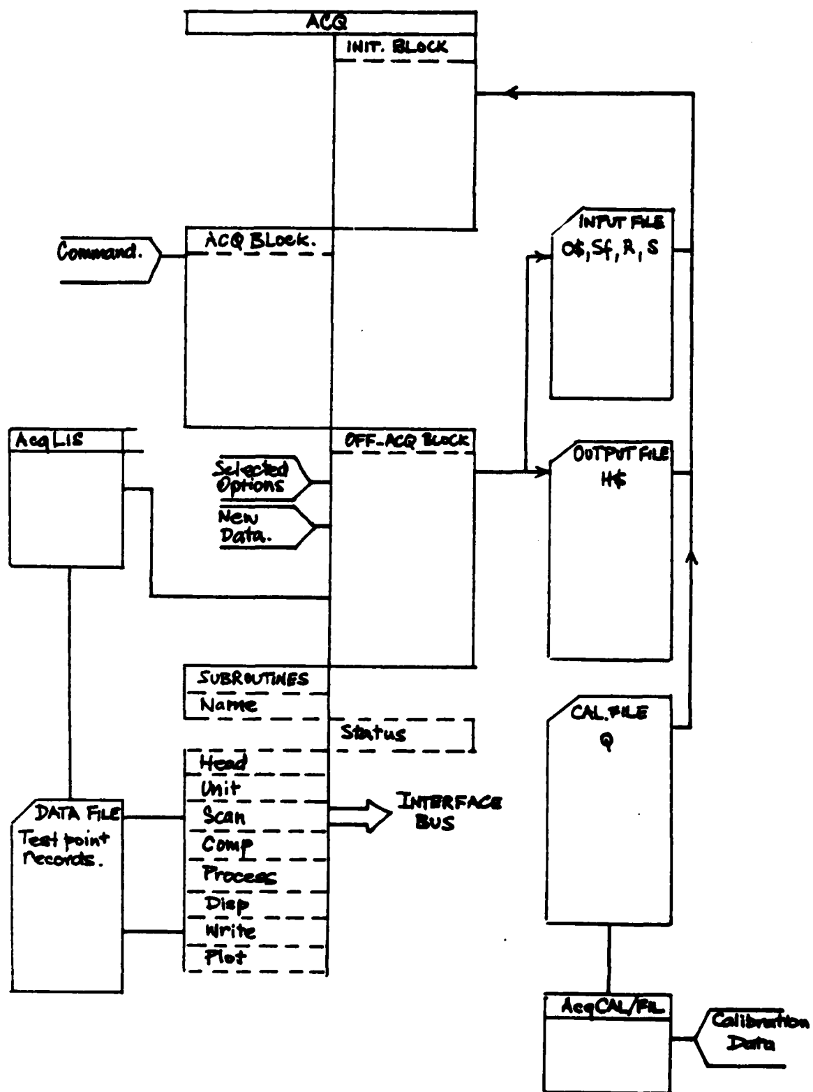
Figure 4.5(2) Block diagram of data reduction software.
