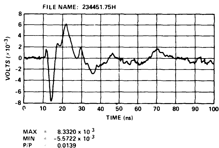
Figure 76. Configuration 9 test point 1, azimuth angle = 234 deg: (a) vertical polarization experiment and (b) horizontal polarization experiment, elevation angle = 45 deg (file names do not reflect correct configuration).
