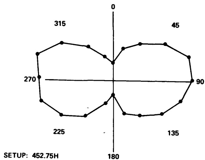
Figure 36. Configuration 7 polar plot for test point 2: elevation angle = 45 deg and polarization = horizontal.
