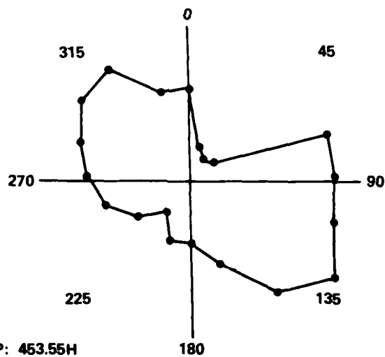
Figure 31. Configuration 5 polar plot for test point 3: elevation angle = 45 deg and polarization = horizontal.
