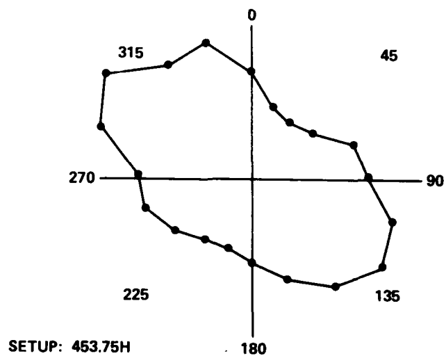
Figure 37. Configuration 7 polar plot for test point 3: elevation angle = 45 deg and polarization = horizontal.
