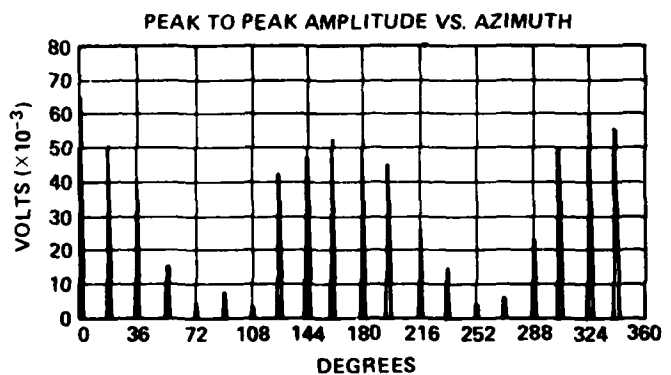
Figure 39. Configuration 2 histogram for test point 1: elevation angle = 45 deg and polarization = horizontal.
