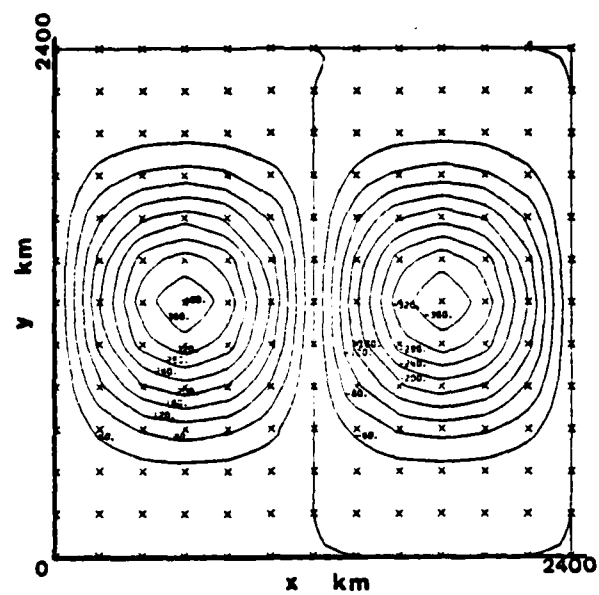
Figure 8. Initial field for the scalar S.
