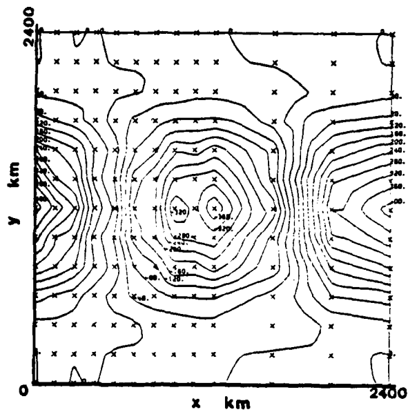
Figure 32. 24 hour forecast for field in figure 30.
