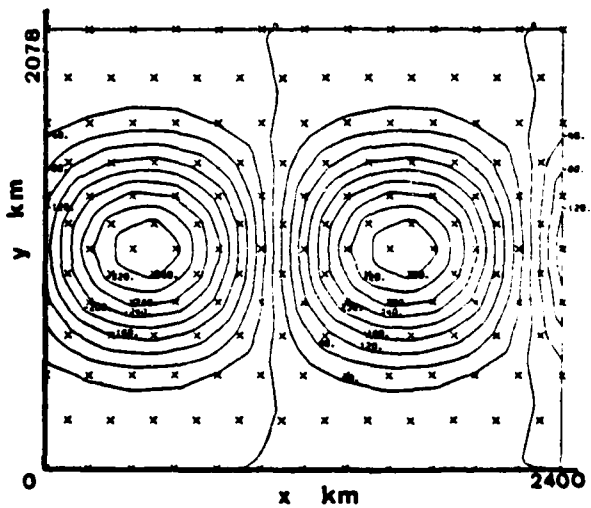
Figure 27. Analytic solution corresponding to figure 26.
