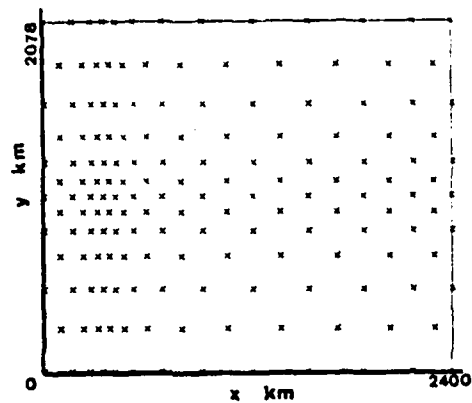
Figure 14. Same as figure 13 but r_1 = 5 , r_2 = 3 .
