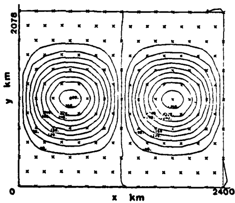
Figure 19. Initial S field for Robert filter tests.
