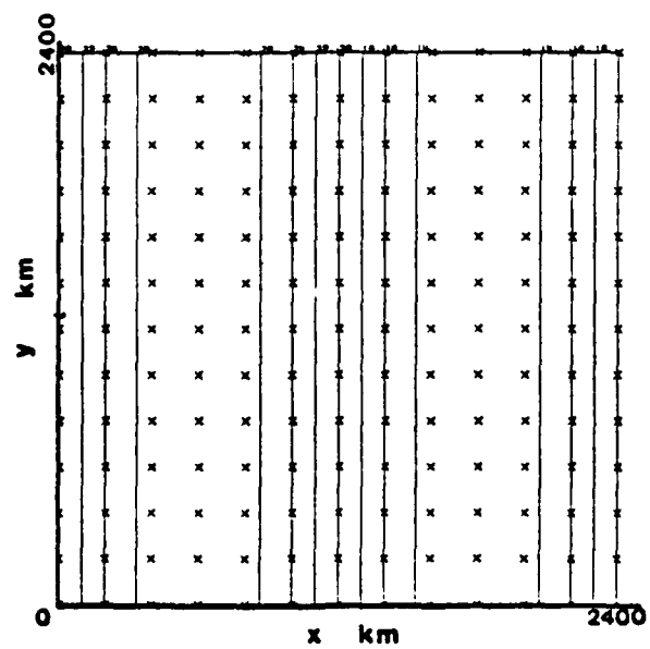
Figure 9. Initial u field with wind ratio R = 0.4 .
