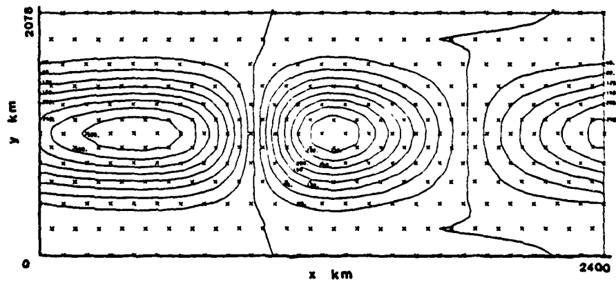
Figure 17. Same as figure 16 but with optimum diffusion.
