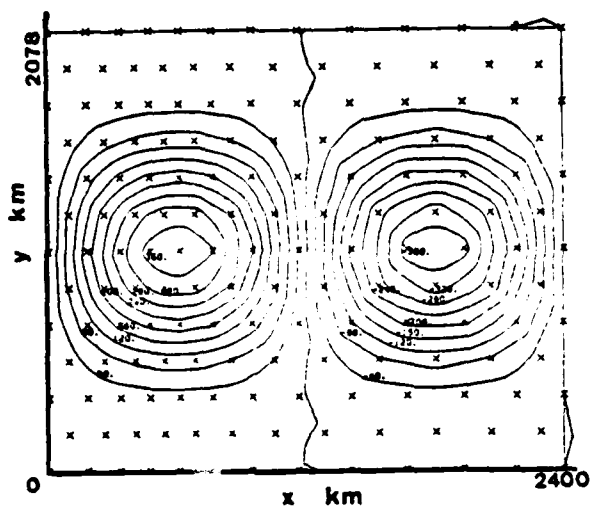
Figure 28. Initial S field for Case 2.
