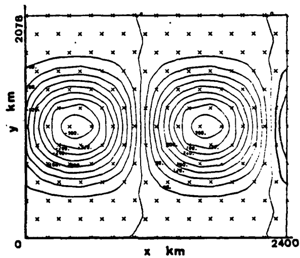
Figure 21. Analytic solution for Robert filter tests.
