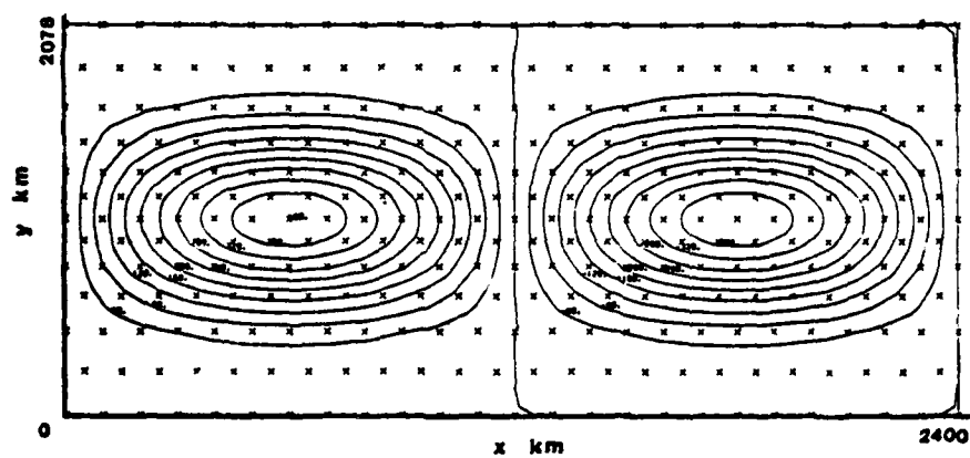
Figure 15. Initial S field for the diffusion tests.
