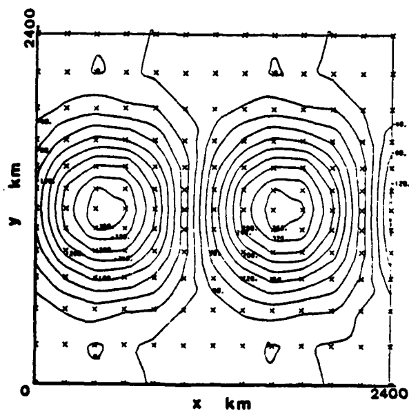
Figure 23. 48 hour forecast for field in figure 22.
