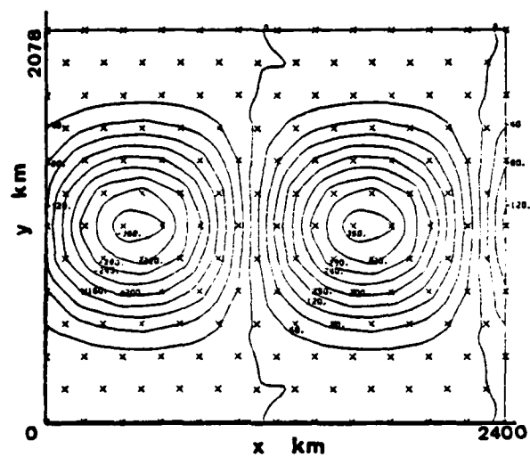
Figure 20. 48 hour forecast for field in figure 19.
