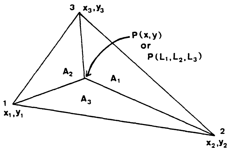
Figure 6. A typical element illustrating the area coordinate system.
