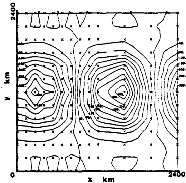
Figure 31. 12 hour forecast for field in figure 30.
