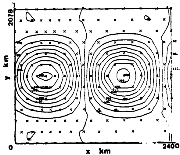
Figure 39. 48 hour forecast for field in figure 38.
