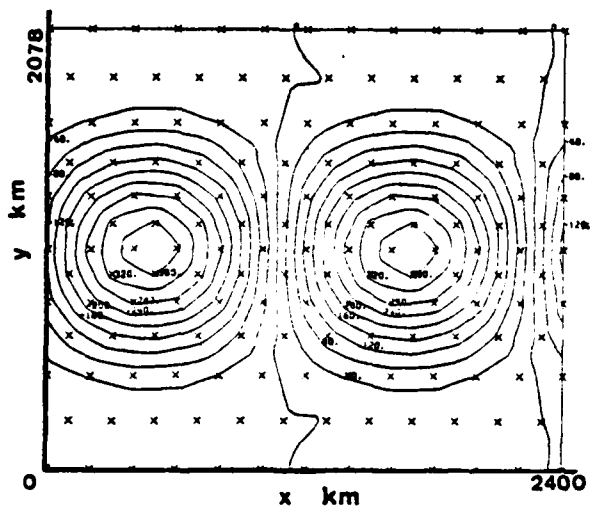
Figure 26. 48 hour forecast for field in figure 25.
