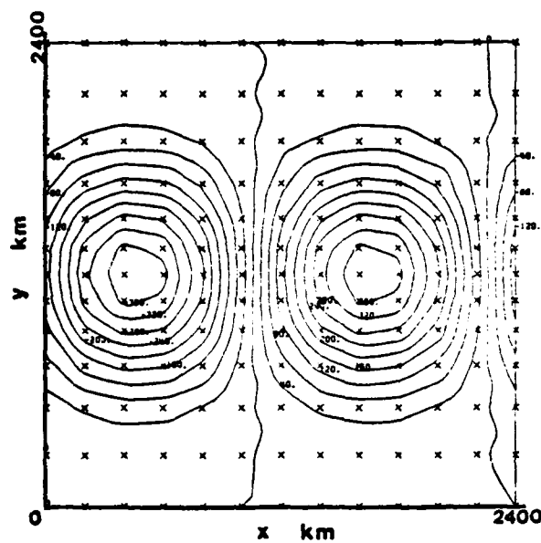
Figure 24. Analytic solution corresponding to figure 23.
