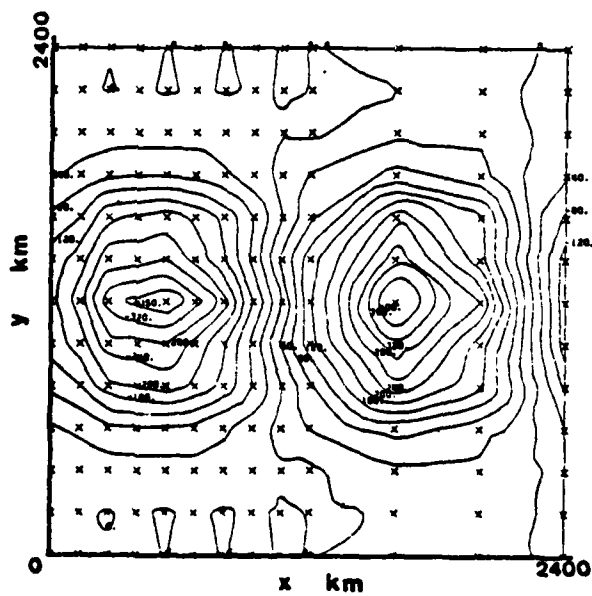
Figure 33. 48 hour forecast for field in figure 30.
