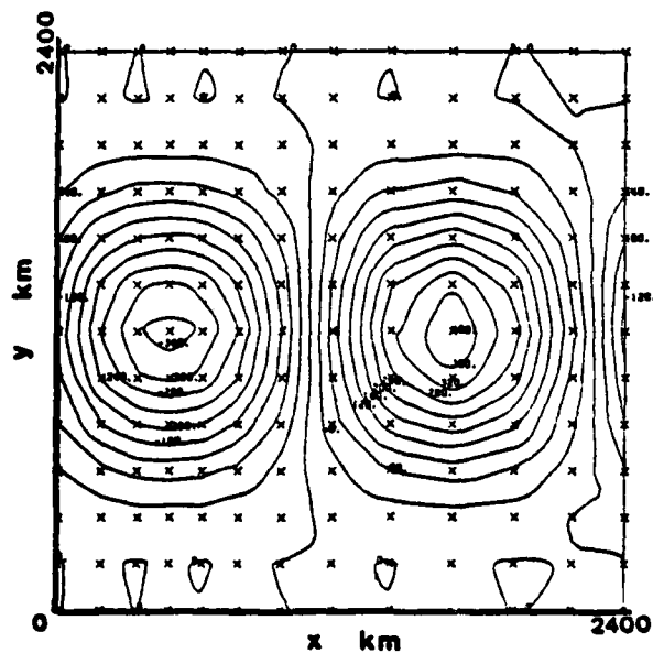
Figure 35. 48 hour forecast for field in figure 34.
