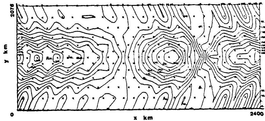
Figure 16. 48 hour forecast for field in figure 15 with no diffusion.
