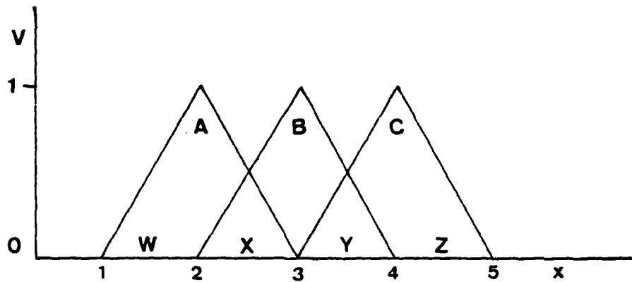
Figure 2. One-dimensional example of linear basis functions.
