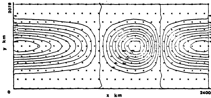
Figure 18. Analytic solution for diffusion tests.
