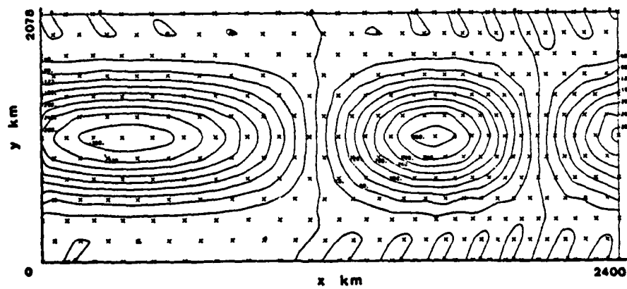
Figure 37. 48 hour forecast for field in figure 36.
