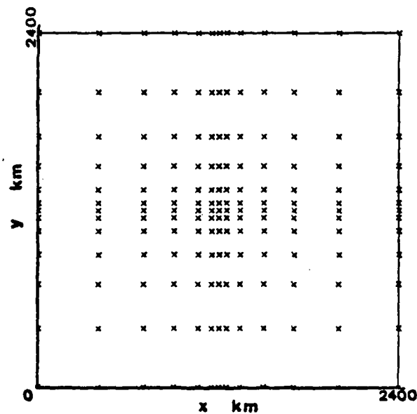
Figure 11. Same as figure 10 with non-uniform elements.
