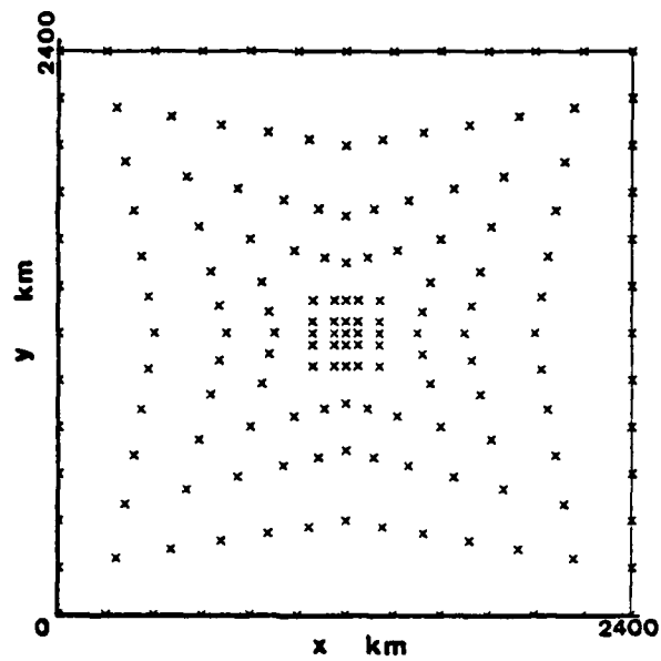
Figure 12. An alternate method of varying resolution.
