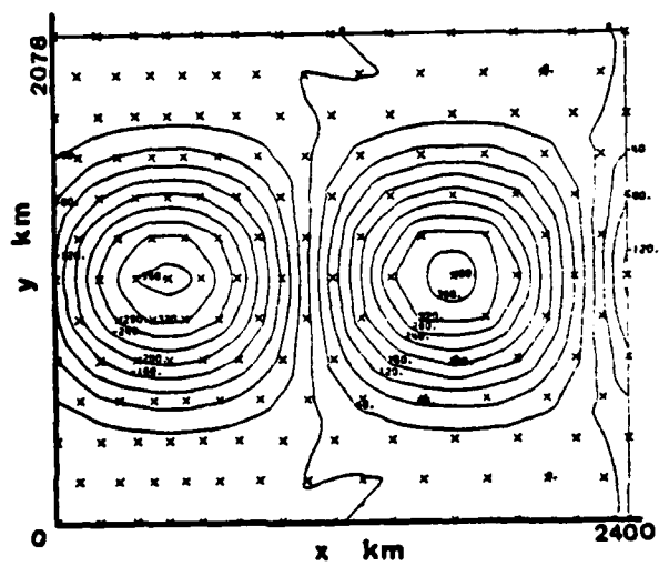
Figure 29. 48 hour forecast for Case 2.
