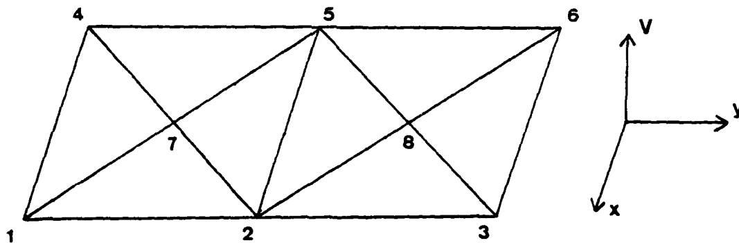
Figure 3. A domain with eight nodes and eight triangular elements.
