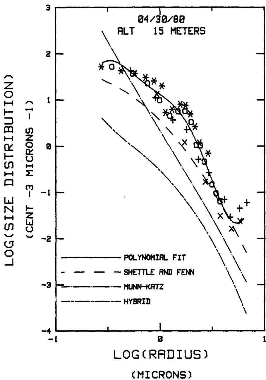
Figure 23a. Size Distribution, L #3, 15 Meters RELATIVE HUMIDITY 82.32, MIXING RATIO 7.48, WIND SPEED 4.1
