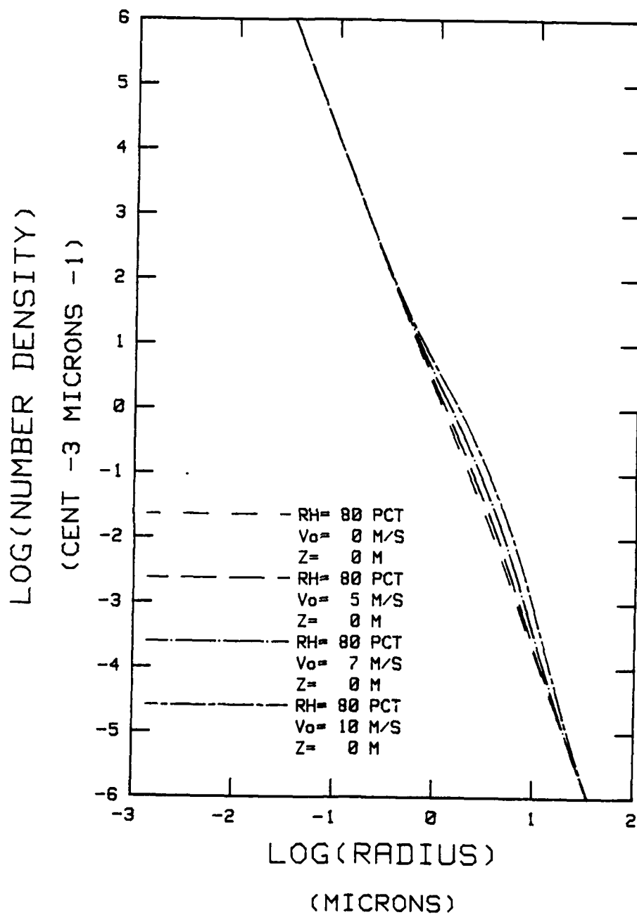
Figure 6. Munn-Katz Total Size Distribution Dependence on Wind Speed TOTAL SIZE DISTRIBUTION
