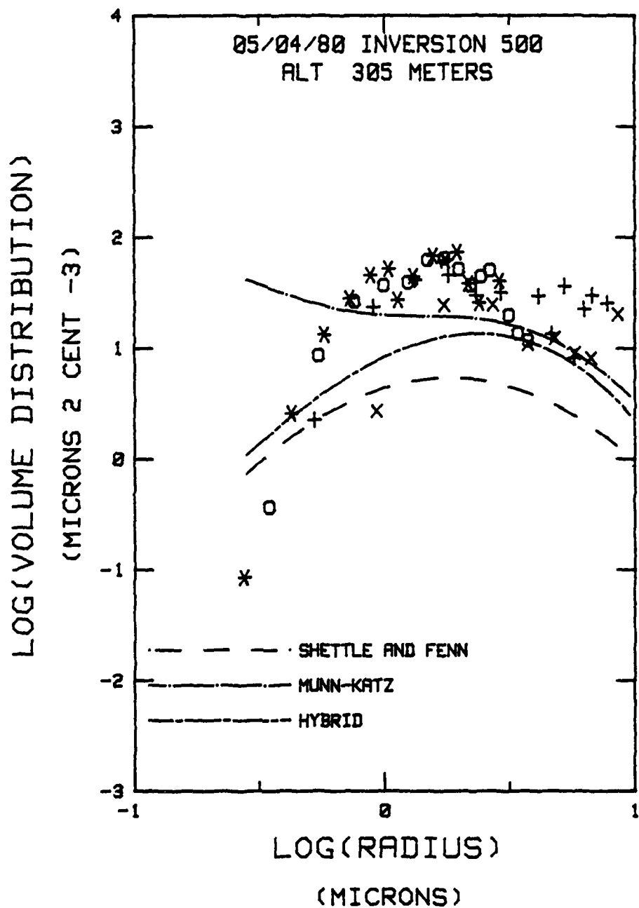
Figure 32b. Volume Distribution, L #16, 305 Meters RELATIVE HUMIDITY 88.84, MIXING RATIO 6.72, WIND SPEED 8.7
