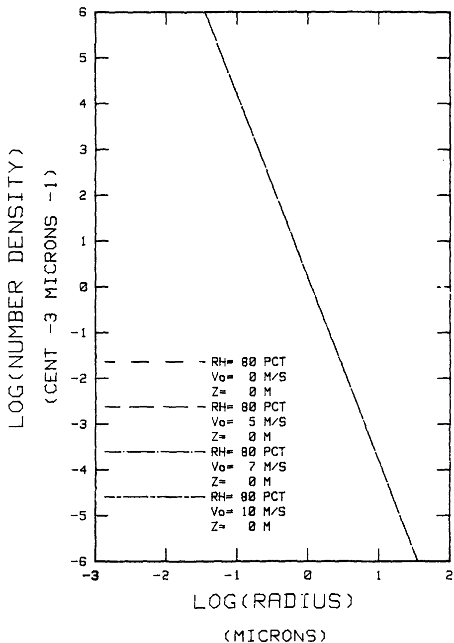
Figure 4. Munn-Katz Continental Dependence on Wind Speed
