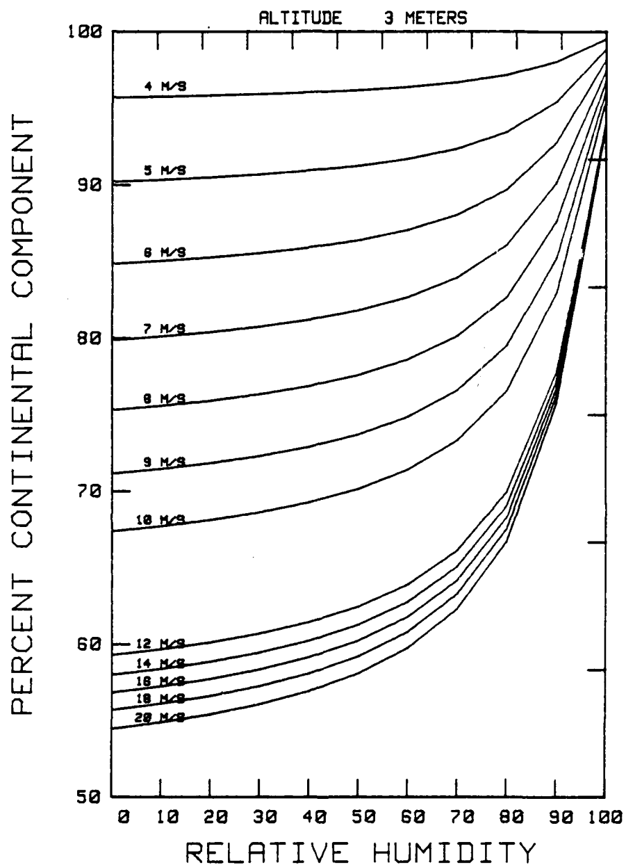
Figure 16. Hybrid Weighting Factor, 3 Meter Altitude PERCENT CONTINENTAL COMPONENT
