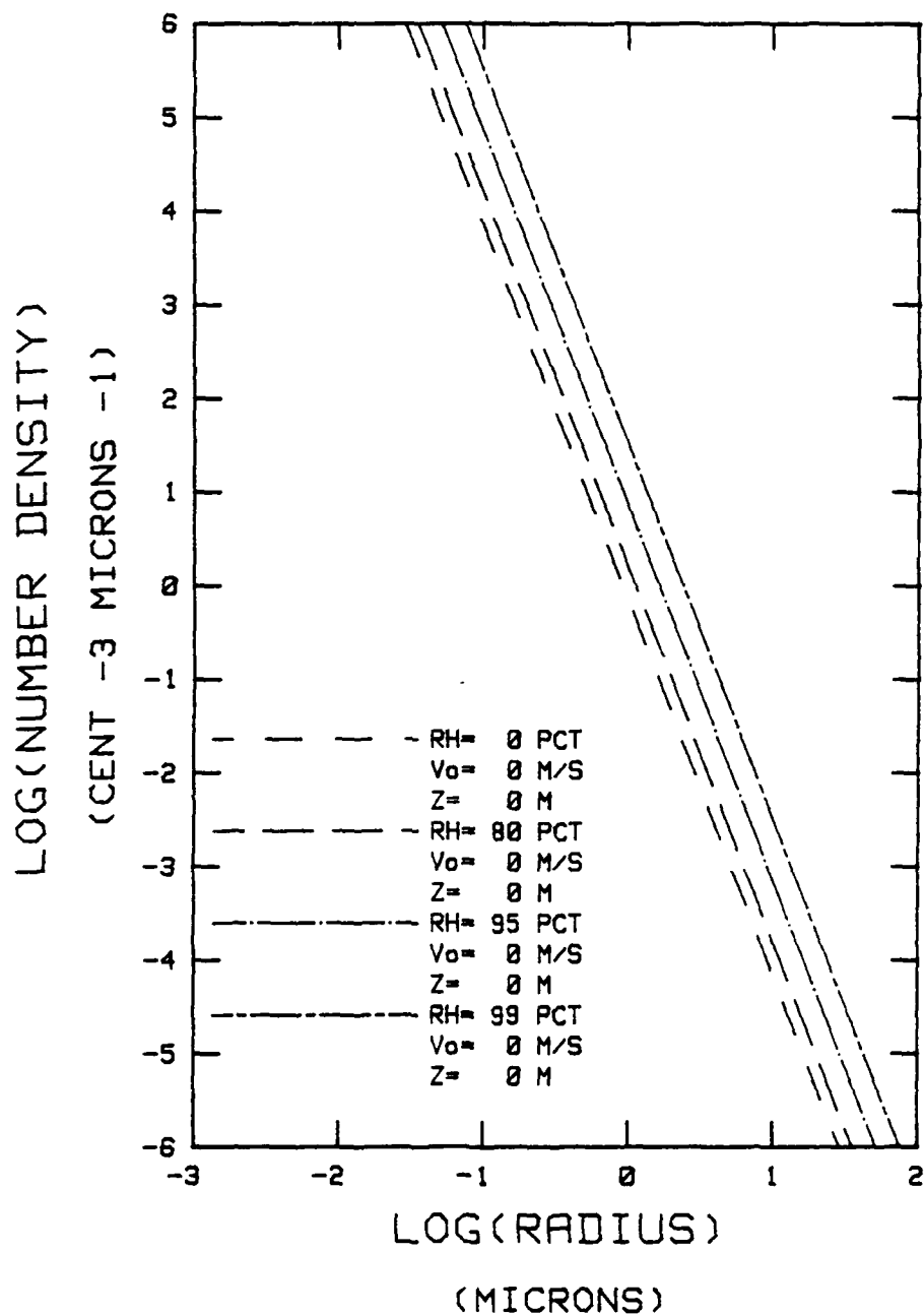
Figure 7. Munn-Katz Continental Dependence on Relative Humidity CONTINENTAL COMPONENT ONLY
