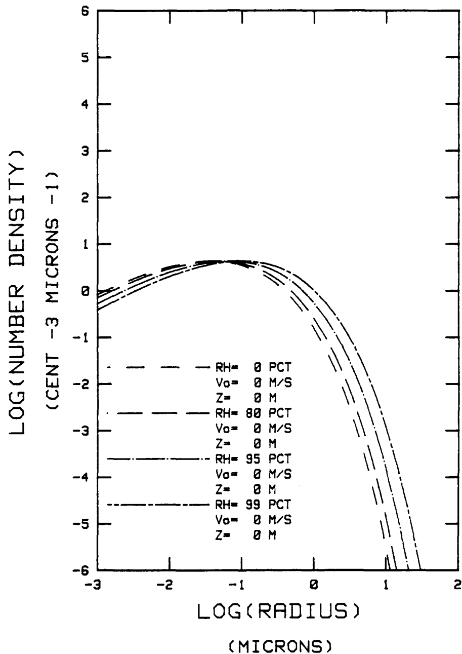
Figure 8. Munn-Katz Maritime Dependence on Relative Humidity MARITIME COMPONENT ONLY
