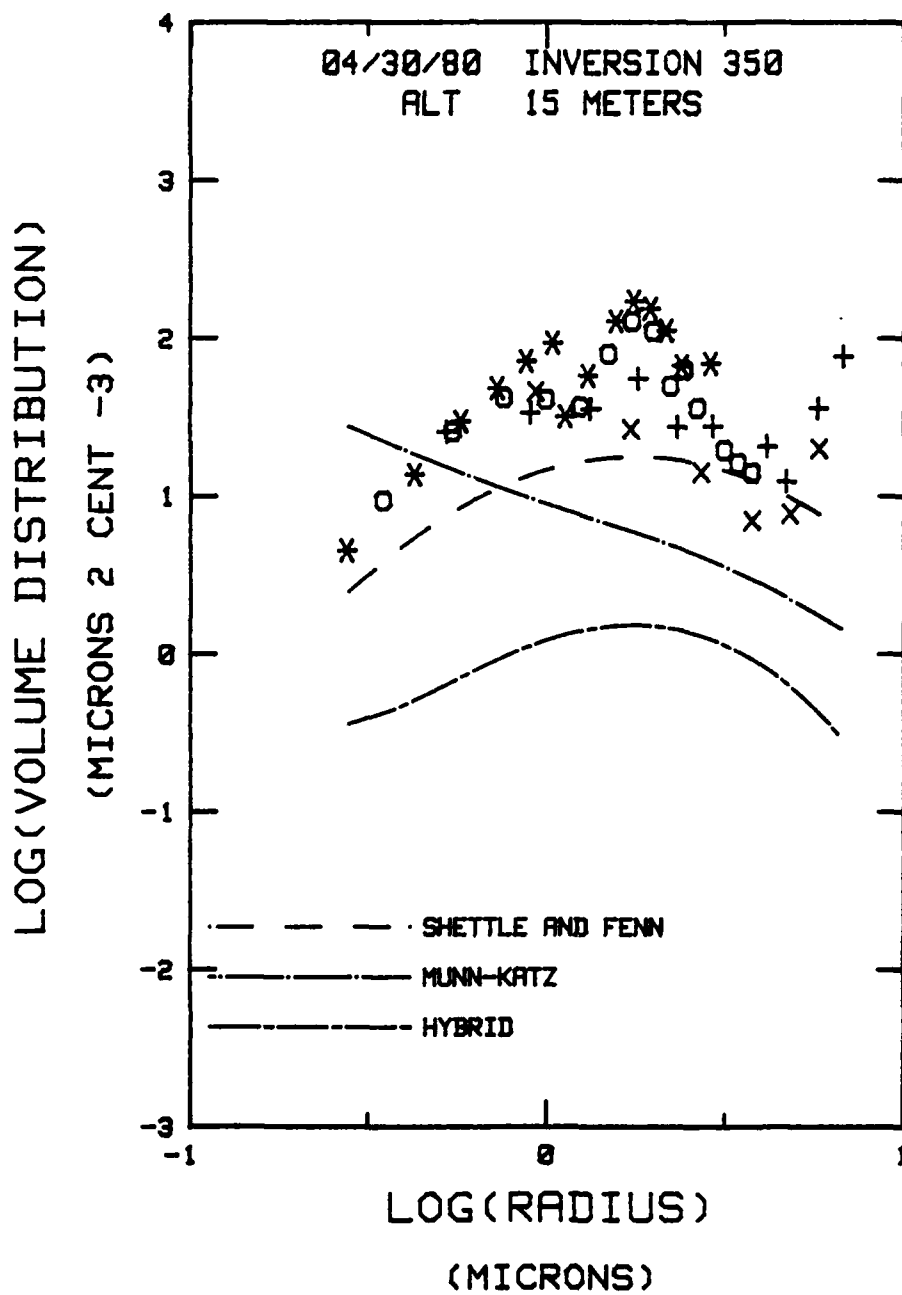
Figure 23b. Volume Distribution, L #3, 15 Meters RELATIVE HUMIDITY 82.32, MIXING RATIO 7.40, WIND SPEED 4.1
