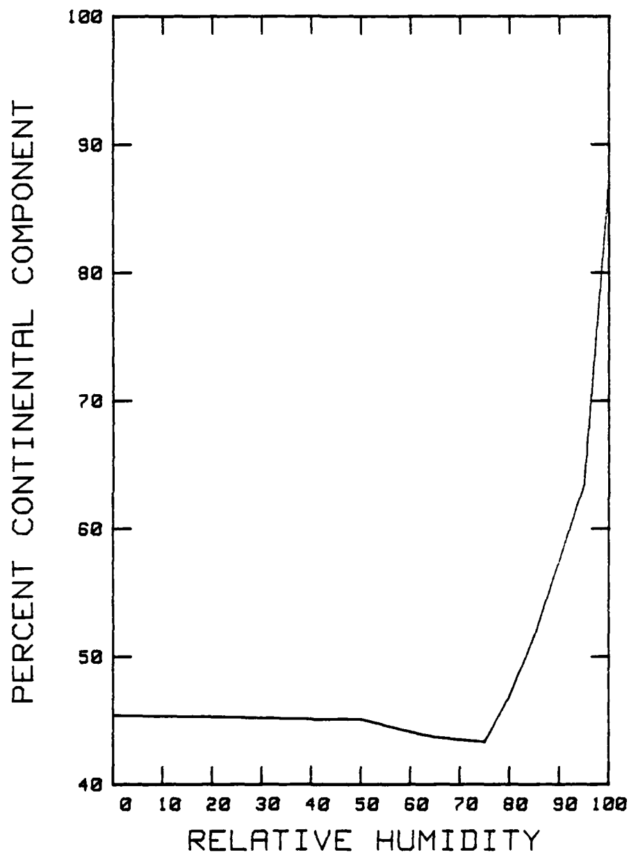
Figure 15. Shettle and Fenn Weighting Factor PERCENT CONTINENTAL COMPONENT AS A FUNCTION OF RELATIVE HUMIDITY
