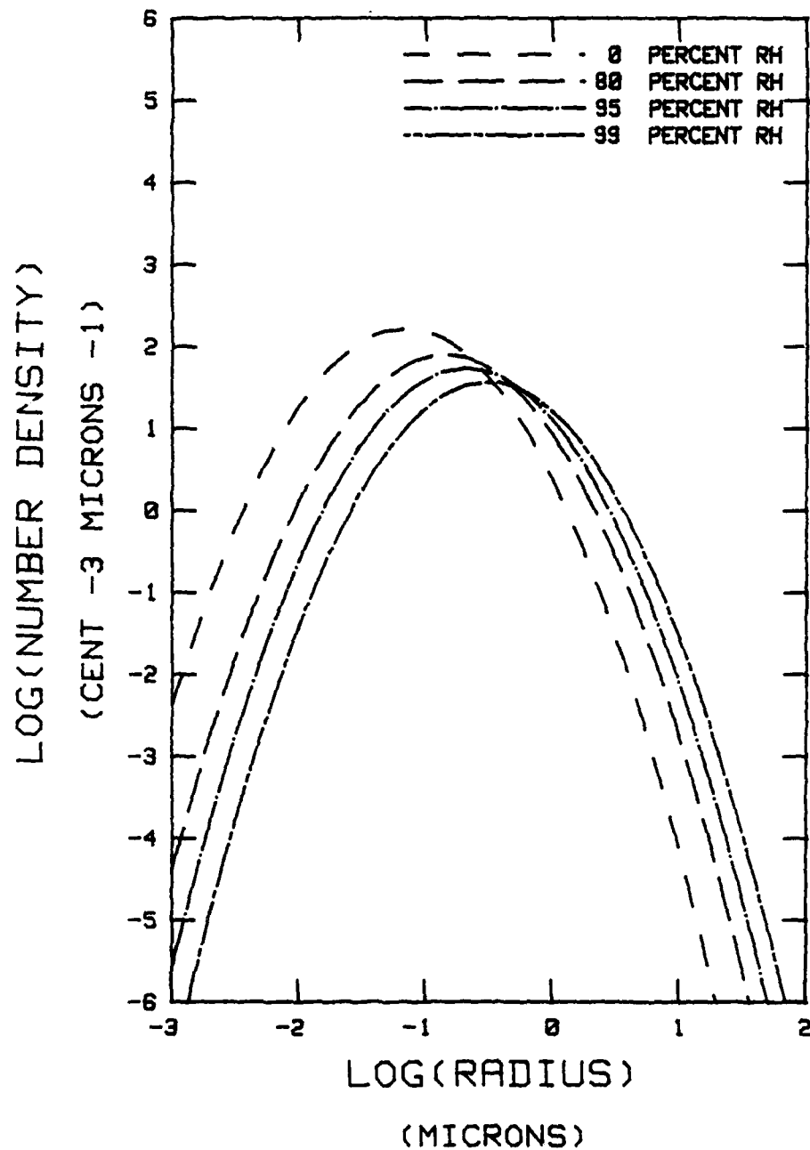
Figure 2. Shettle and Fenn Maritime (coarse) Component as a Function of Relative Humidity PARTICLE CONCENTRATION FIXED AT 40 \text{ CM}^{-3}
