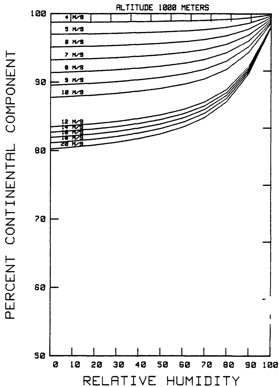
Figure 20. Hybrid Weighting Factor, 1000 Meter Altitude PERCENT CONTINENTAL COMPONENT
