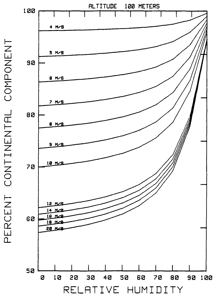
Figure 18. Hybrid Weighting Factor, 100 Meter Altitude PERCENT CONTINENTAL COMPONENT
