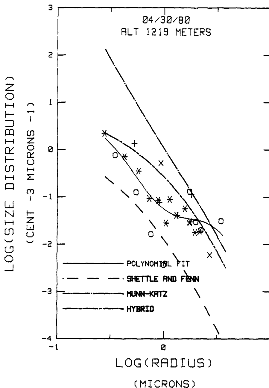
Figure 30a. Size Distribution, L #4, 1219 Meters RELATIVE HUMIDITY 20.48, MIXING RATIO 2.37, WIND SPEED 7.7
