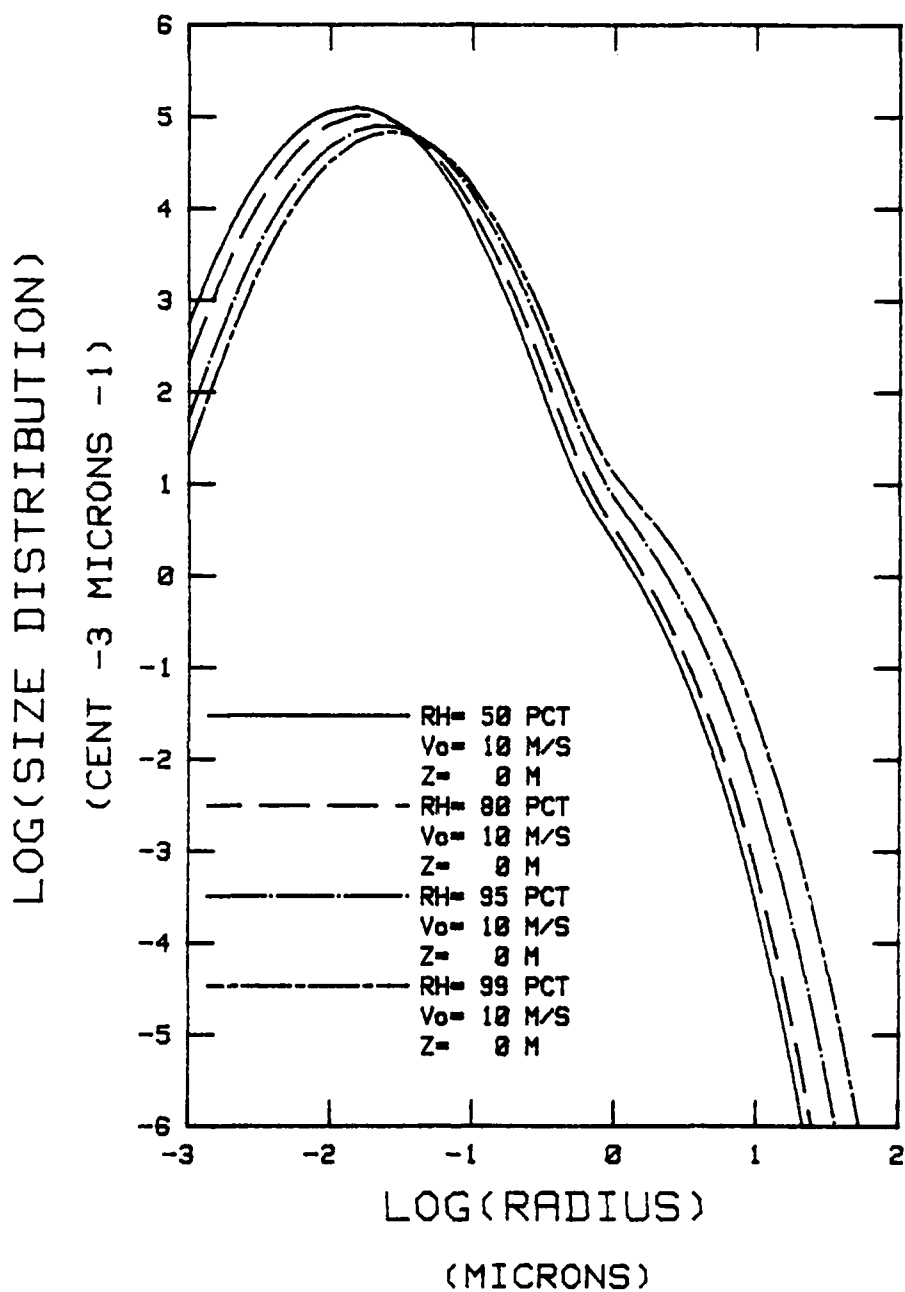
Figure 11. Hybrid Dependence on Relative Humidity at a Wind Speed of 10 m/s CONTINENTAL COMPONENT PARTICLE CONCENTRATION IS 5000 \text{cm}^{-3}
