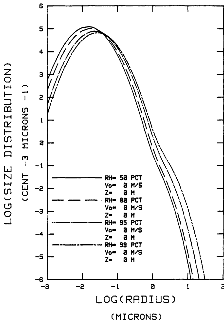
Figure 10. Hybrid Dependence on Relative Humidity at a Wind Speed of 0 m/s CONTINENTAL COMPONENT PARTICLE CONCENTRATION IS 5000 cm -3
