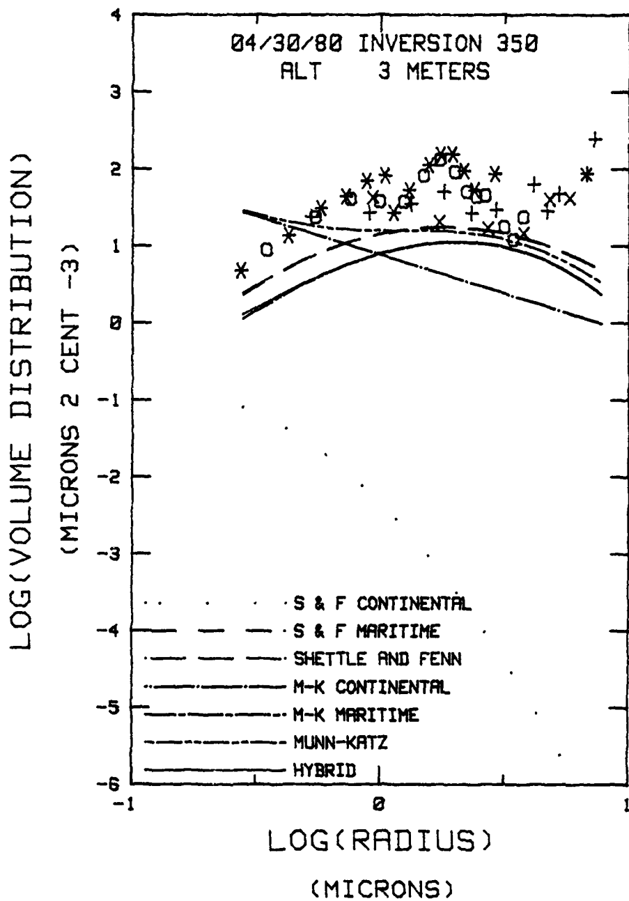
Figure 36. L #4 Volume Distribution, 3 Meters, Model Components RELATIVE HUMIDITY 82.12, MIXING RATIO 7.41, WIND SPEED 7.7
