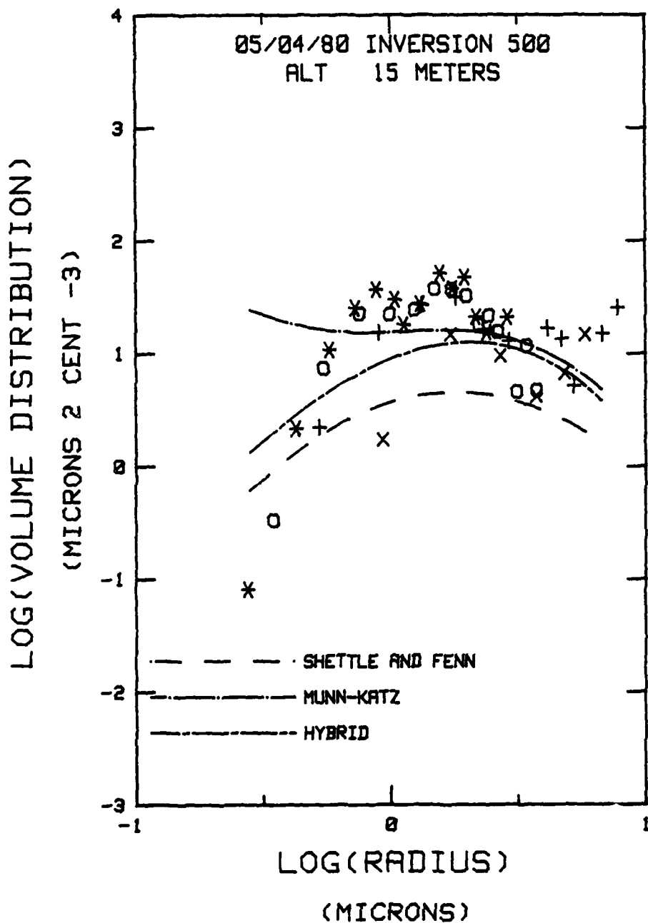
Figure 31b. Volume Distribution, L #16, 15 Meters RELATIVE HUMIDITY 77.83, MIXING RATIO 6.79, WIND SPEED 8.7
