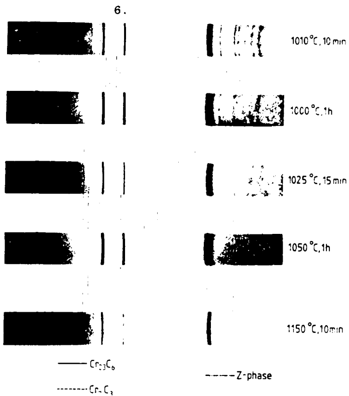
Figure 5(a) X-ray powder photographs showing the phases present in Nitronic 50 heat treated at 1000 to 1150°C
