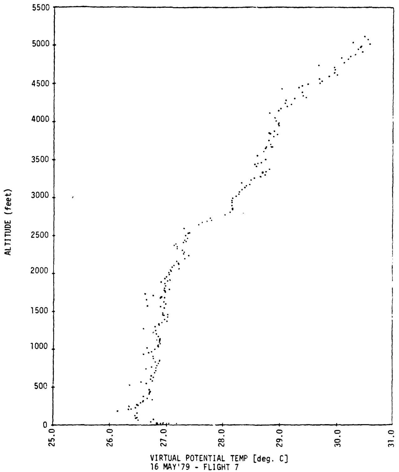
Figure 4.1(a) - Vertical distribution of virtual potential temperature during Flight #7. Taken from Ruhnke (1979).
