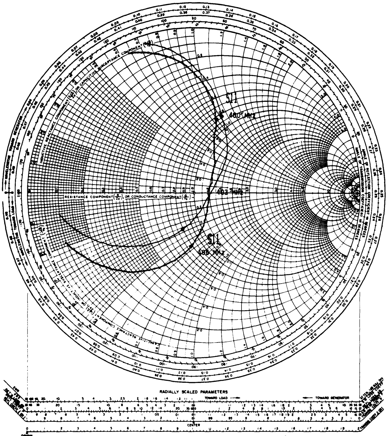
Figure 3-7. 403 MHz SAW Matched Reflection Coefficients
