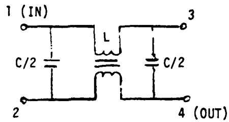
Figure 3-15 COUPLER SCHEMATIC
