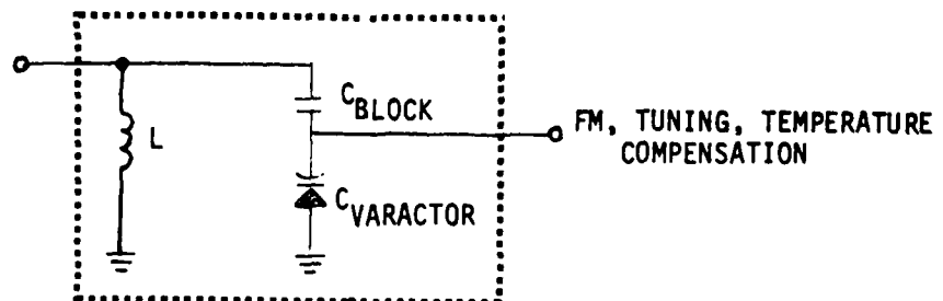
Figure 3-16. COUPLER LOAD
