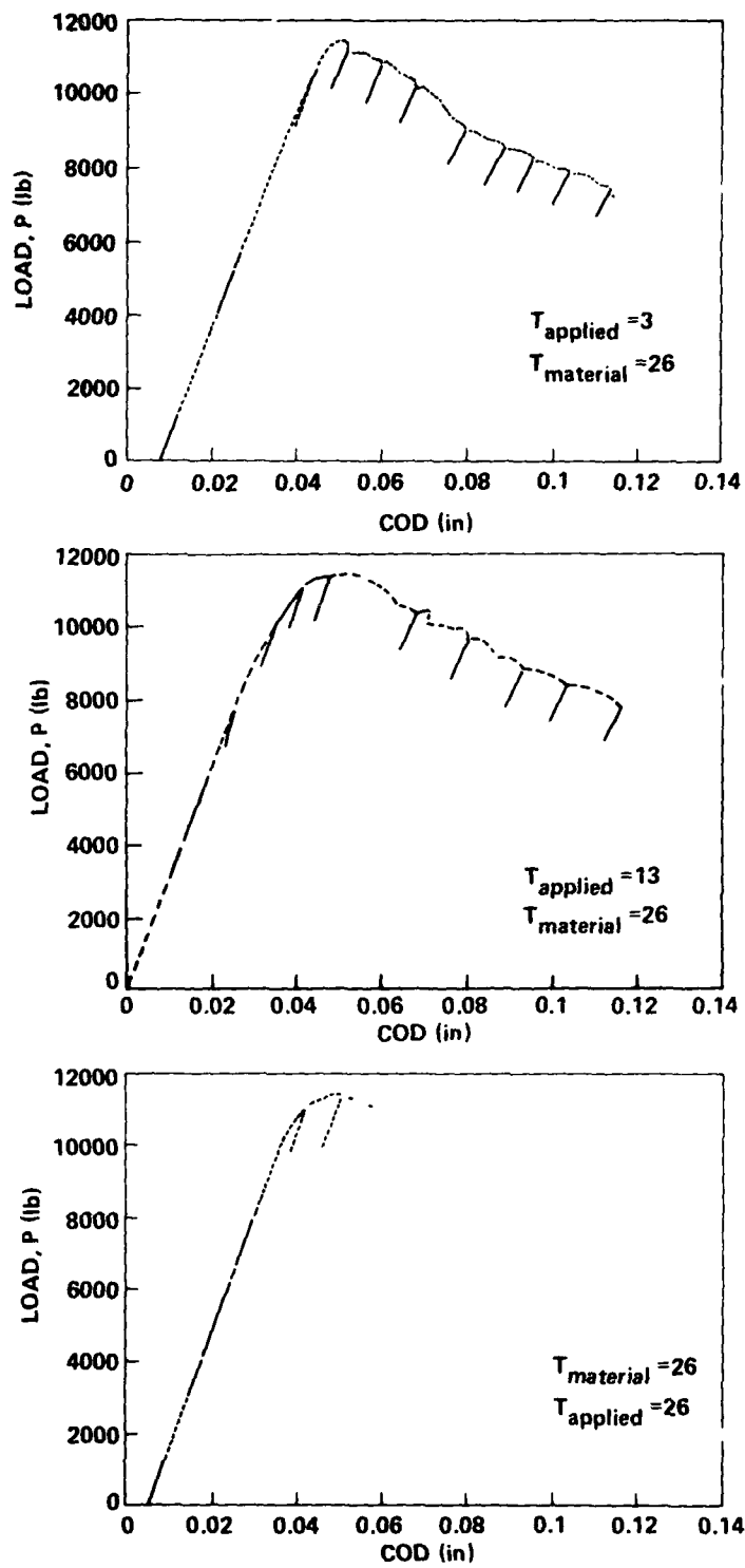
Figure 3 - Load Displacement Records for Three General Types of Tearing Behavior on HY-130 Steel
