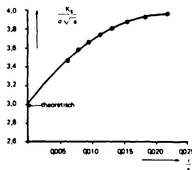
Fig 3.10 Determination of stress intensity for an edge crack specimen
