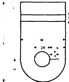
Fig 7.1 Laying down lug geometry by typical parameters
