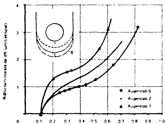
Fig 8.8 Crack propagation rate for lugs 2, 6 and 7
