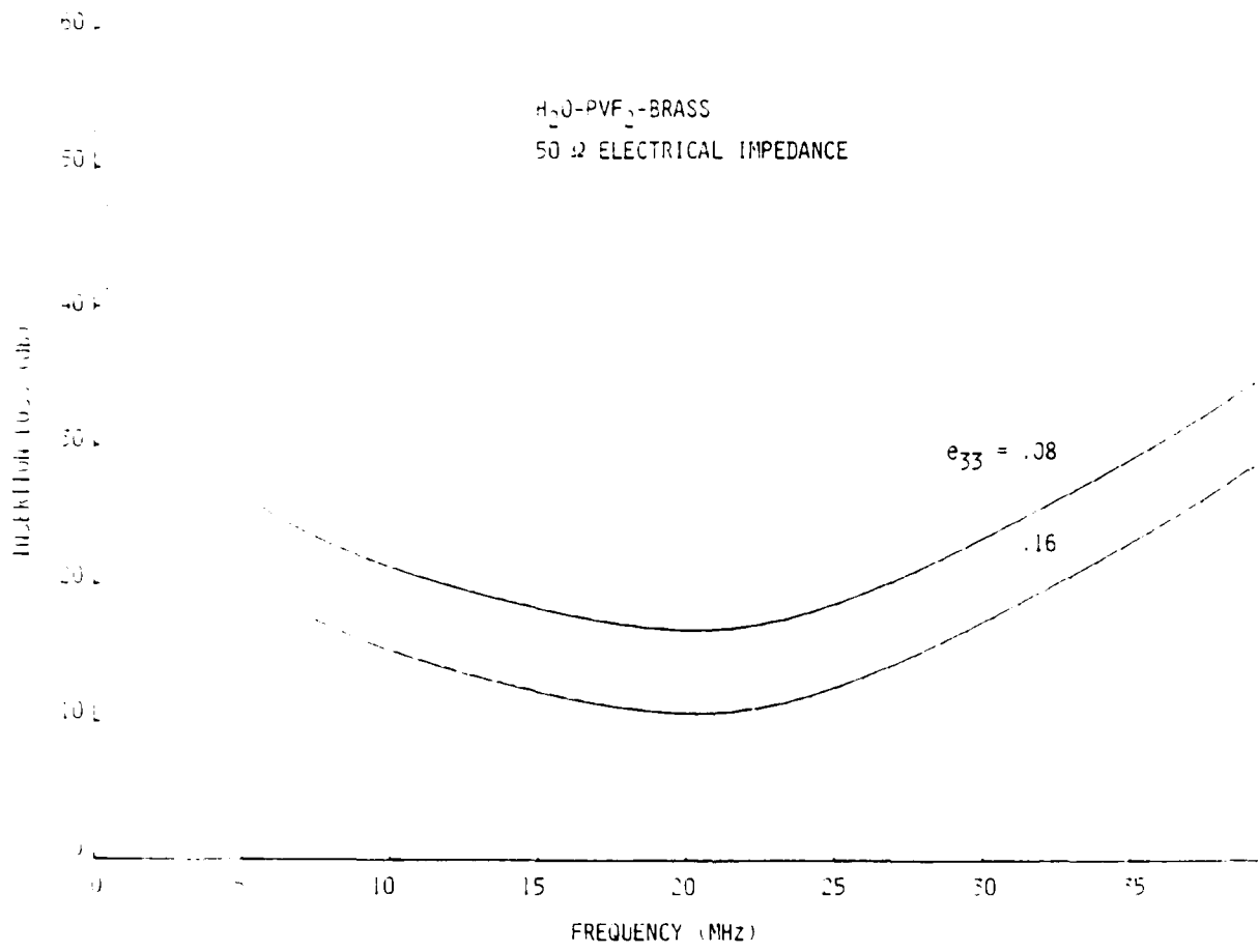
Fig. 7--Theoretical insertion loss of idealized bulk wave transducers. Backing material brass; PVF 2 film thickness 25 μ; film area 1 cm; film \epsilon/\epsilon_0 = 8 .
