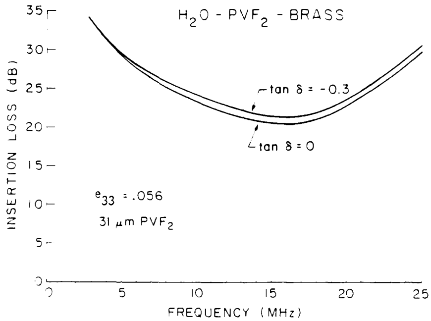
Fig. 8--Theoretical effect of dielectric loss. Backing material brass; electrical impedance 50 \Omega ; \text{PVF}_2 film thickness 31 \mu ; film area 1 \text{ cm}^2 ; film \epsilon/\epsilon_0 = 7 ; e_{33} = .056 .
