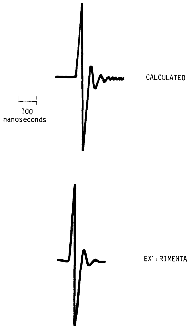
Fig. 14--Comparison of calculated and experimental PVF 2 transducer impulse response. The transducer was brass-backed and operated into a water load. Film area = 1 cm 2 , film thickness = 25 μm.
