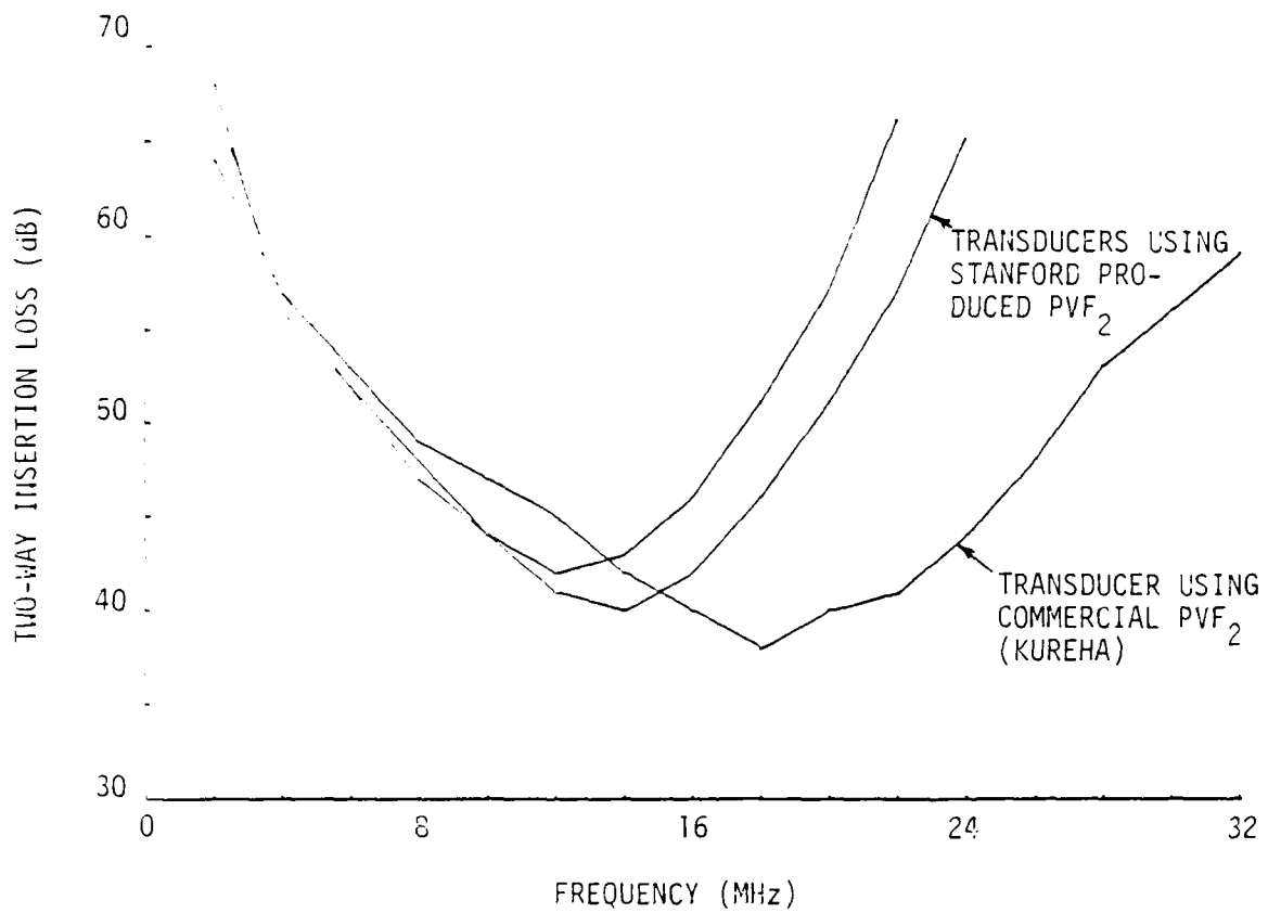
Fig. 20--Measured two-way insertion loss curves for transducers using Stanford and Kureha films.
