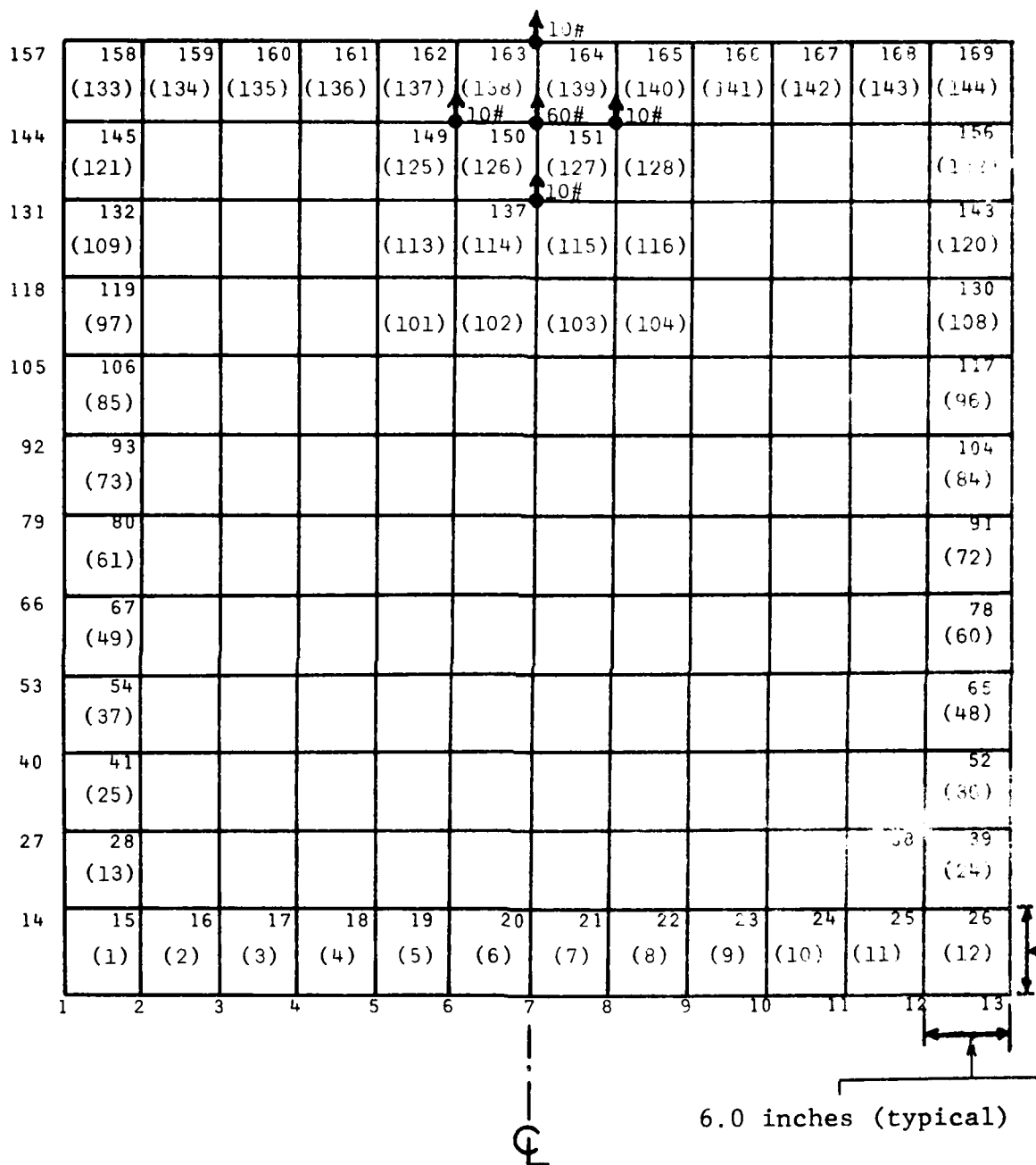
Figure 2. Nodes and Elements Used in the Preliminary Finite Element Analysis of the T17 FOD Cover. Node Numbers are Given Just to the Lower Left of the Nodes and Element Numbers are Given in the Middle of the Elements. The Load is Shown to the Right of the Arrows With A # Symbol.
