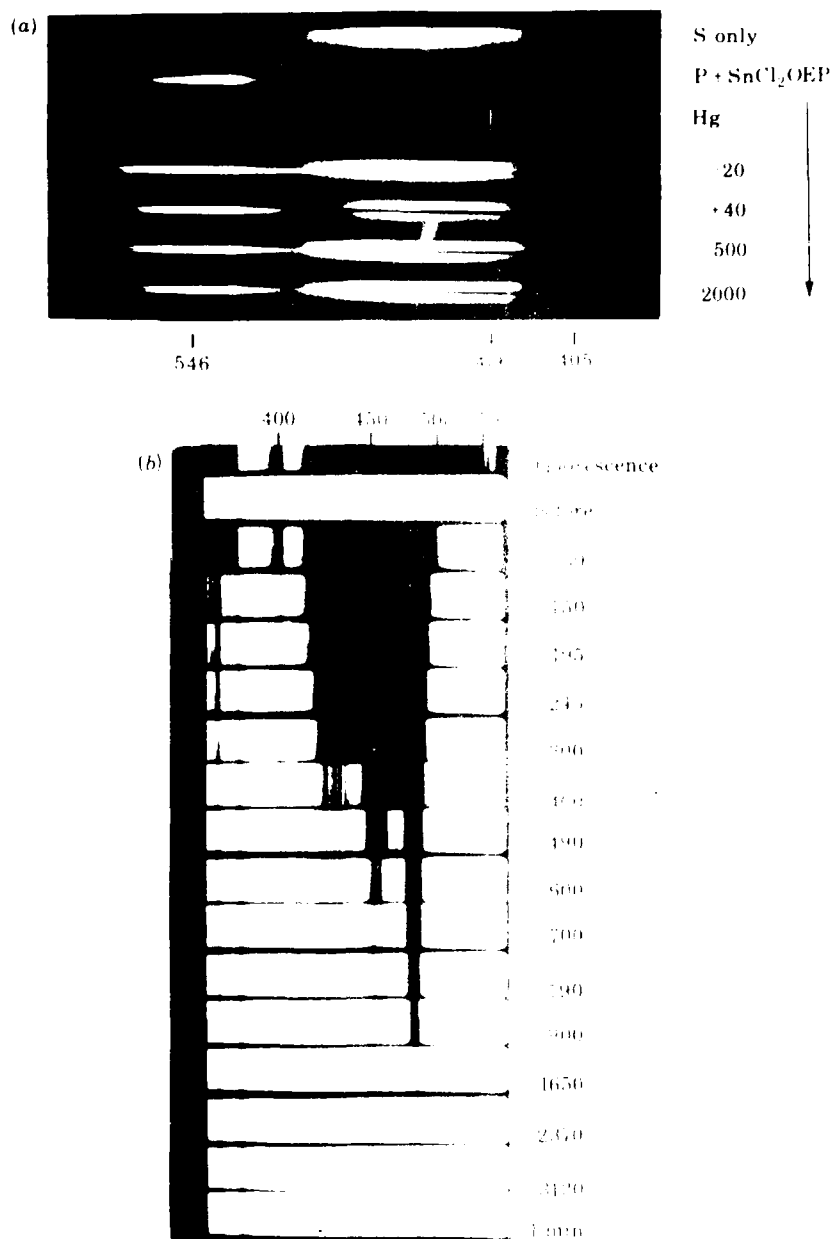
FIGURE 2. (a) Picosecond flash photolysis of tin dichlorooctethyl porphyrin, showing decay of excited singlet absorption (short-lived) and triplet absorption (longer-lived). (b) Conventional flash photolysis of 1,2-benzanthracene in viscous paraffin solution showing decay of triplet absorption. Time scale in microseconds.
