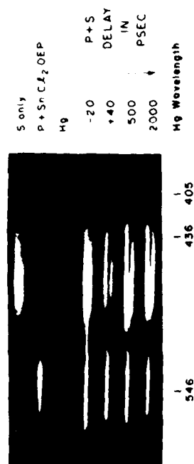
Fig. 5.15. Photographic record of excited state decay of [(OEP) \text{SnCl}_4 ] in 1,2-dichloroethane showing both S_1 and T_1 absorption as studied by Magde et al. [57]. The persistent excited-state absorbance due to the T_1 state is particularly evident in the 500- and 2000-psec exposures.
