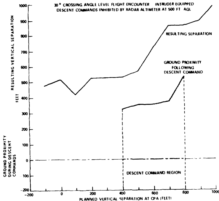
FIGURE 19. DESCENT COMMANDS NOT INHIBITED BY RADAR ALTIMETER (INTRUDER EQUIPPED — 30° CROSSING ANGLE)
