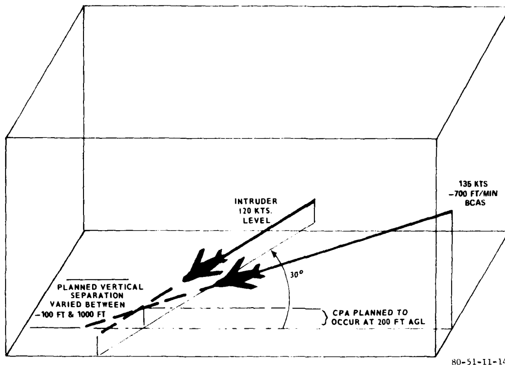
FIGURE 15. BASIC GEOMETRY FOR ILS ENCOUNTER WITH LEVEL FLIGHT CROSSING INTRUDER
