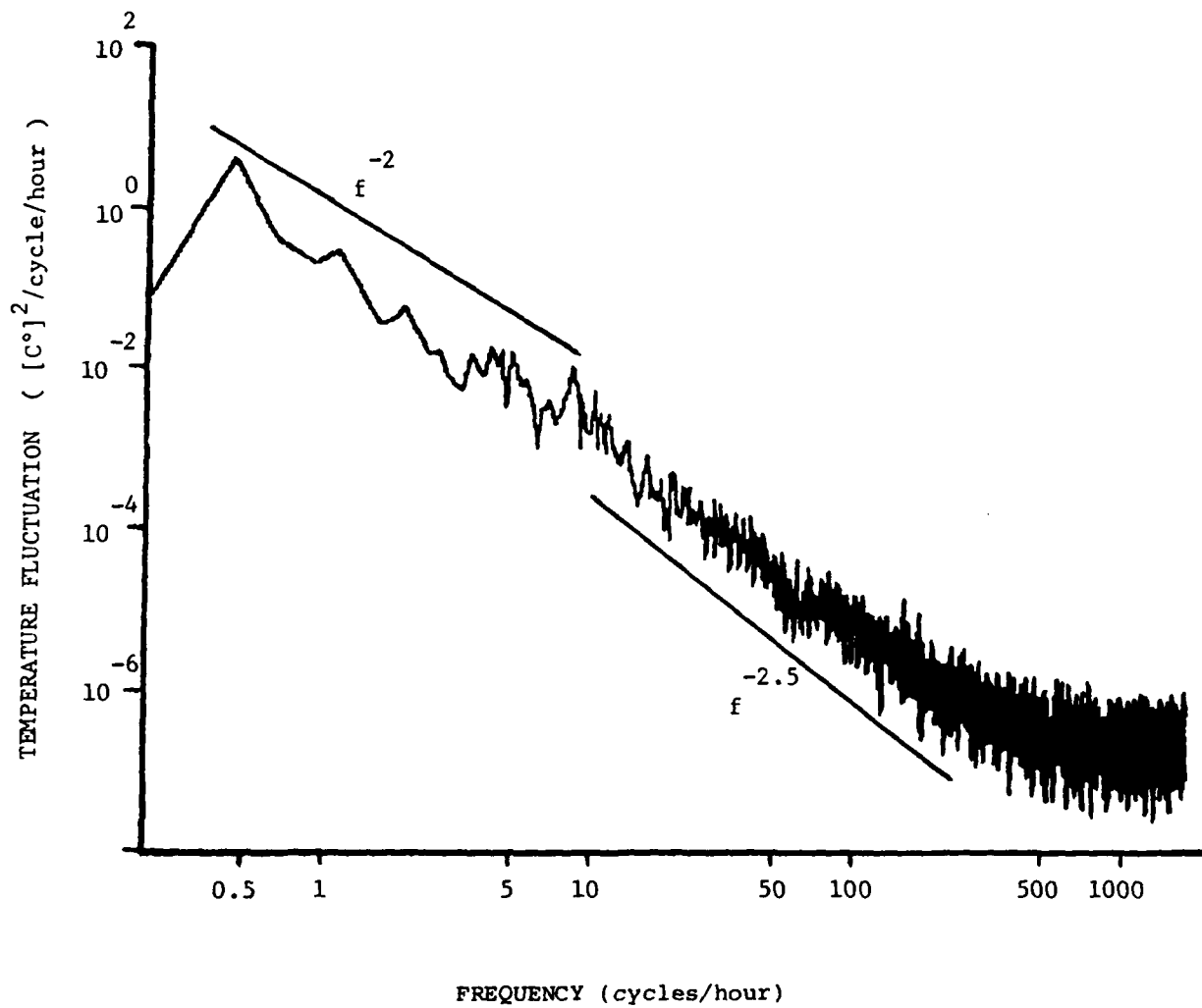
Figure 9. Averaged energy density spectrum of temperature fluctuations observed at ten sensors in upper half of the array.
