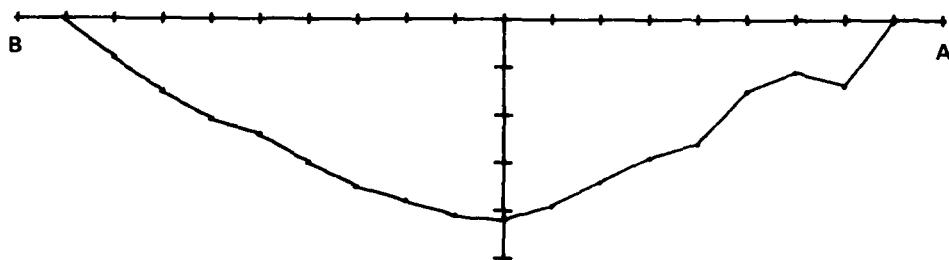
Figure C-36. Crater 31 (TNT).
