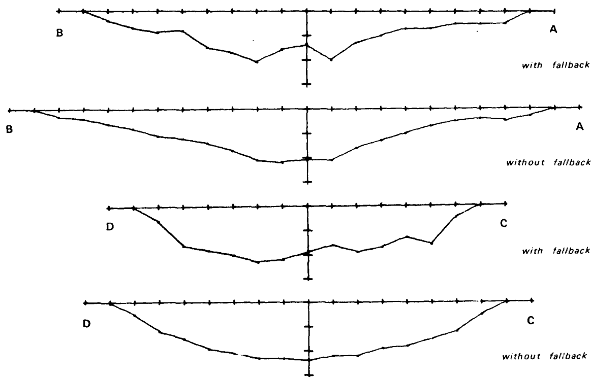
Figure C-19. Crater 13 (105mm).
