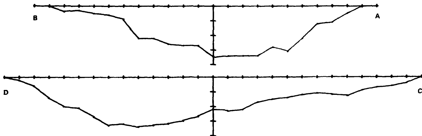
Figure C-51. Crater 46 (155mm).
