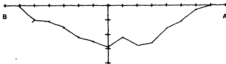
Figure C-10. Crater 1 (TNT).
