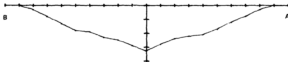
Figure C-27. Crater 21 (TNT).
