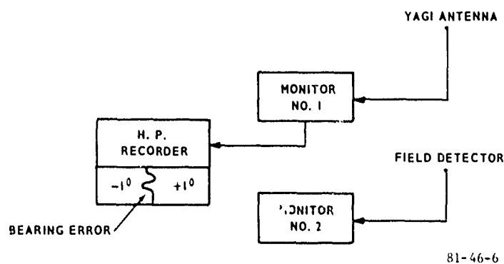
FIGURE 6. TEST SETUP TO DETERMINE PROPER FIELD DETECTOR ELEMENT LENGTH
