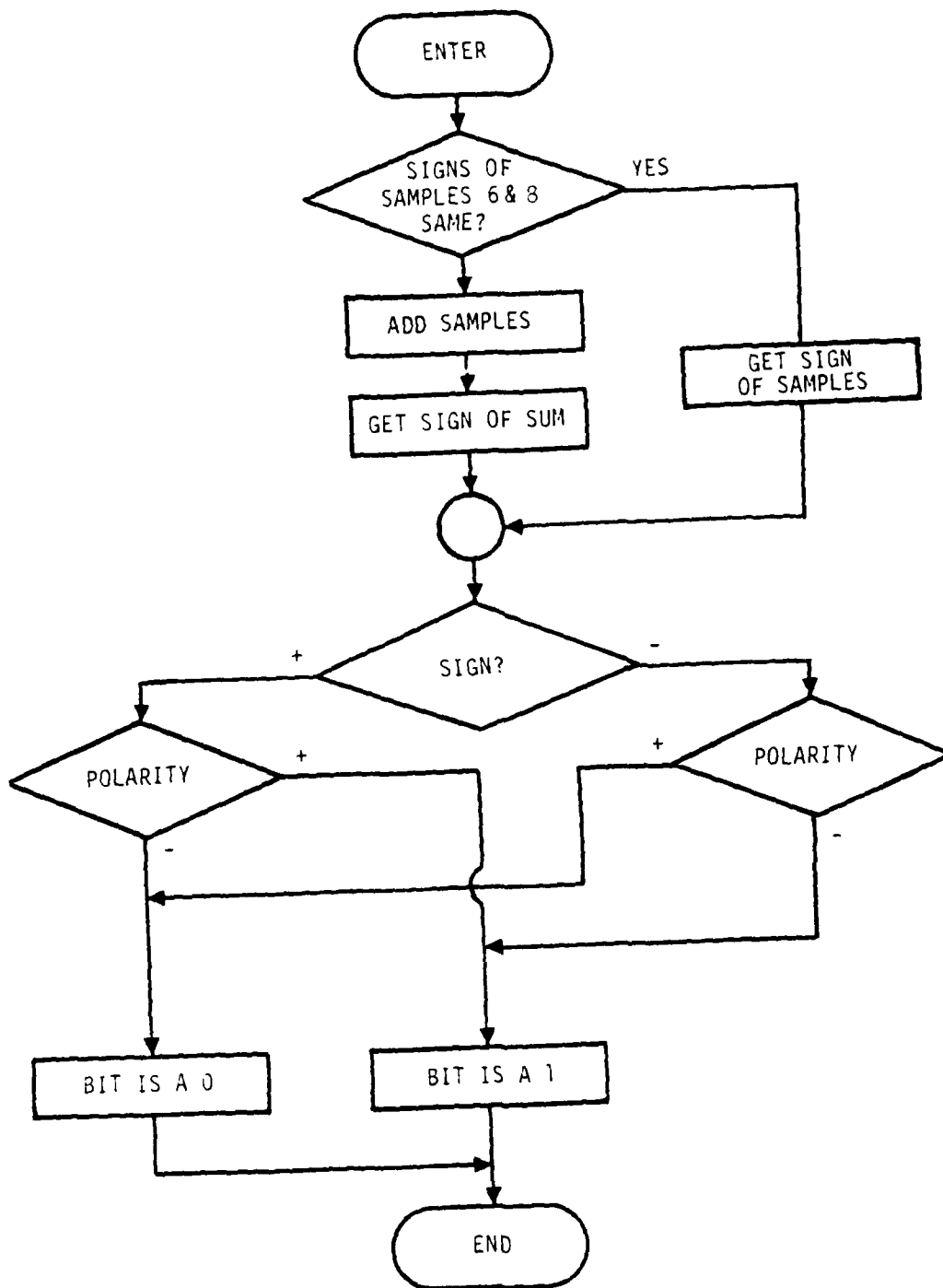
FIGURE 7. BIT PROCESSING.
