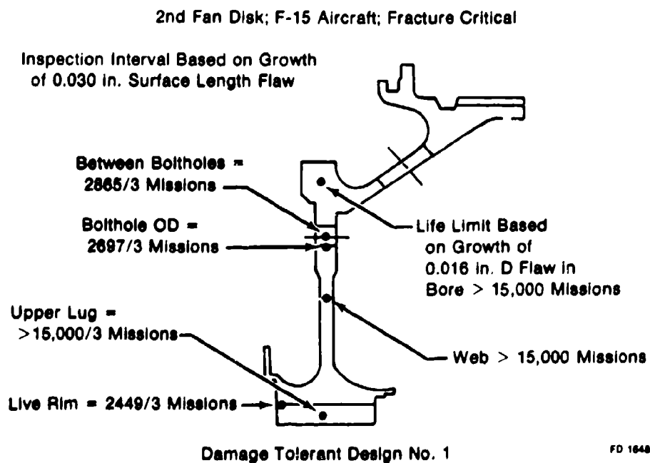
Figure 31. Disk Life Limits.
