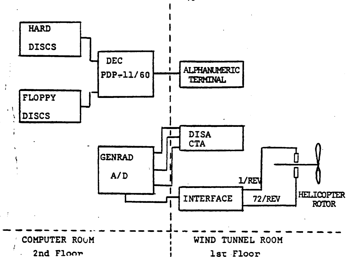
Figure 1. DATA ACQUISITION SYSTEM.
