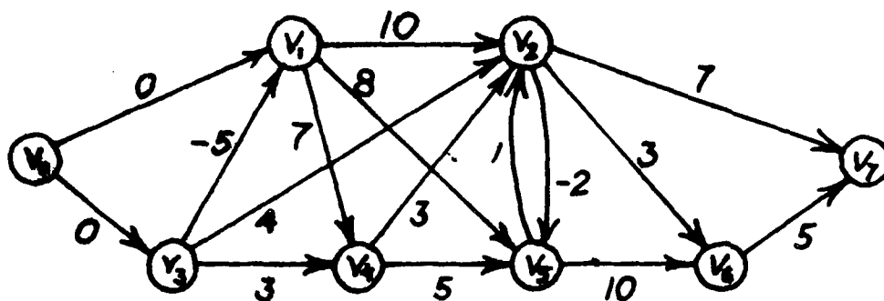
(b) The placement graph for separation 3.
