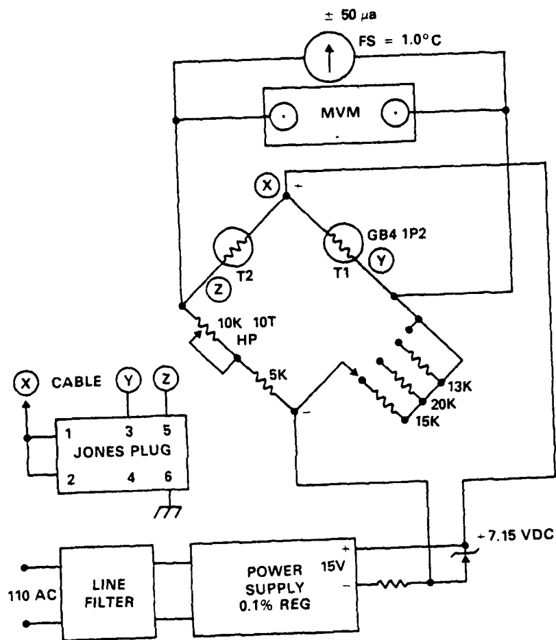
Fig. 3 — Schematic of the \Delta T system
