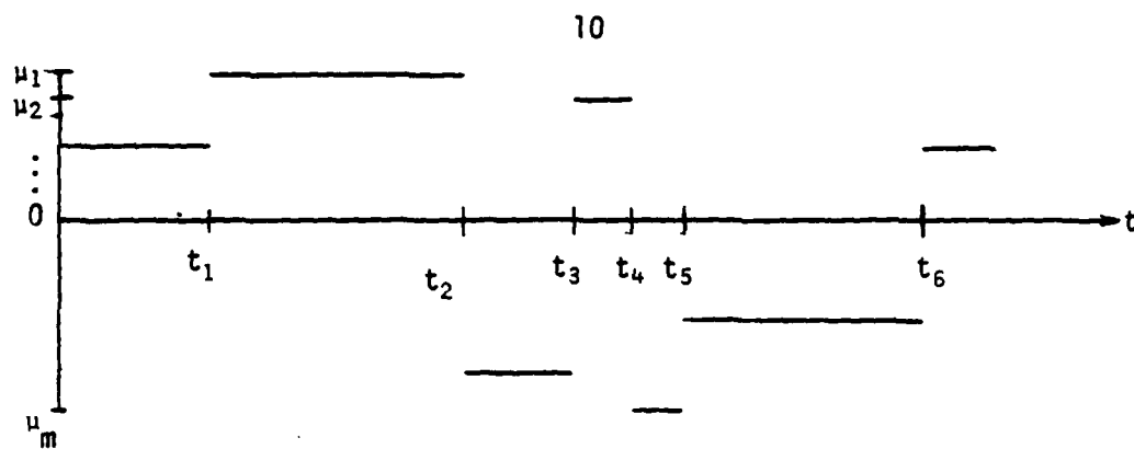
a. Sample paths of X_t process.
