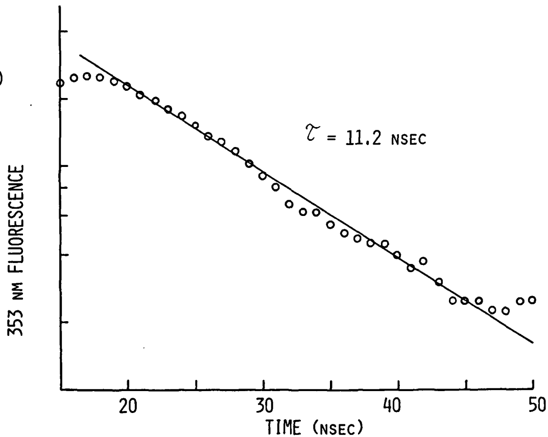
Figure 1. The 353 nm Fluorescence from a Gas Mixture of He+10 Torr Xe + 0.7 torr UF 6 at a Total Pressure of 125 torr. a) Oscilloscope traces showing the 351 nm exciting laser pulse and the 353 nm fluorescence signal. b) Semi-logarithmic plot of the 353 nm fluorescence decay.
