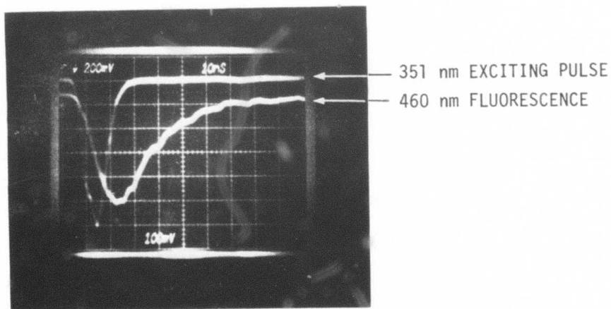
(b) 460 nm, 10 nsec/DIV
