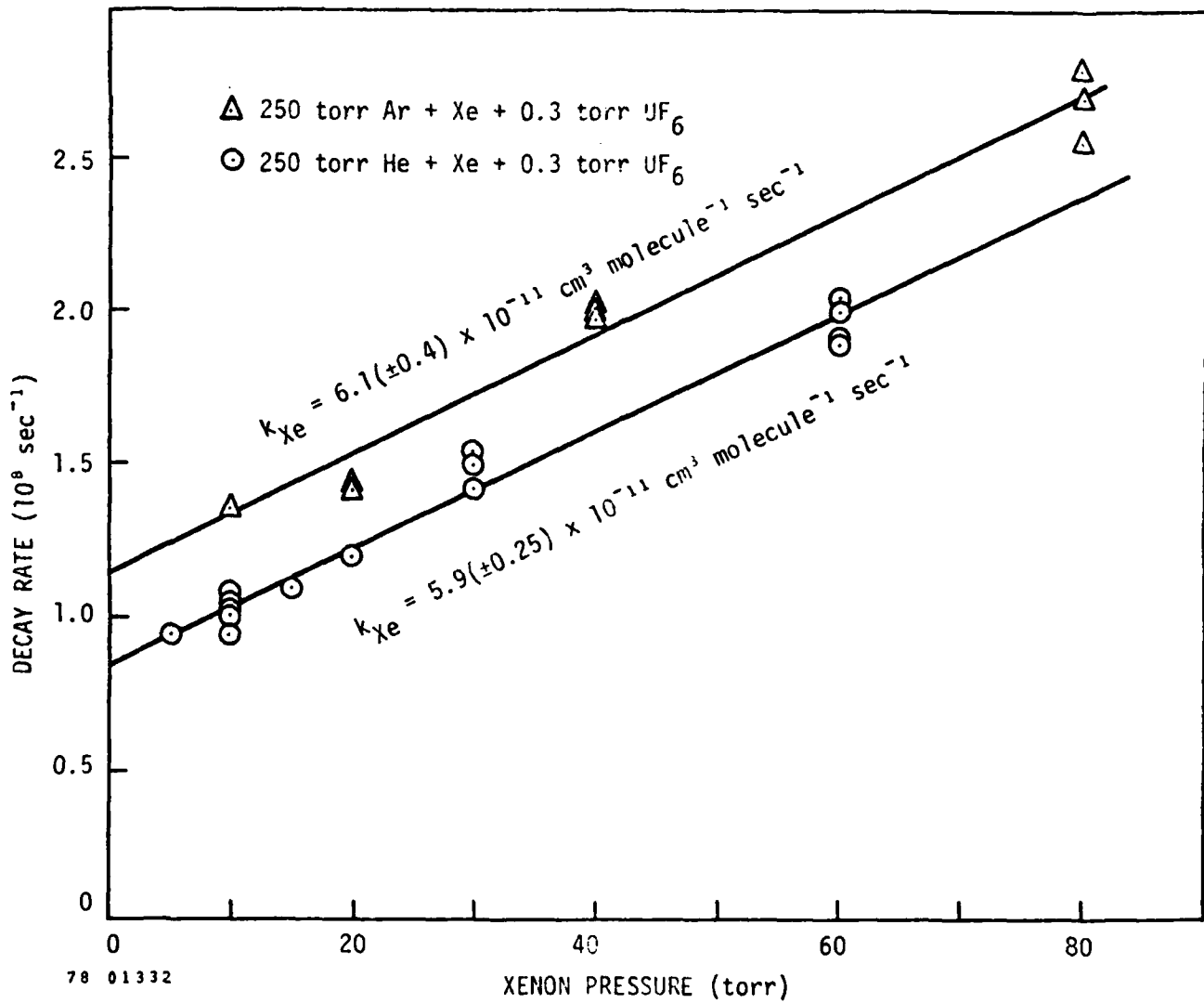
Figure 5. Variation of the 353-nm Fluorescence Decay Rate as a Function of Xe Partial Pressure. One set of experiments utilized Ar as the diluent while the other utilized He. The rate constants determined from the least squares fit to the data are indicated in the figure.
