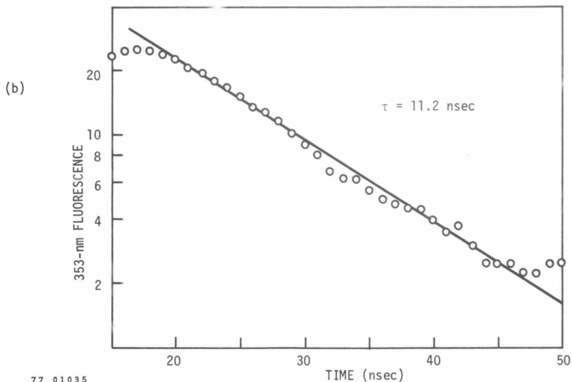
Figure 2. The 353-nm Fluorescence from a Gas Mixture of He + 10 torr Xe + 0.7 torr \text{UF}_6 at a Total Pressure of 125 torr (a) Oscilloscope Traces Showing the 351-nm Exciting Laser Pulse and the 353-nm Fluorescence Signal and (b) Semi-Logarithmic Plot of the 353-nm Fluorescence Decay
