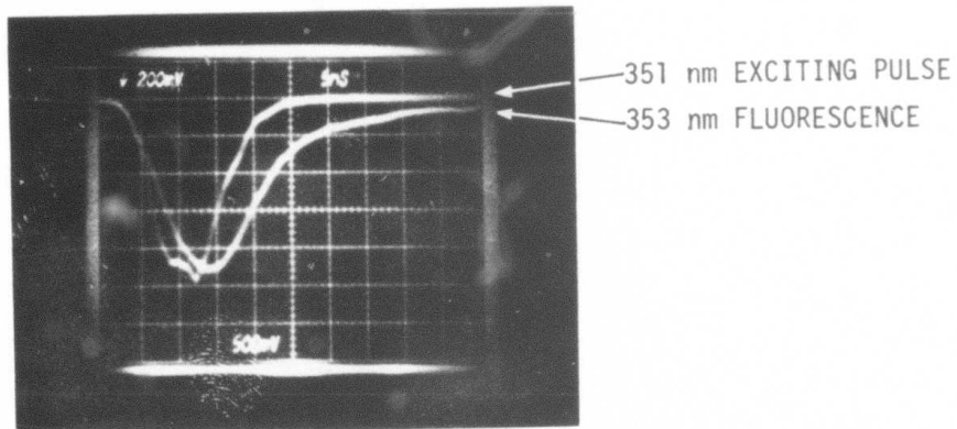
(a) 353 nm, 5 nsec/DIV
