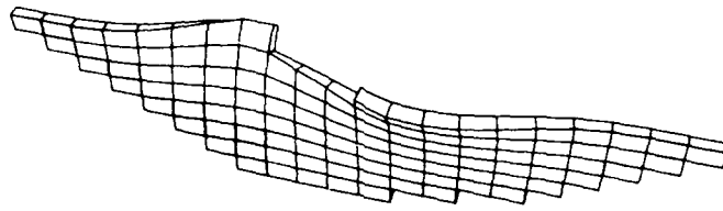
MODE 2, f = 264.7 Hz
