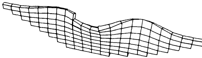
MODE 3, f = 310.5 Hz
