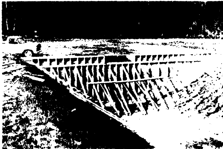
b. Upstream view of model dam formwork
