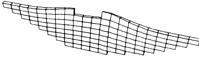
MODE 1, f = 233.3 Hz
