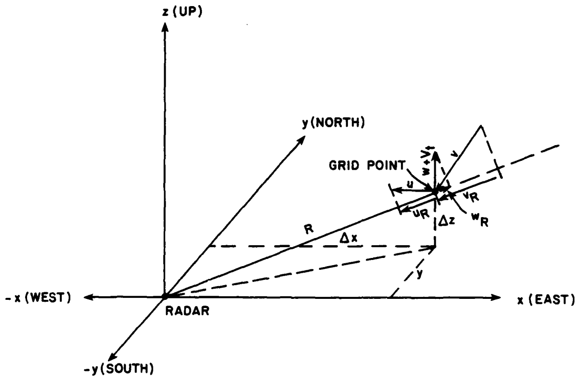
Figure 10. Illustration of conversion back to single-Doppler winds, with u , v , w , and V_t the obtained values from the dual-Doppler analysis. u_R , v_R , and w_R are the radial components of the u , v , and (w + V_t) respectively. R is the distance from the radar to the grid point.
