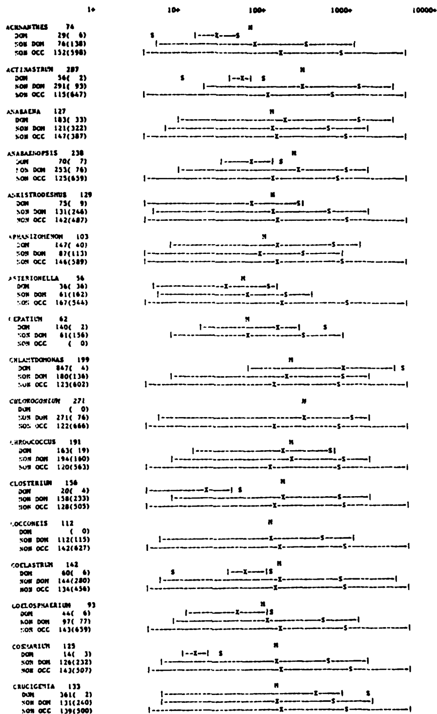
FIGURE A-1. Occurrence of 57 phytoplankton genera as related to total phosphorus levels.
