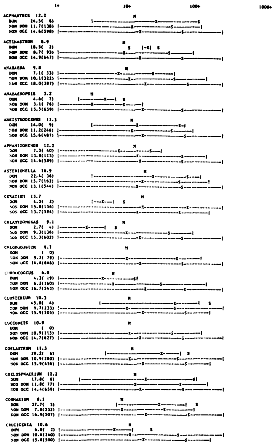
Figure A-3. Occurrence of 57 phytoplankton genera as related to N/P ratio values.
