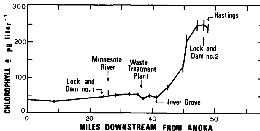
FIGURE 8. Mean concentrations of chlorophyll a during August and September 1976 in the Mississippi River near Minneapolis and St. Paul, Minnesota. The vertical line through each point indicates the 95% confidence interval for the mean (from data obtained by the Minneapolis-St. Paul Metropolitan Waste Control Commission).
