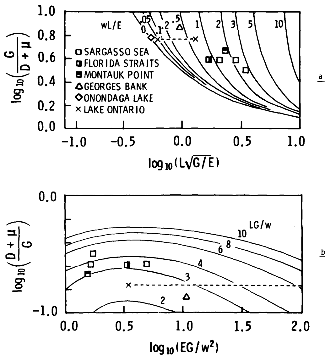
FIGURE 5. Application to lakes and oceans (a) the range of biologically and physically relevant dimensionless numbers. (b) normalized population growth rate versus normalized dispersion coefficient - a possible adaptation to the vertical dispersion in the oceans (Di Toro 1974).
