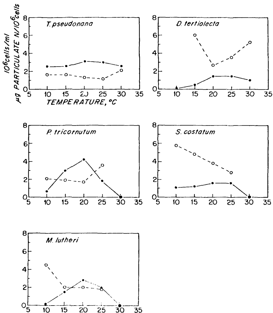
FIGURE 6. Effect of temperature on steady-state cell numbers (solid lines) and nitrogen cell quota (dashed lines) for five marine phytoplankton species grown in continuous culture at a dilution rate of 0.6/day. From Goldman (1977b). Redrawn from Goldman (1977b).
