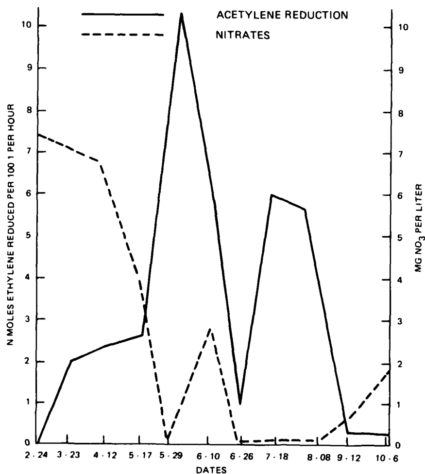
Figure 1. Comparison between nitrogen fixation and nitrate concentration.
