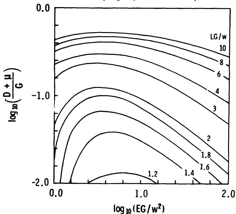
FIGURE 4. Normalized population net growth rate versus normalized vertical dispersion coefficient for various normalized euphotic zone depths. The plot illustrates the effects of these parameter variations if it is assumed that growth rate and settling velocity are constant (Di Toro 1974).
