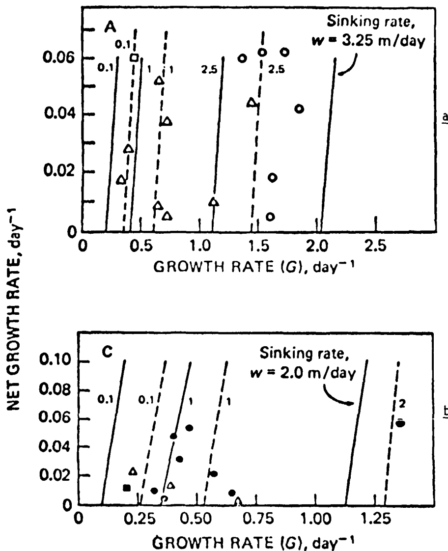
FIGURE 6. (a) Observed net growth rate versus average gross growth rate for Lake LBJ, 1973-1974. Lines of algal sinking velocity consistent with the observed euphotic zone depth and vertical dispersion. Key: Greens (open circles), Diatoms (triangles), Blue-Greens (open square), Mixed (closed circle), Flagellate dominated (closed square). Solid lines assume D = 0.05 day -1 ; dashed lines assume D = 0.25 day -1 . (b) Similar to (a) for Lake Erie, 1970 (Schnoor and Di Toro 1979). Redrawn from Schnoor and Di Toro (1979).
