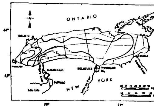
FIGURE 14. Lake Ontario three-dimensional sensitivity calculation. The computed June 1972 average chlorophyll in the 0- to 4-m layer (a). The effect of reversing the direction of all flows in the calculation (b); the effect of reducing all flow to 10% of their magnitude (c). These contours are differences in the sensitivity and the calibration computations, in \mu\text{g Chl a/l} , for the top layer (0-4 m) average June 1972 (Thomann et al. 1978).
