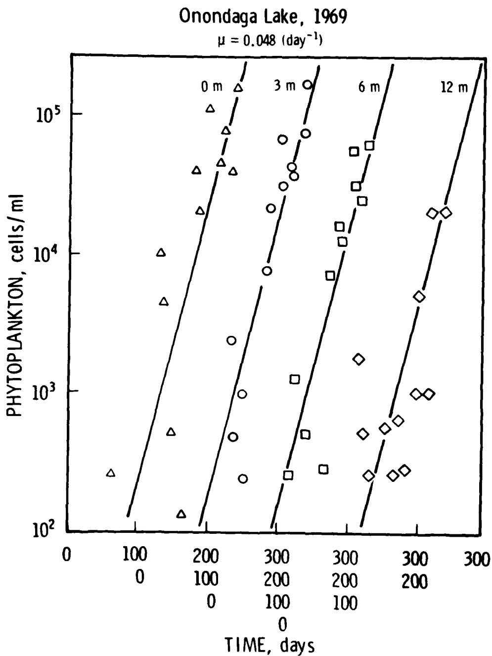
FIGURE 2. Onondaga Lake, two stations, 1969. Logarithm of phytoplankton total cell counts versus time at depths of 0, 3, 6, and 12 meters. The time scales for each depth are displaced to the right and labeled below each other for clarity, as indicated (Di Toro 1974).
