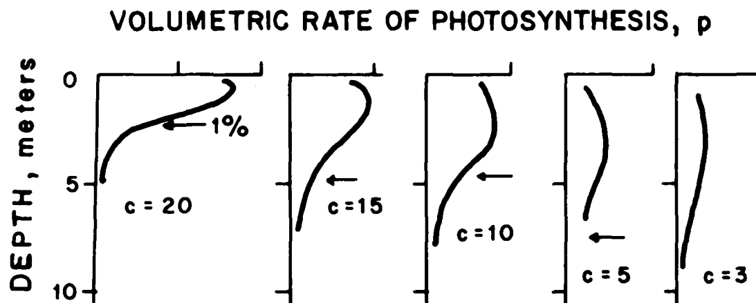
FIGURE 6. Relationships between rates of photosynthesis and depth at nearshore sites of Lake Victoria, central Africa, at concentrations, c , of chlorophyll a between 3 \text{ mg m}^{-3} and 20 \text{ mg m}^{-3} (from Talling 1965) Redrawn from Talling 1965.
