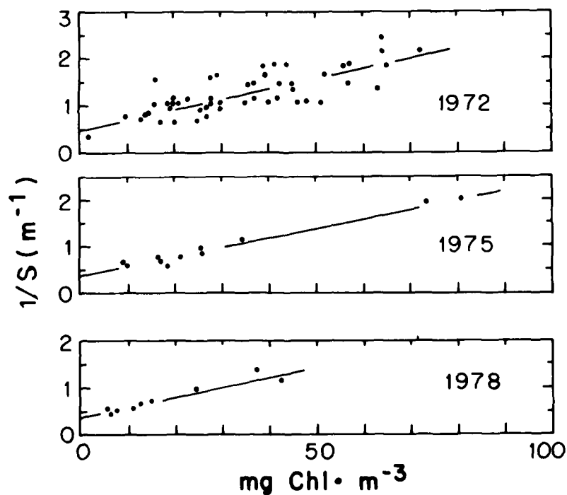
FIGURE 5. Linear regressions of reciprocal Secchi depth on concentrations of chlorophyll in Halsted Bay, Lake Minnetonka (from Megard, Settles, Boyer, and Combs 1979). Redrawn from Megard, Settles, Boyer, and Combs (1979).
