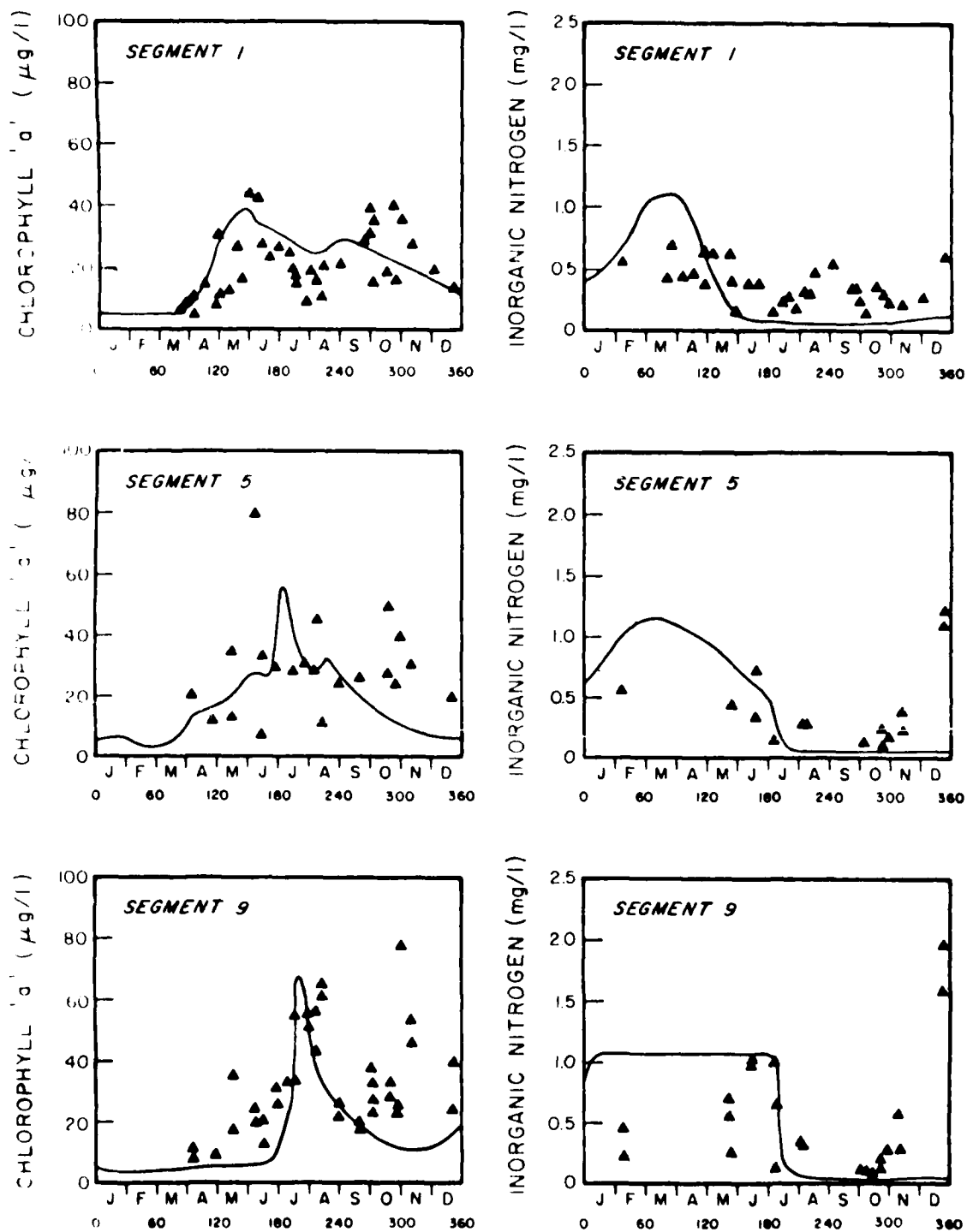
FIGURE 11. Observed and computed chlorophyll and inorganic nitrogen concentrations for Lake Livingston. Segment numbers refer to Figure 10 (Di Toro et al. 1976). Redrawn from Di Toro et al. (1976).
