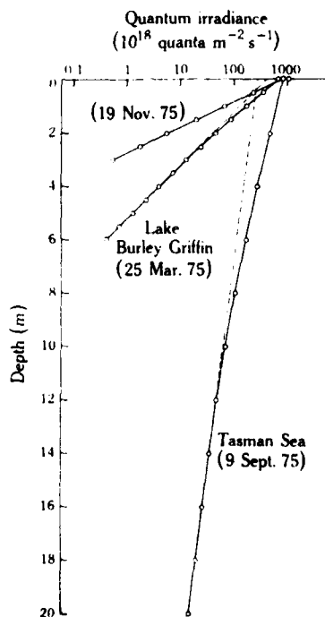
FIGURE 1. Relationship between log PAR and depth in Lake Burley Griffin (Australia) and the Tasman Sea (from Kirk 1977). Redrawn from Kirk 1977.
