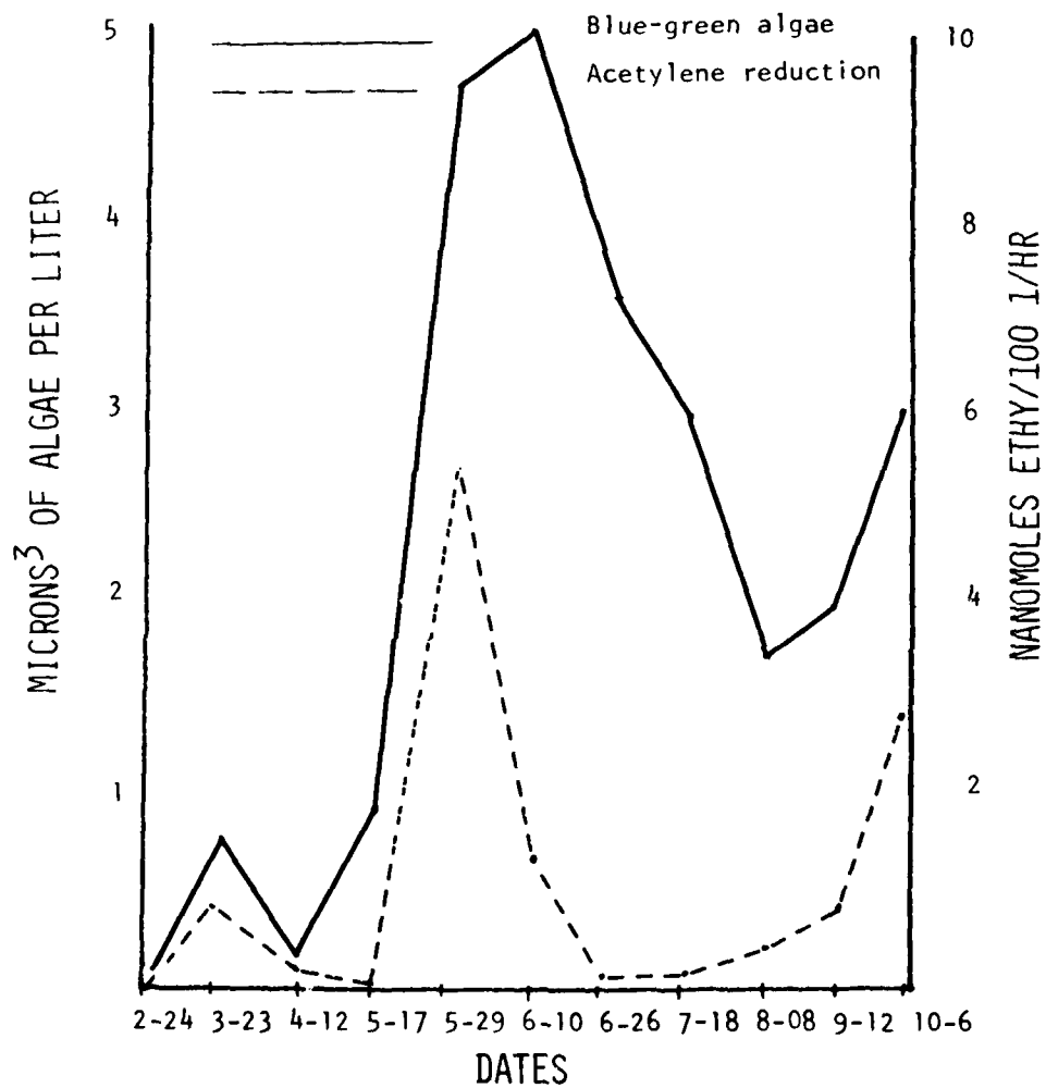
FIGURE 3. Comparison of blue-green algae volumes and acetylene reduction at the bottom of Station A.
