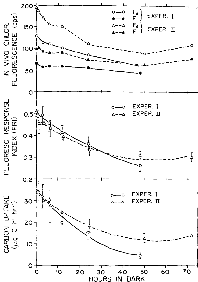
FIGURE 1. Decline of in vivo chlorophyll fluorescence ( F_i = unpoisoned sample fluorescence, F_d = DCMU-poisoned sample fluorescence), the fluorescence response index (FRI), and photosynthetic carbon uptake in Lake Texoma phytoplankton assemblages during light-deprivation experiments.
