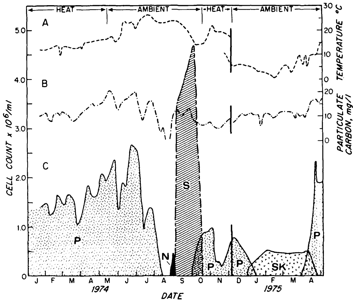
FIGURE 3. Summary of data collected in outdoor ponds at Environmental Systems Laboratory of Woods Hole Oceanographic Institution from January 1974 through April 1975. A - Pond temperature data; B - Particulate carbon data; C - Species data (P = Phaeodactylum tricornutum , N = Nitzschia closterium , S = Stichococcus sp., SK = Skeletonema costatum ). From Goldman and Ryther (1976). Redrawn from Goldman and Ryther (1976).
