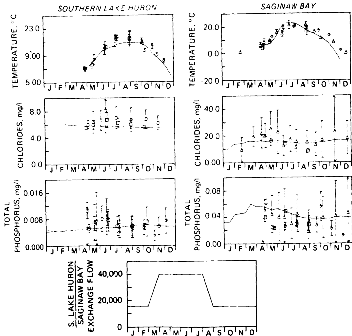
Figure 8. Calibration of Saginaw Bay - Southern Lake Huron exchange flow. Symbols are means \pm standard deviation of observed temperatures, chloride, and total phosphorus concentrations. Lines are the calculated results using the indicated exchanging flow (in ft 3 /sec) (Di Toro and Matystik 1979).
