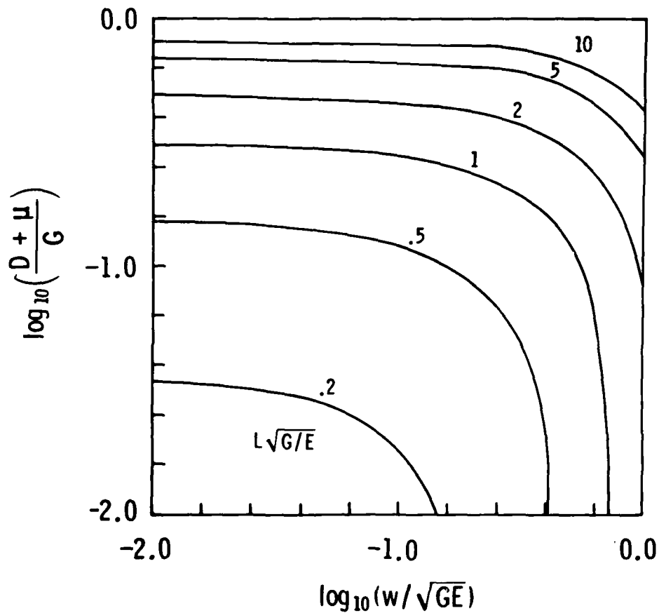
FIGURE 3. Normalized population net growth rate versus normalized algal settling velocity for various normalized euphotic zone depths. The plot illustrates the effects of these parameter variations if it is assumed that growth rate and dispersion coefficients are constant (Di Toro 1974).
