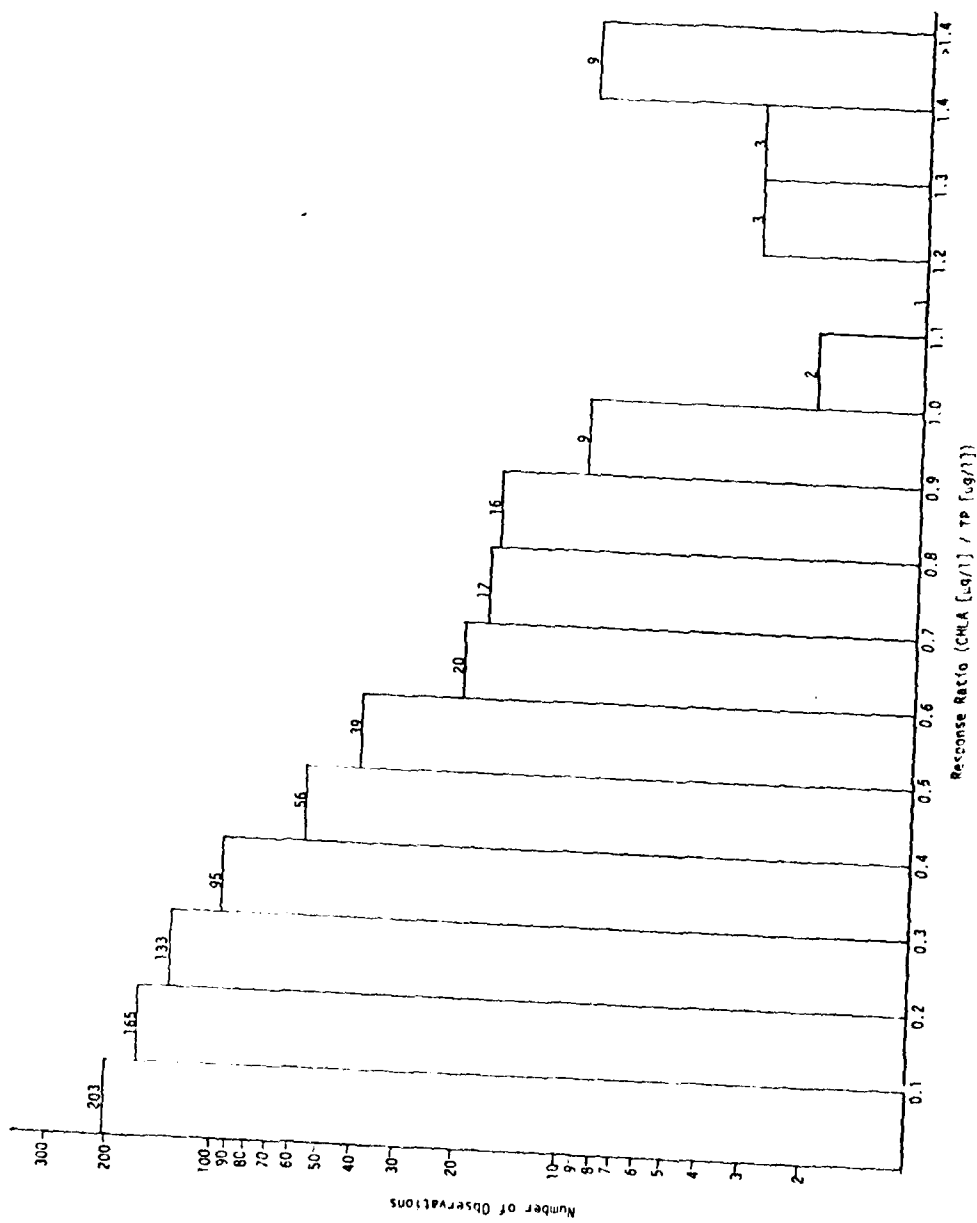
FIGURE 1. Response ratio in 757 United States lakes and reservoirs.
