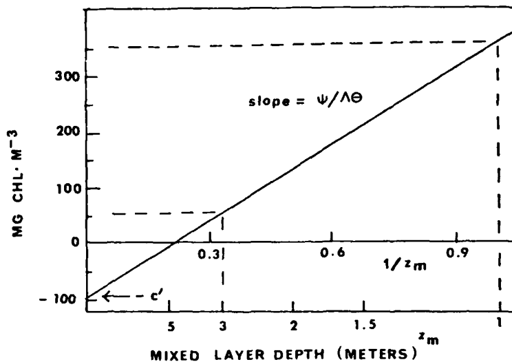
FIGURE 9. Steady-state concentrations of chlorophyll a in the Mississippi River as a function of the thickness of the mixed layer z_m . A decrease of z_m from 3 m to 1 m would increase concentrations of chlorophyll from 50 \text{ mg m}^{-3} to 350 \text{ mg m}^{-3} .
