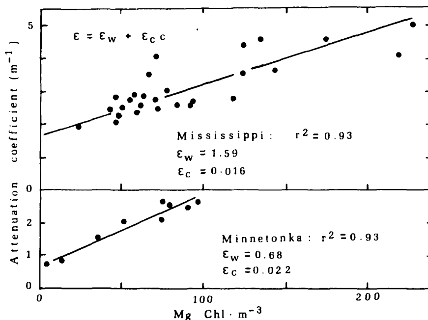
FIGURE 3. Regression of the vertical attenuation coefficient for PAR on concentrations of chlorophyll a in Lake Minnetonka and in the section of the Mississippi River that flows through Minneapolis and St. Paul, Minnesota.
