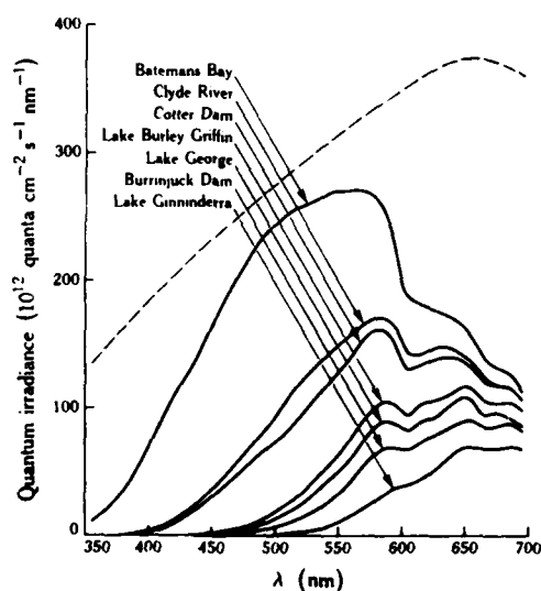
FIGURE 2. Effects of different concentrations of dissolved organic materials on the spectral composition of underwater PAR (from Kirk 1977). Redrawn from Kirk 1977.
