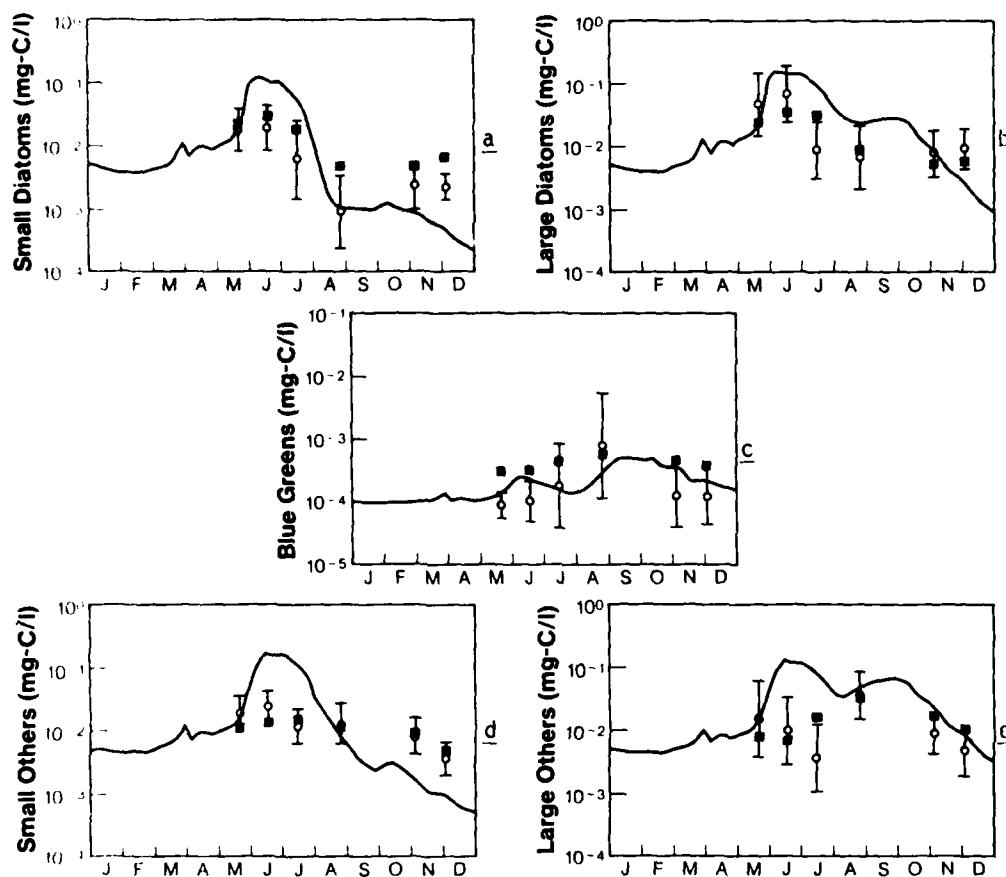
FIGURE 5. Seasonal dynamics of data and model output from epilimnion (0-20 m) of Lake Ontario during 1972; a - Small diatoms, b - Large diatoms, c - Blue-greens, d - Small others, e - Large others. \circ = lake-wide mean \pm 1 S.D. for surface samples and \blacksquare = lakewide mean for depth-integrated profiles (from Scavia 1979a). Redrawn from Scavia 1979a.
