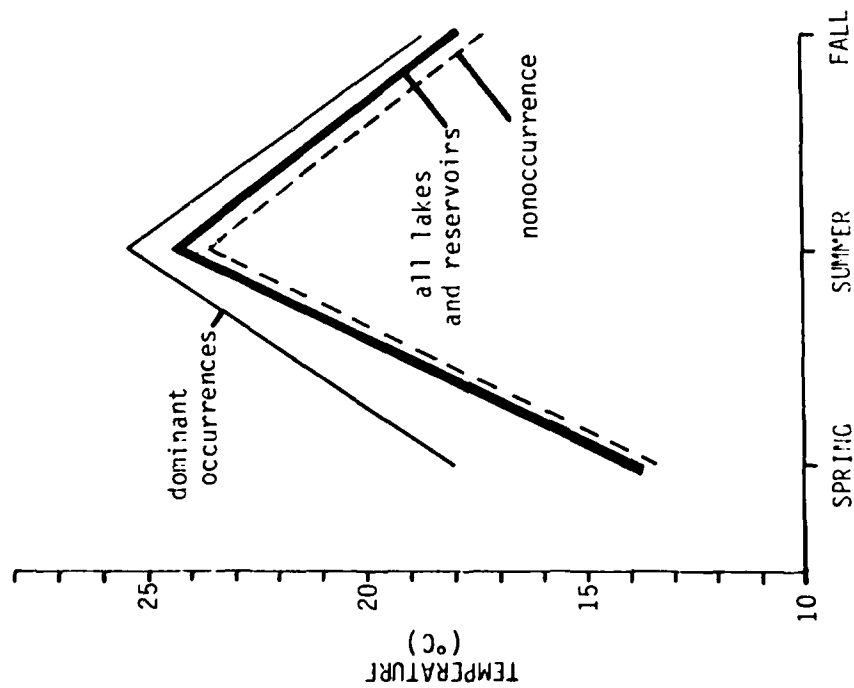
FIGURE 1. Mean seasonal temperature values associated with dominant occurrence and nonoccurrence of blue-green algae.
