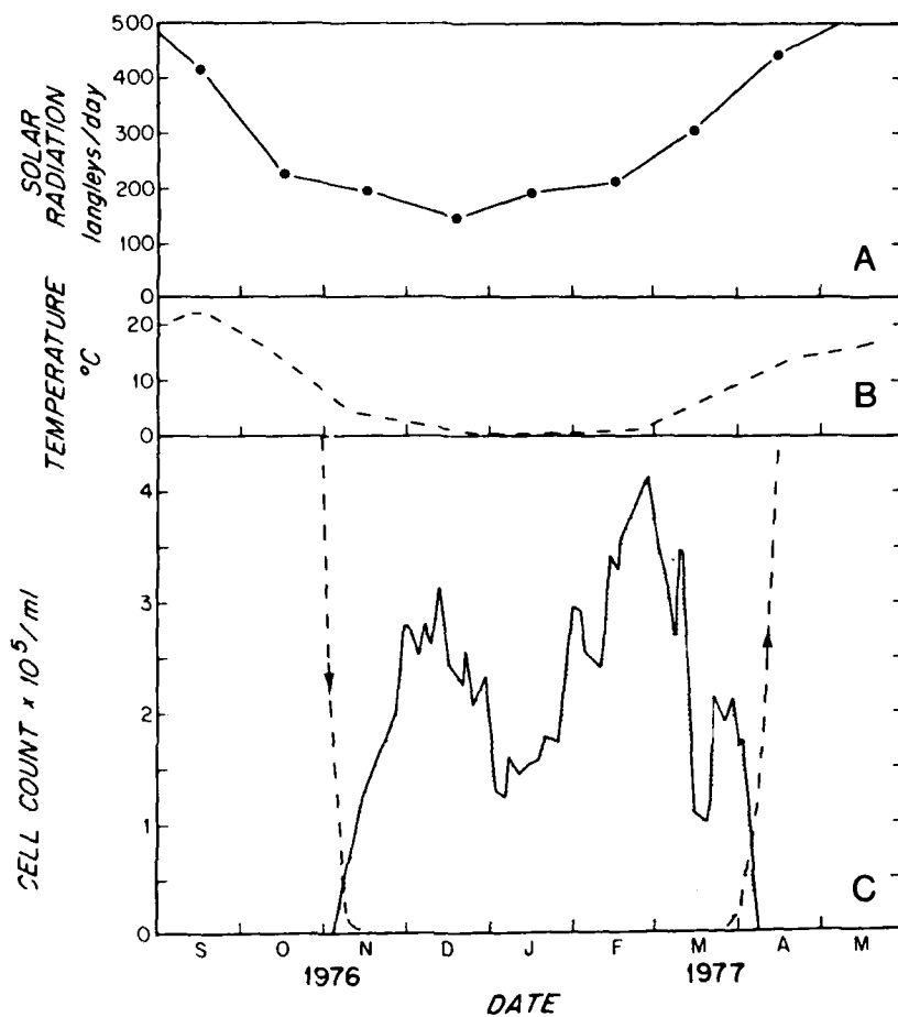
FIGURE 4. Summary of data collected in an outdoor pond at Environmental Systems Laboratory of Woods Hole Oceanographic Institution from September 1976 through May 1977. A - Solar radiation data; B - Pond temperature data; C - Species data (dashed lines = Phaeodactylum tricornutum ; shaded area = Skeletonema costatum ). Unpublished data.
