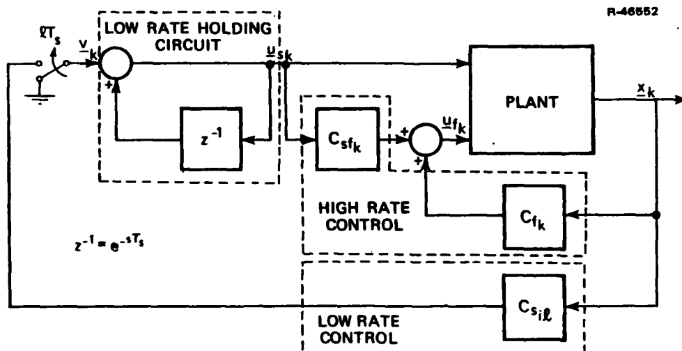
Figure 2.1-1 Multirate Regulator Structure
