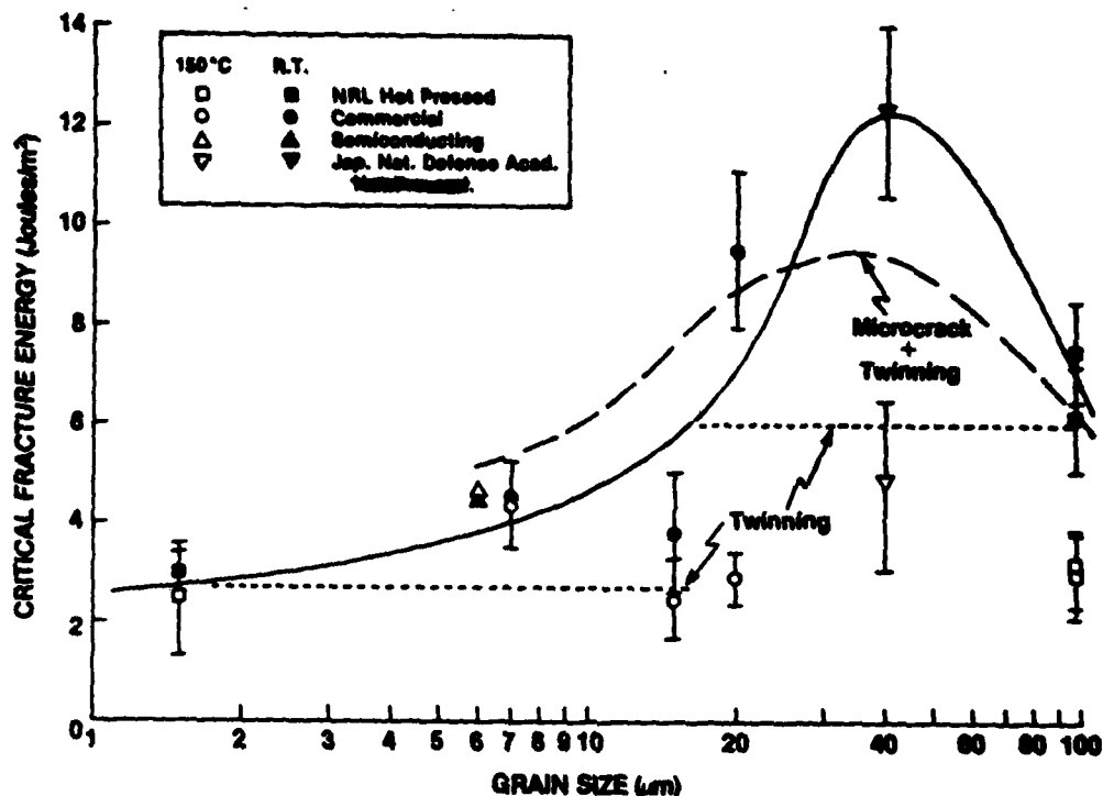
Figure 1. Fracture energy of \text{BaTiO}_3 as a function of grain size. — best fit to room temperature data; ... contribution due to twinning; - - - combined effect of twinning and microcracking predicted by Eq. 2.
