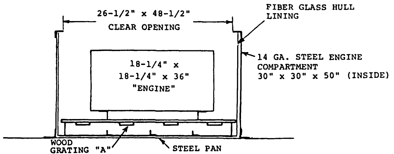
Figure 3-7. Fire Model 7 (Open-top and End Engine Compartment).
