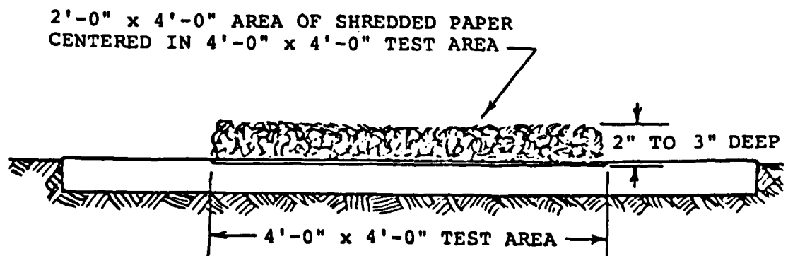
Figure 3-3. Fire Model 3 (Fuel Saturated Paper).
