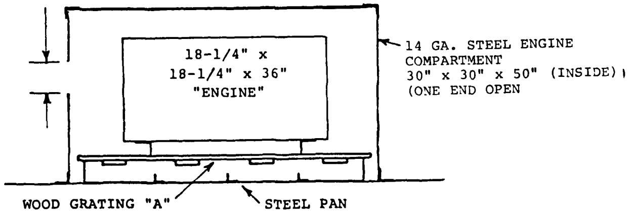
Figure 3-4. Fire Model 4 (Open Ended Engine Compartment).
