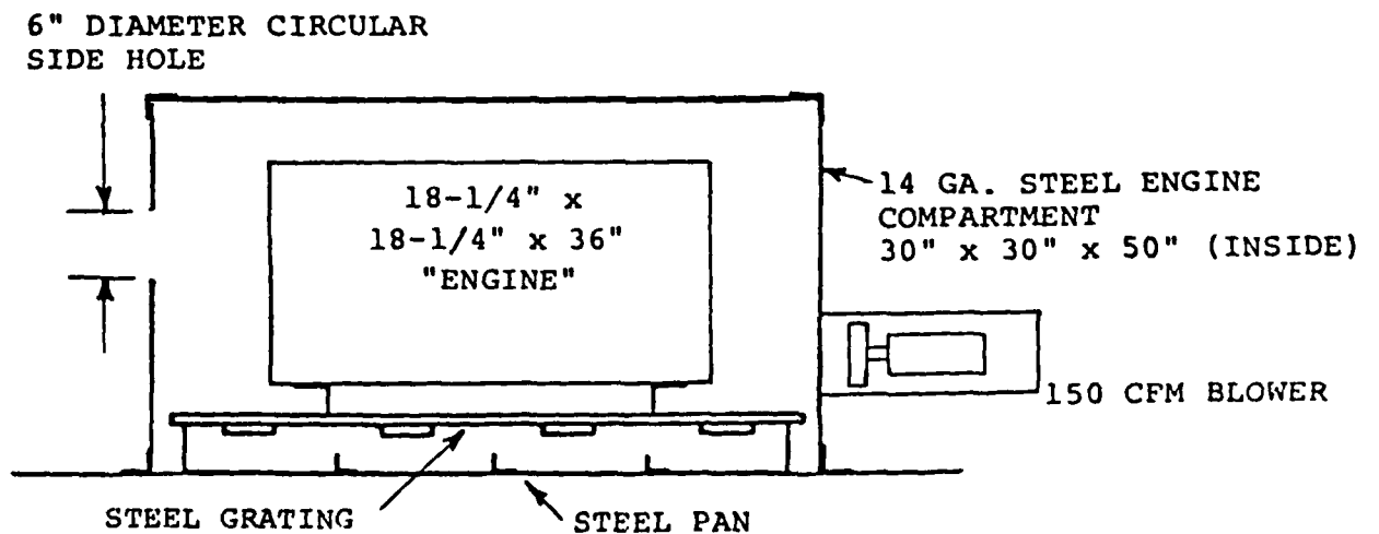
Figure 3-5. Fire Model 5 (Power Ventilated Engine Compartment).
