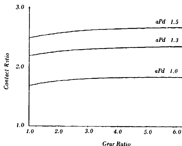
Figure 7 Contact Ratio vs. Gear Ratio
