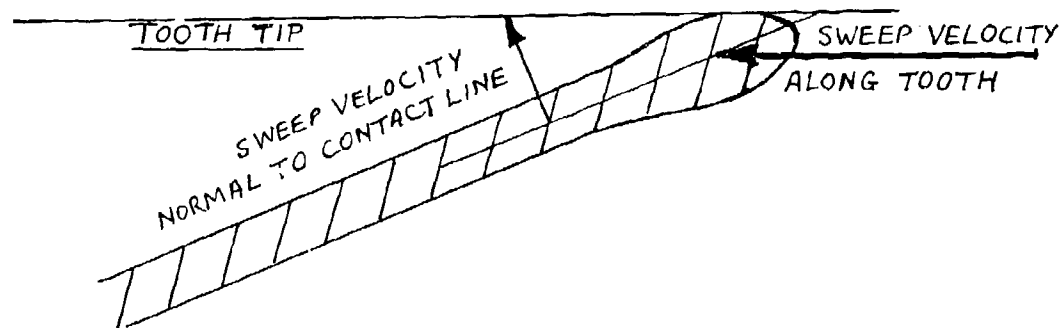
Fig.6 Conditions at the ends of the contact line relating to oil film generation
