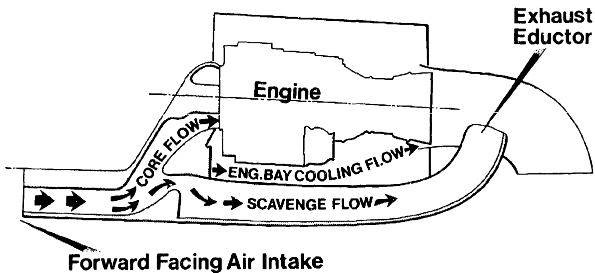
Fig. 14 An asymmetric separator proposal
