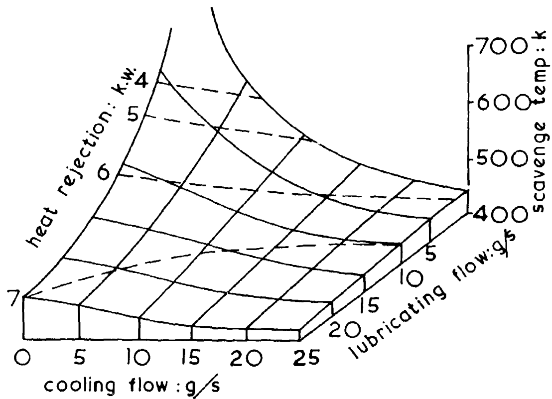
Fig.3 Heat rejection to the oil system as a function of cooling and lubricating flows for a typical externally cooled high speed turbine roller bearing chamber
