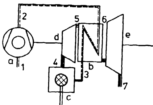
Fig. 13 Recuperator Upstream the Power Turbine
