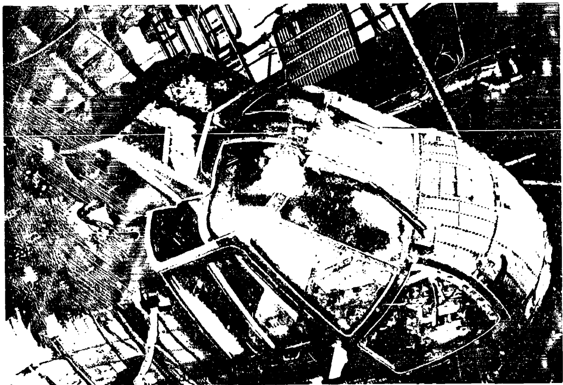
Fig.2 Sea King Forward ice accretion (NGII test)
