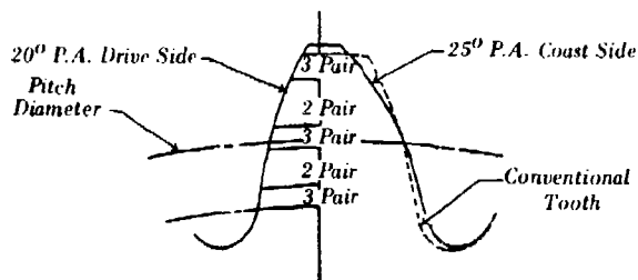
Figure 18 Buttress Tooth Form
