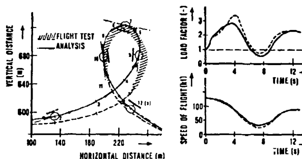
Fig. 9 - Potential acrobatic power.
