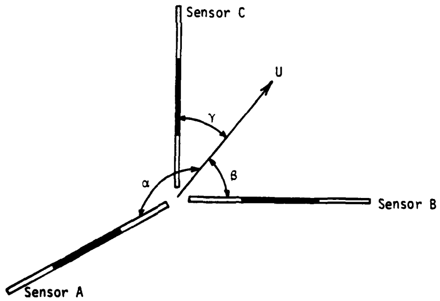
Figure 3-2. Geometry of 3-Dimensional Hot Film Probe Tip
