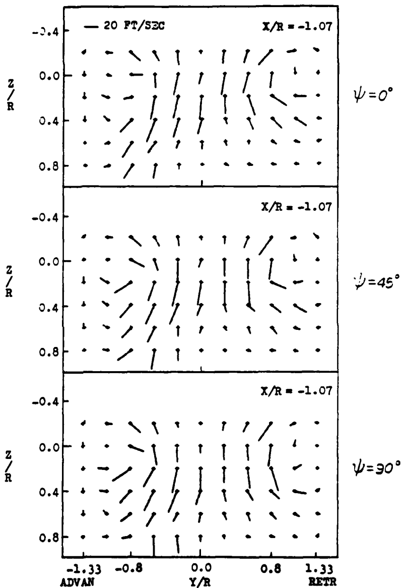
Figure 4-4. Y-Z Vectors for X/R = -1.07 at Several Blade Angles
