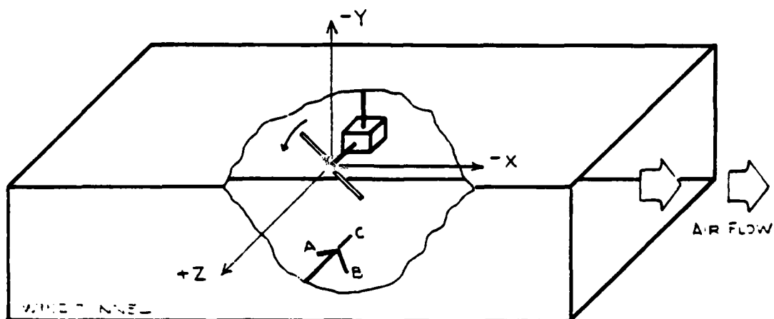
Figure 2-5. The Spatial Orientation of the Probe in the Wind Tunnel. However, due to rotor interference, 147 points cannot be measured as indicated by the shaded region in Figure 2-6. Note also that the rotor hub center is the point \langle 0,0,0 \rangle for a shaft tilt angle equal to zero.
