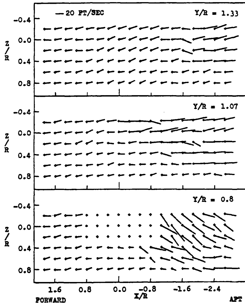
Figure 4-2. X-Z Vectors for \psi = 355^\circ
