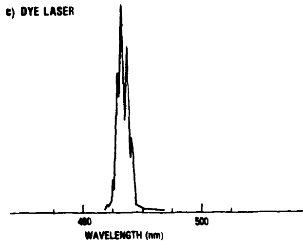
Figure 4-3. Spectra of the Stimulated Emission From a) the XeF C+A Oscillator, b) the C+A Multipass Amplifier, and c) the Injected Dye Laser. These spectra were obtained by densitometering plates taken with a 0.5 meter spectrometer and have been corrected for a factor of two decrease in film sensitivity from 430 to 500 nm.
