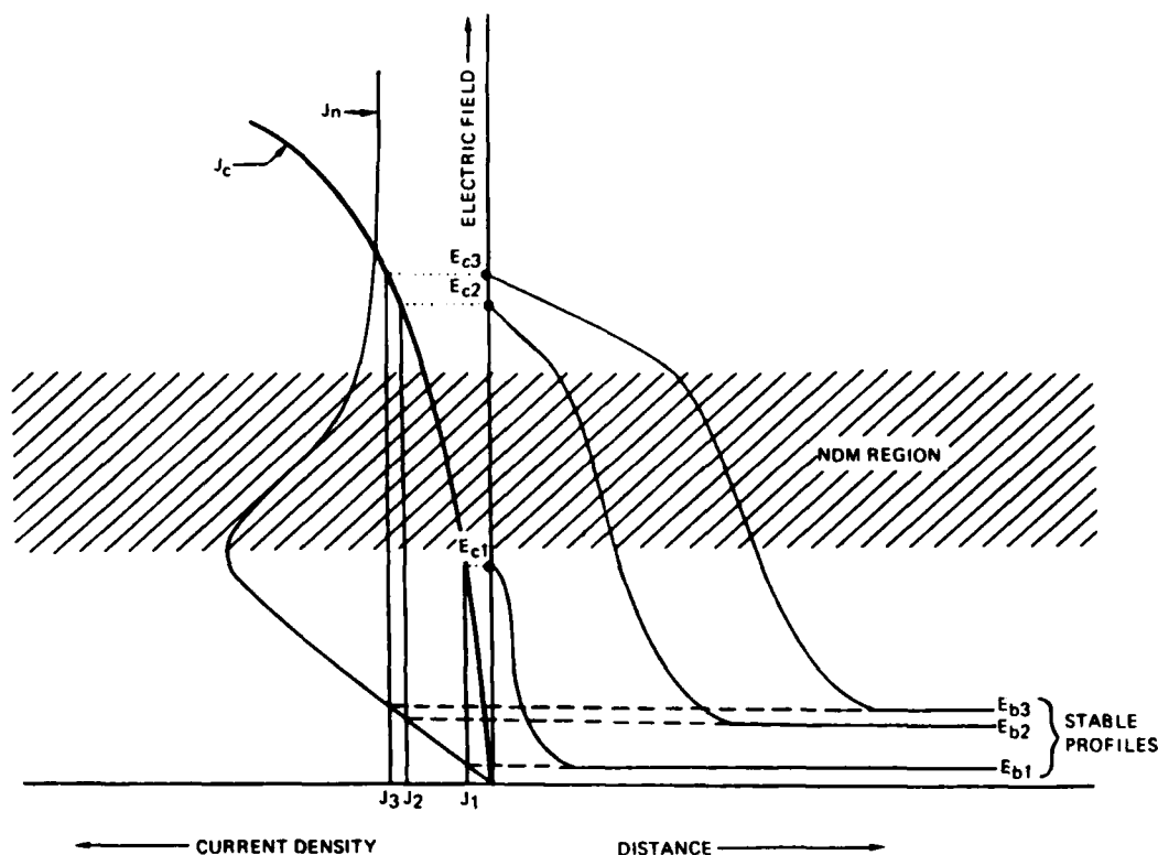
Fig. 5. As in Fig. 3, but j_c(E_c) and j_n(E_c) intersect within the region of saturated drift velocity.
