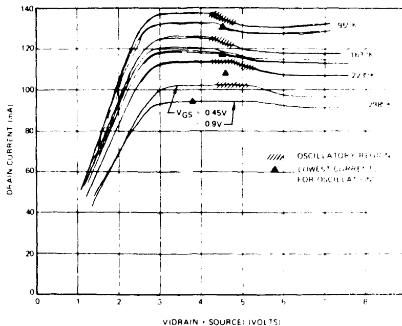
Fig. 9. Temperature dependent pulsed data for the device of Fig. 8. For these measurements a 50 \Omega load and a source from ground.
