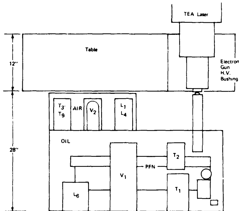
Figure 10. Electron Beam Modulator Layout
