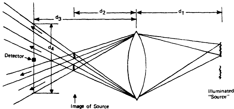
(b) Equivalent Optics
