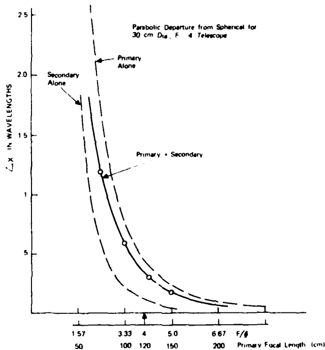
Figure 17. Spherical Telescope Figure Error
