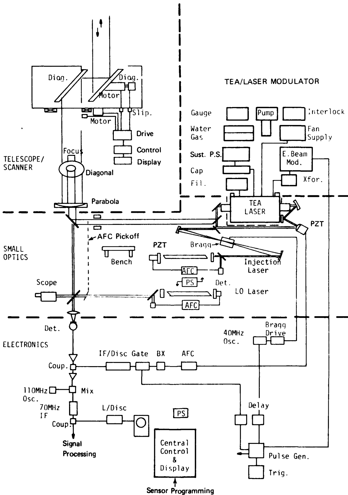
Figure 1. Demonstration System with Separate LO Laser
