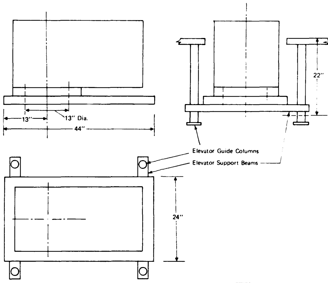
Figure 20. Scanner Elevator
