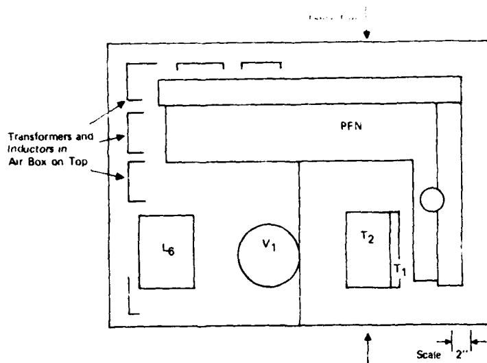
Figure 11. Electron Beam Modulator Layout: Top View
