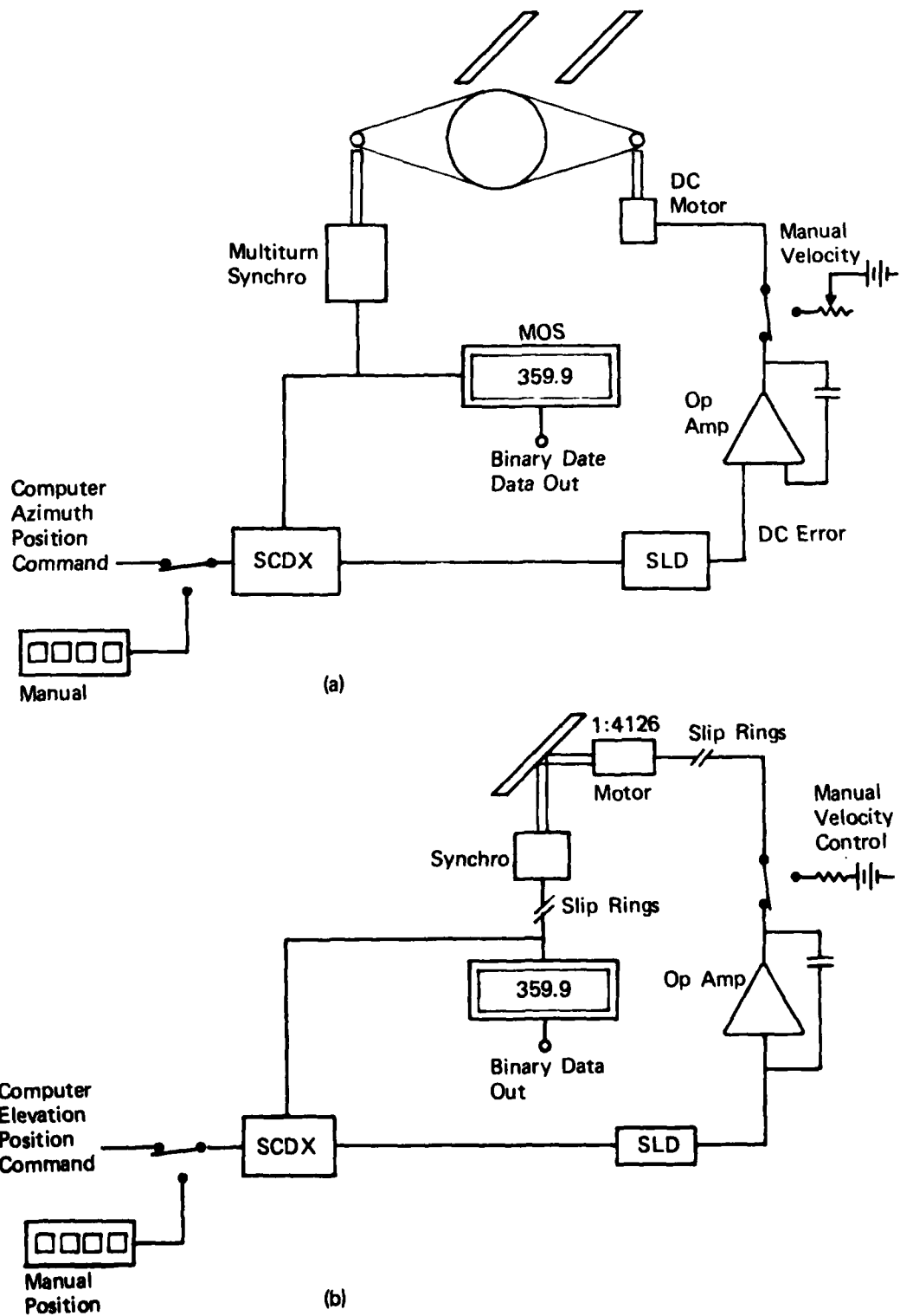
Figure 23. Digital Position Command Servo a) azimuth b) elevation
