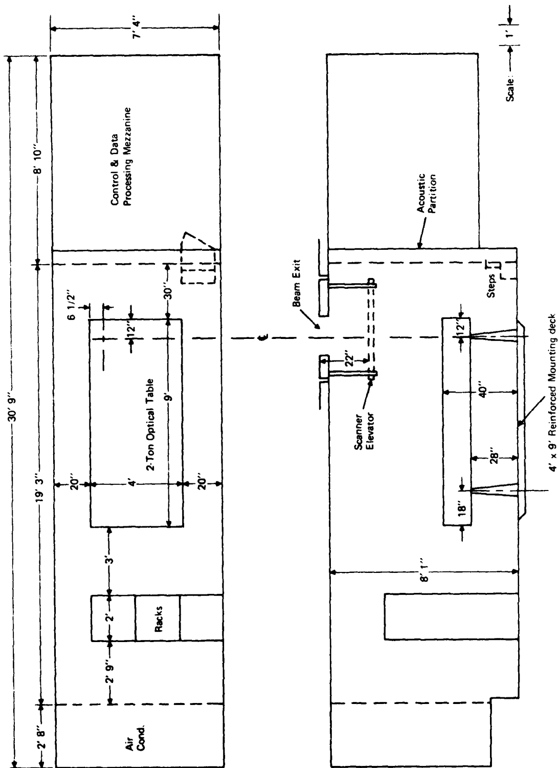
Figure 18. Inside Dimension Requirements
