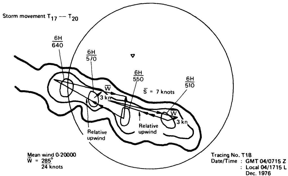
Fig. 11 Manual tracing of weather radar P.P.I. 4 Dec. 1976 at 1715 EST.
