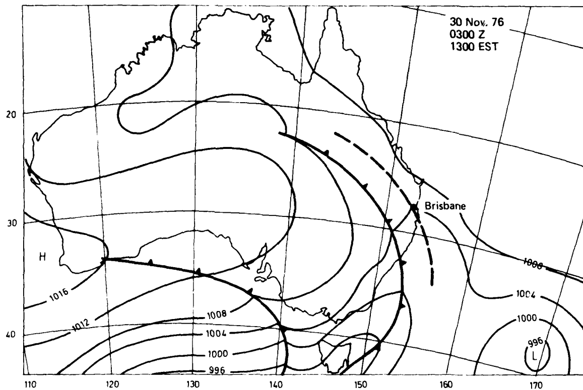
Fig. 18 Surface chart preceding storm on 30 Nov. 1976.
