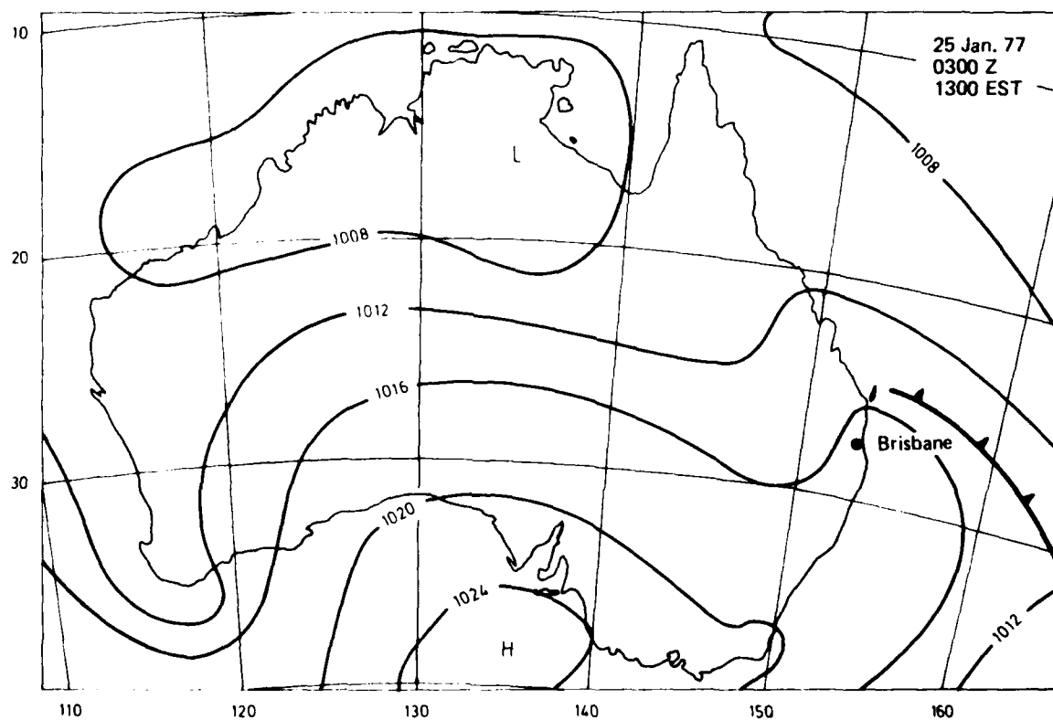
Fig. 45 Surface chart at time of type 5 incident on 25 Jan. 1977.
