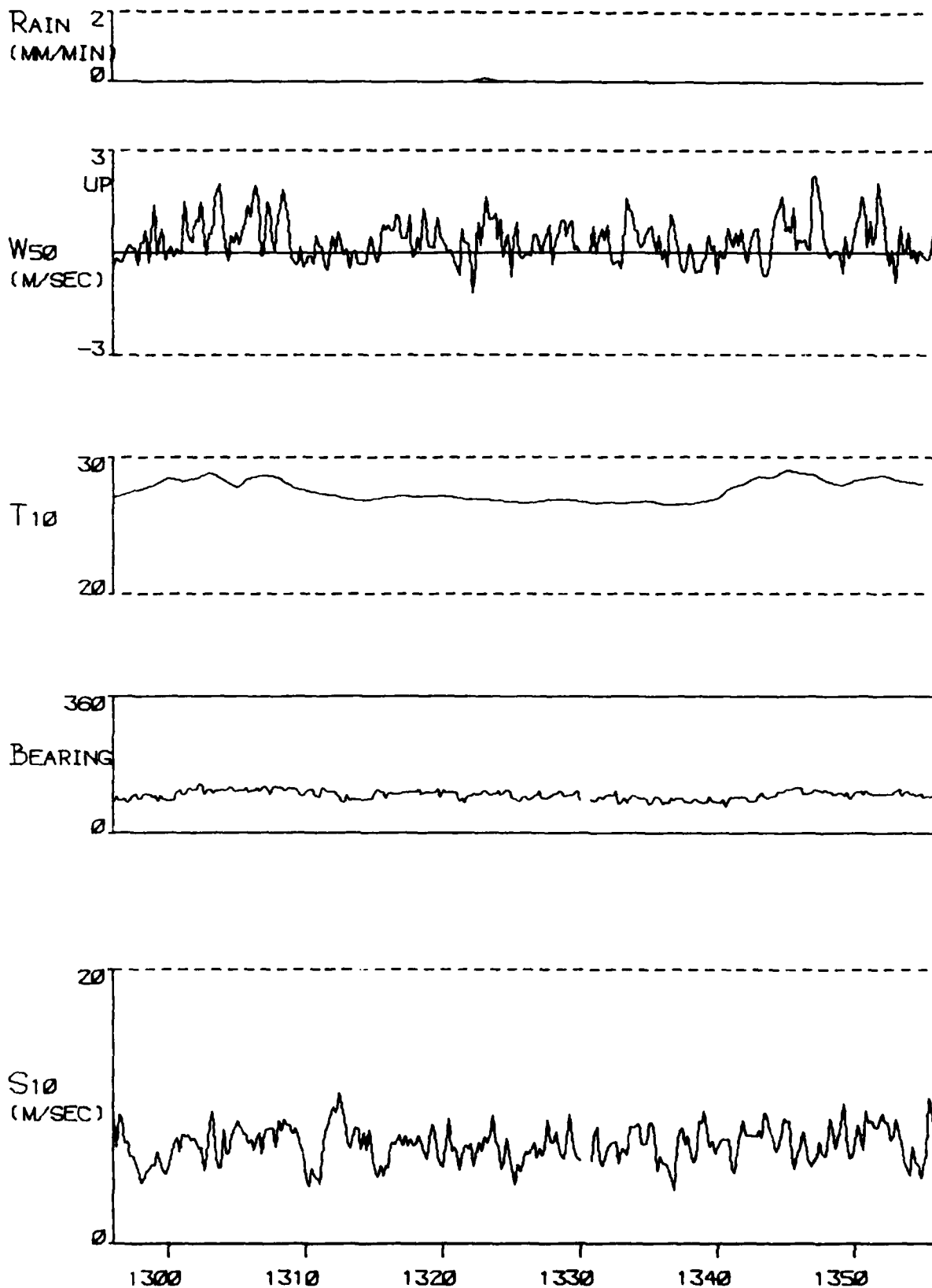
Fig. 49 A selection of parameters recorded during the type 5 incident on 12 Feb. 1977.
