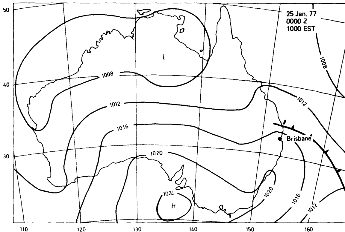
Fig. 44 Surface chart preceding type 5 incident on 25 Jan. 1977.
