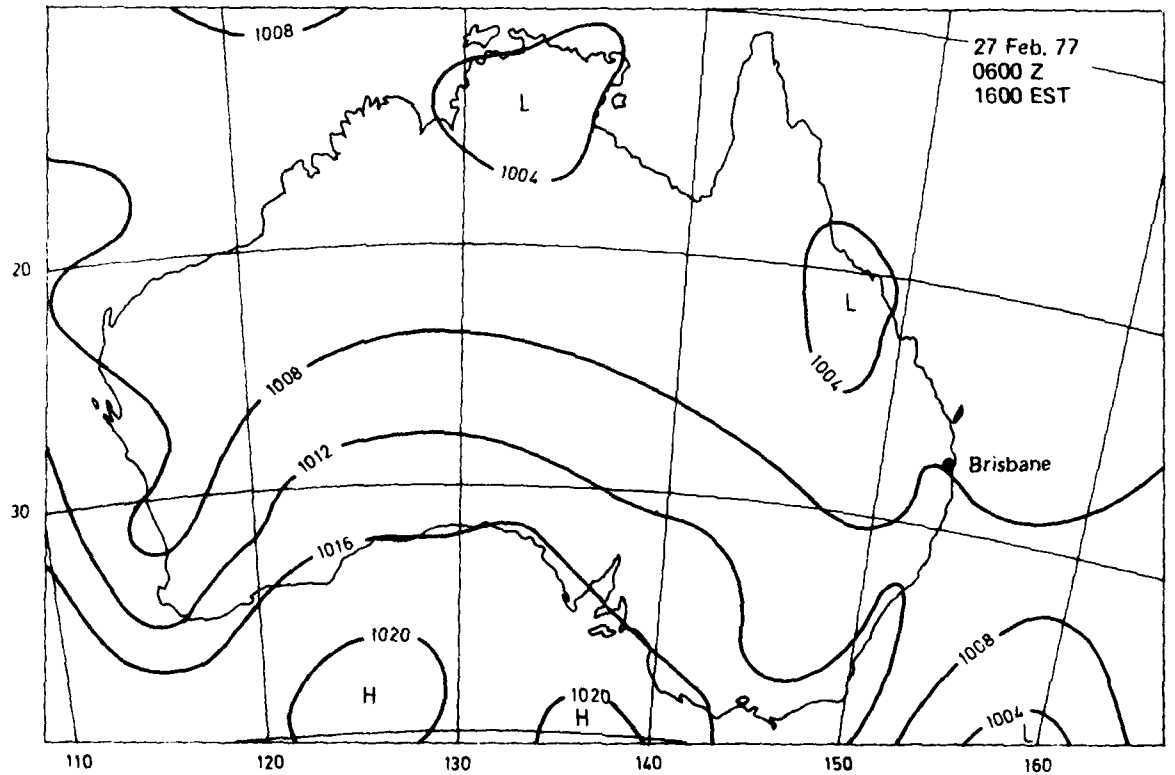
Fig. 34 Surface chart at time of type 4 incident on 27 Feb. 1977.
