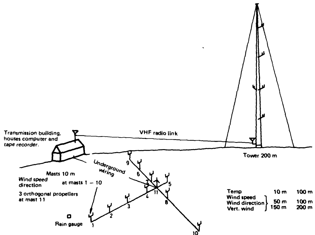
Fig. 1 General layout of meteorological instruments at Bald Hills.
