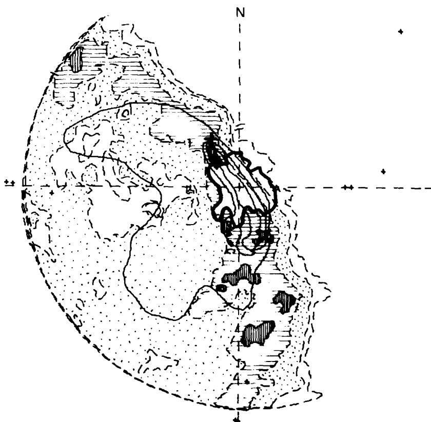
Fig. 14 Comparison of VIP photograph on 7 Nov. 1977 at 1845 EST with manual P.P.I. tracing at 1850 EST.
