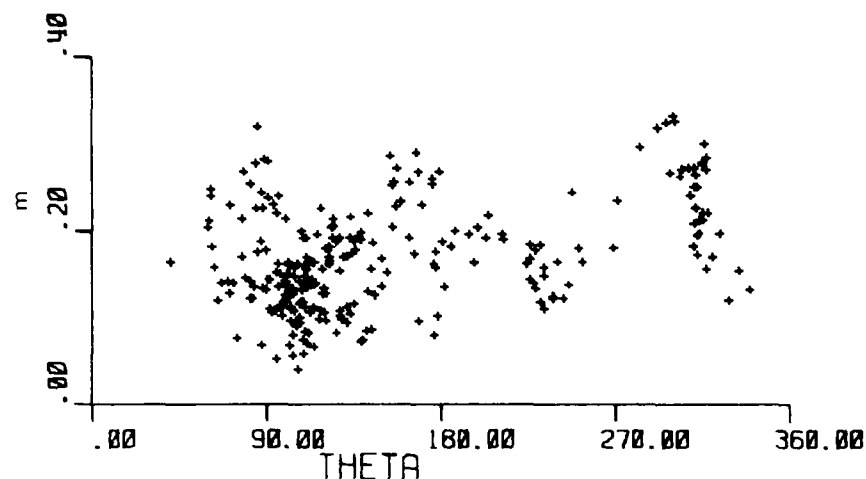
Fig. 56 Value of the wind speed profile exponent, m , for cases where the mean wind speed exceeds 5 m/s as a function of bearing from which wind approaches the Bald Hills site.
